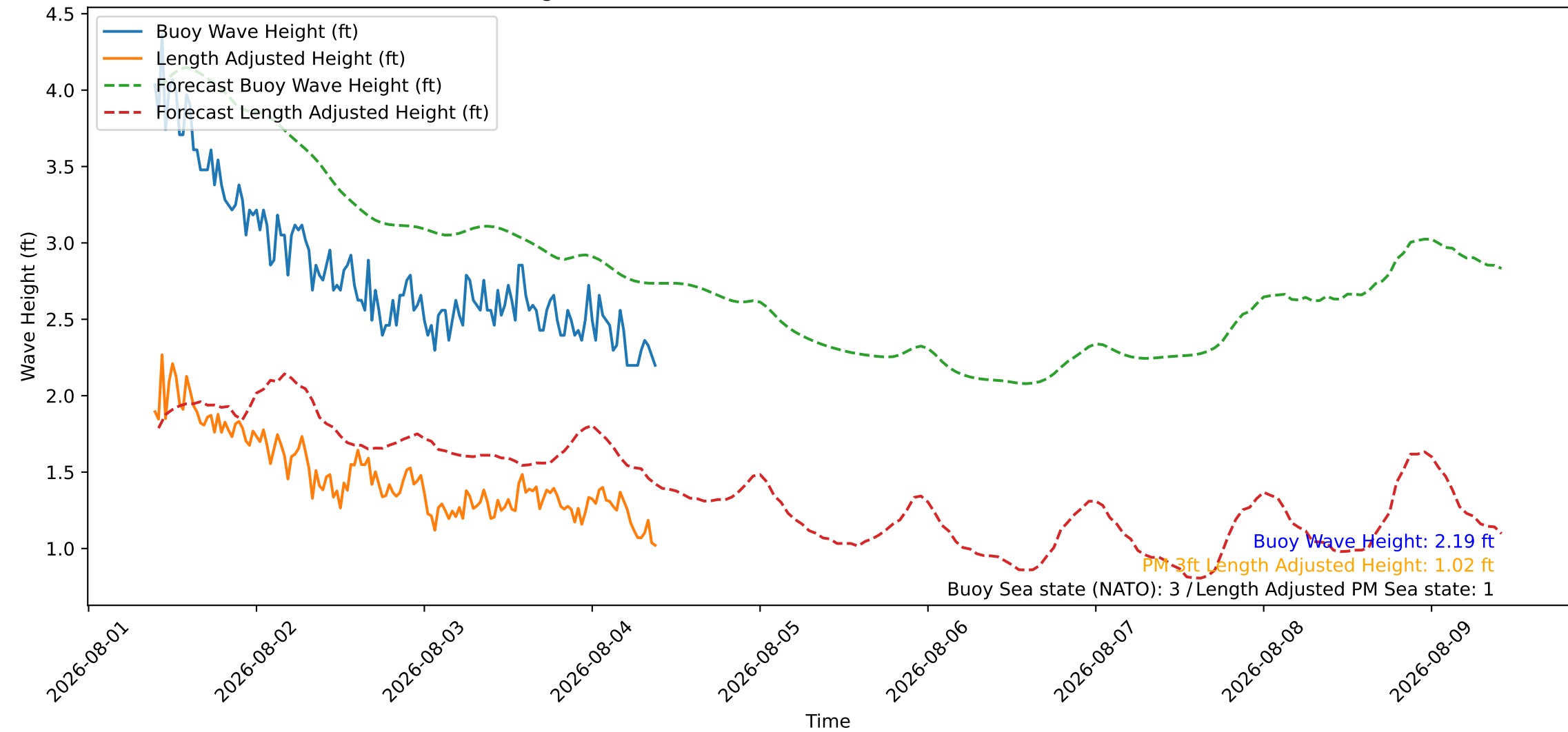
Wave Heights over Time for Oceanside Harbor at 2026-08-04 09:40:26
