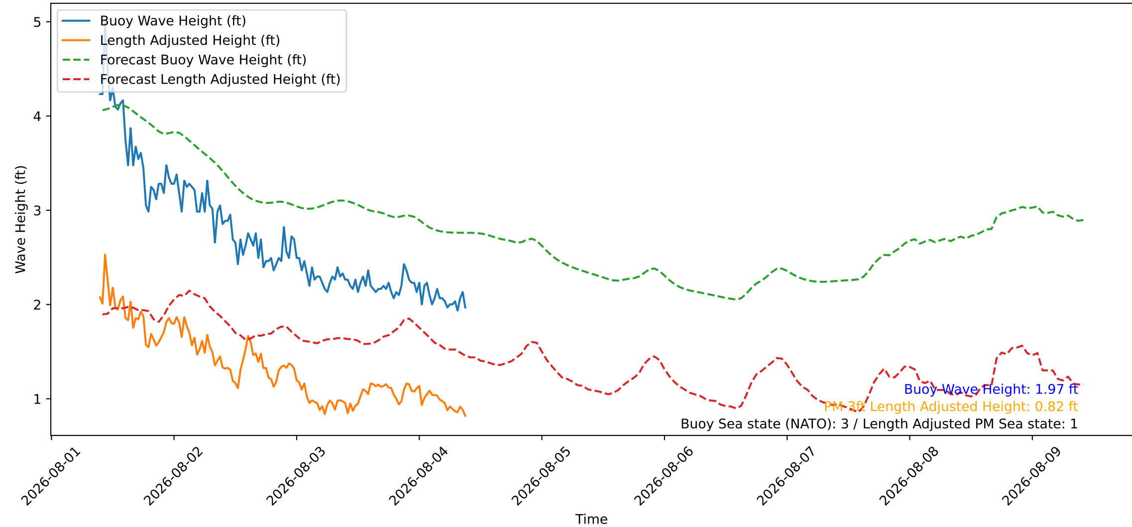
Wave Heights over Time for Green Beach at 2026-08-04 09:41:08
