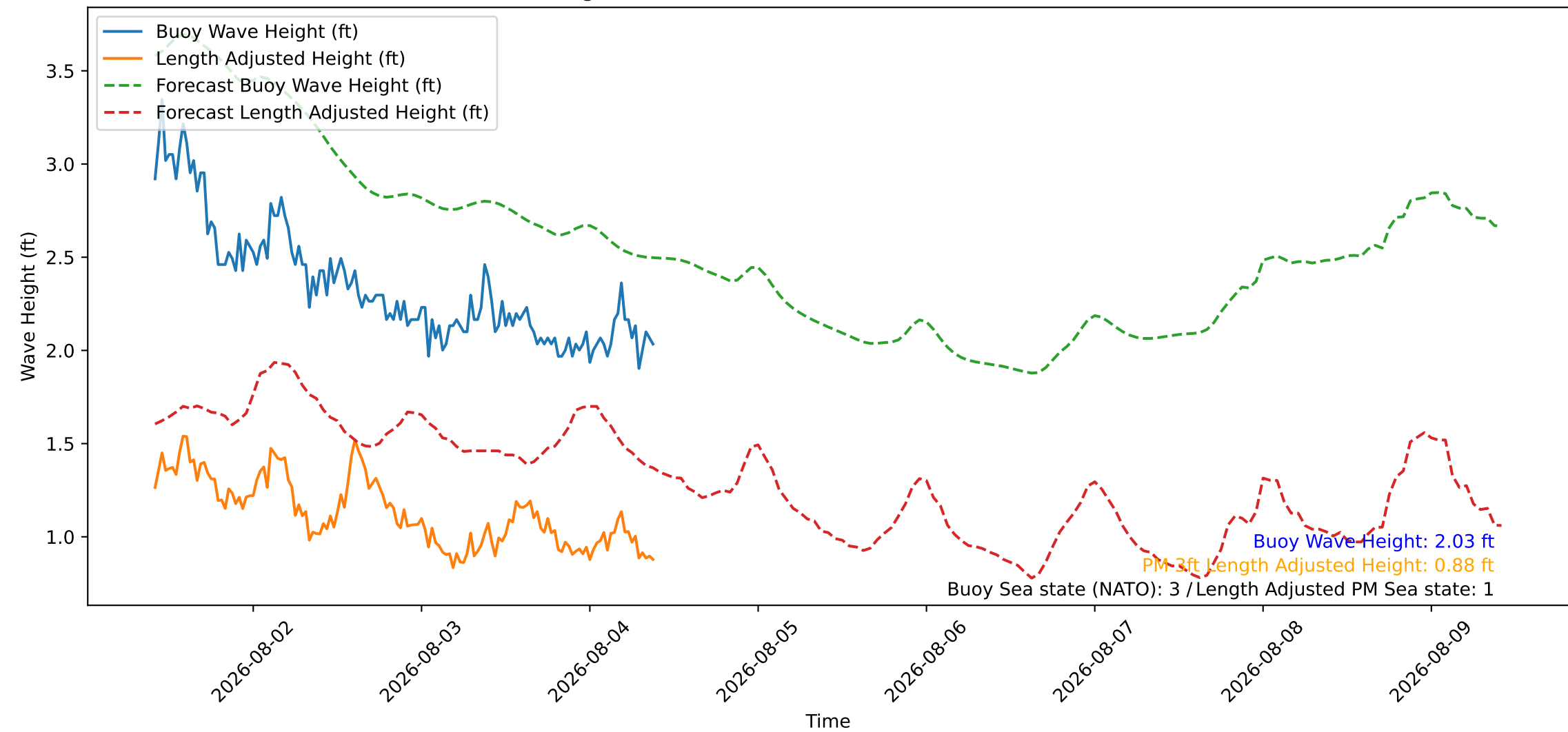
Wave Heights over Time for Red Beach at 2026-08-04 09:40:46
