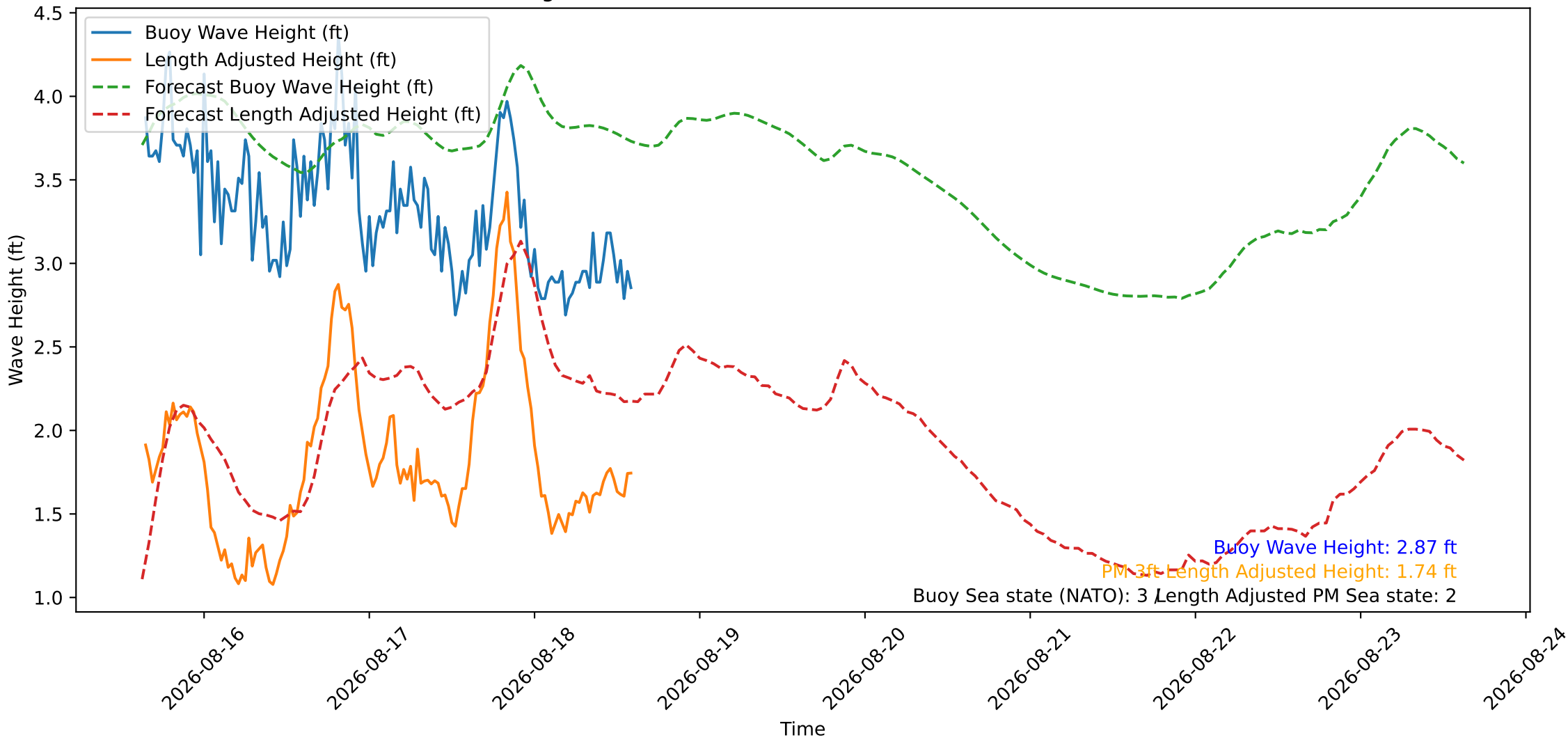
Wave Heights over Time for Green Beach at 2026-08-18 15:01:08
