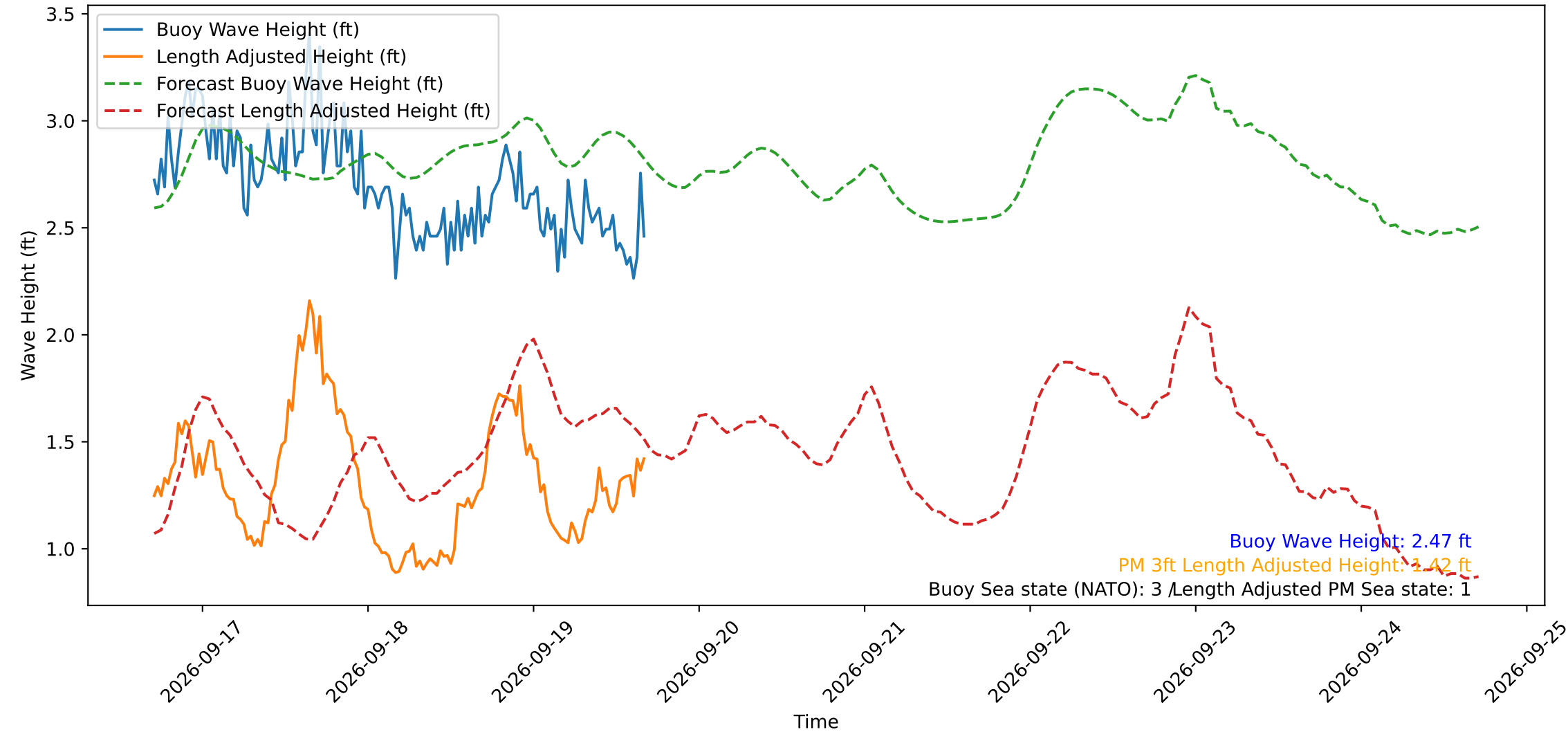
Wave Heights over Time for Red Beach at 2026-09-19 16:50:51
