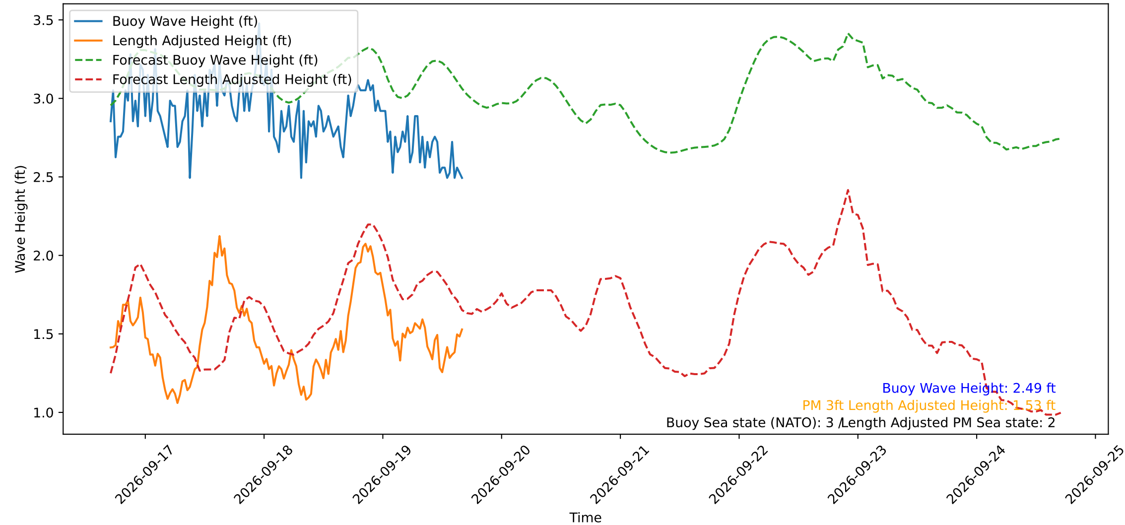
Wave Heights over Time for Green Beach at 2026-09-19 16:51:14
