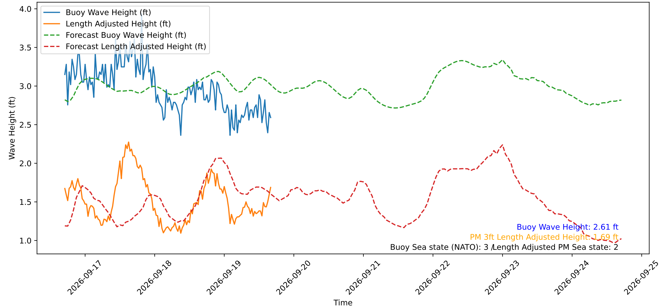
Wave Heights over Time for Oceanside Harbor at 2026-09-19 16:50:30
