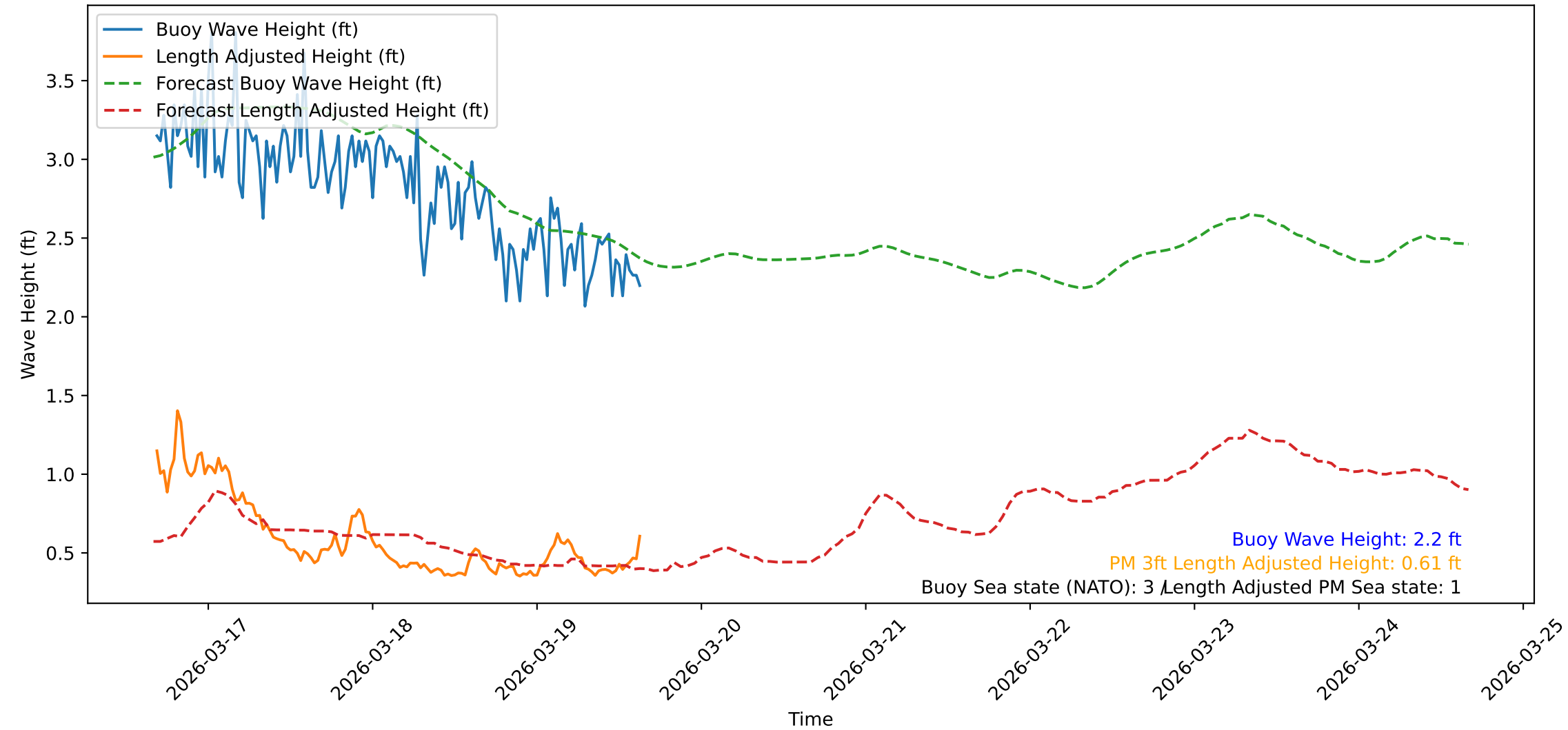
Wave Heights over Time for Red Beach at 2026-03-19 16:00:47
