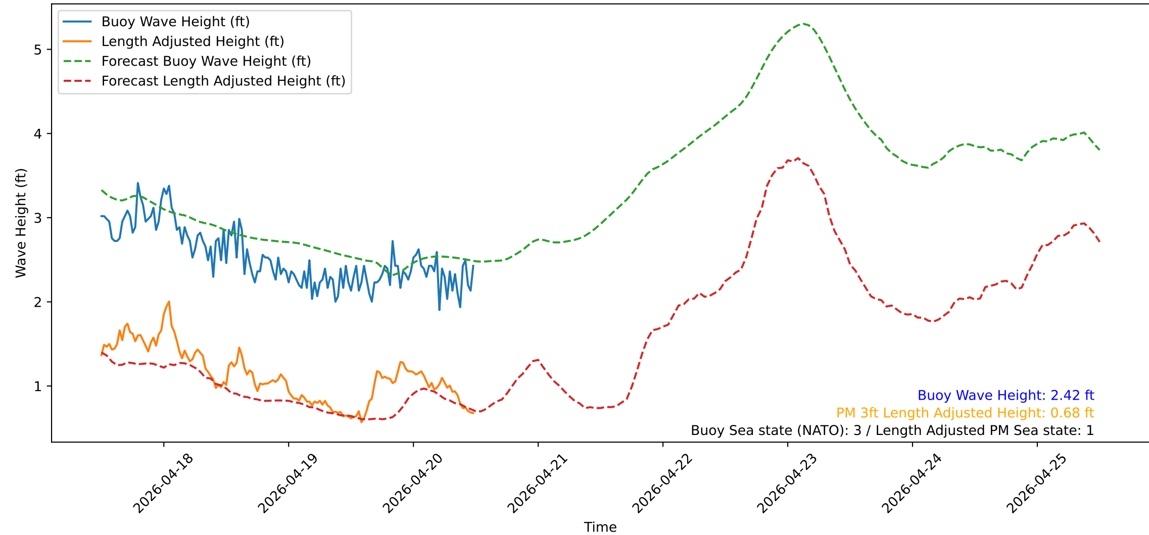
Wave Heights over Time for Oceanside Harbor at 2026-04-20 12:10:31
