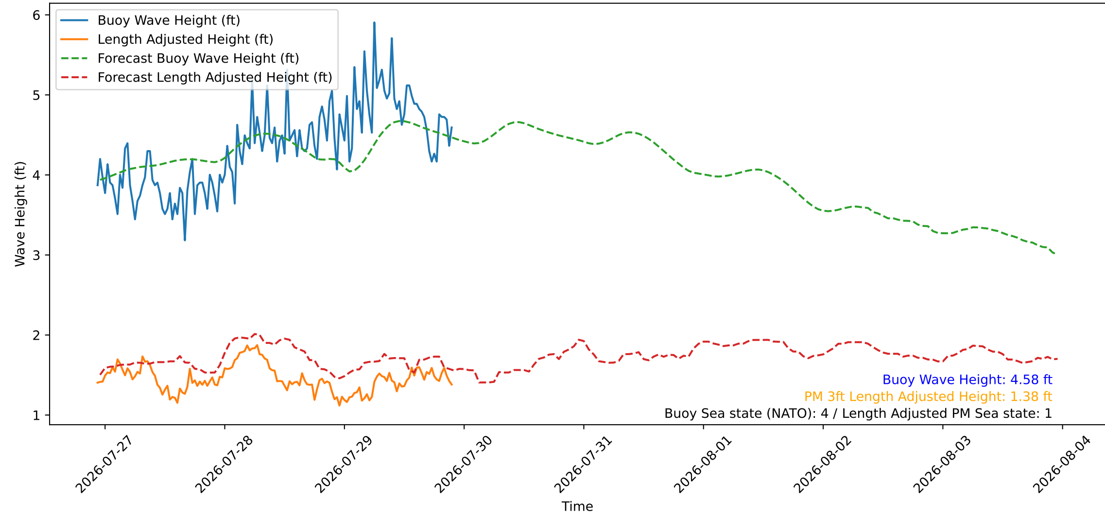
Wave Heights over Time for Oceanside Harbor at 2026-07-29 22:30:26
