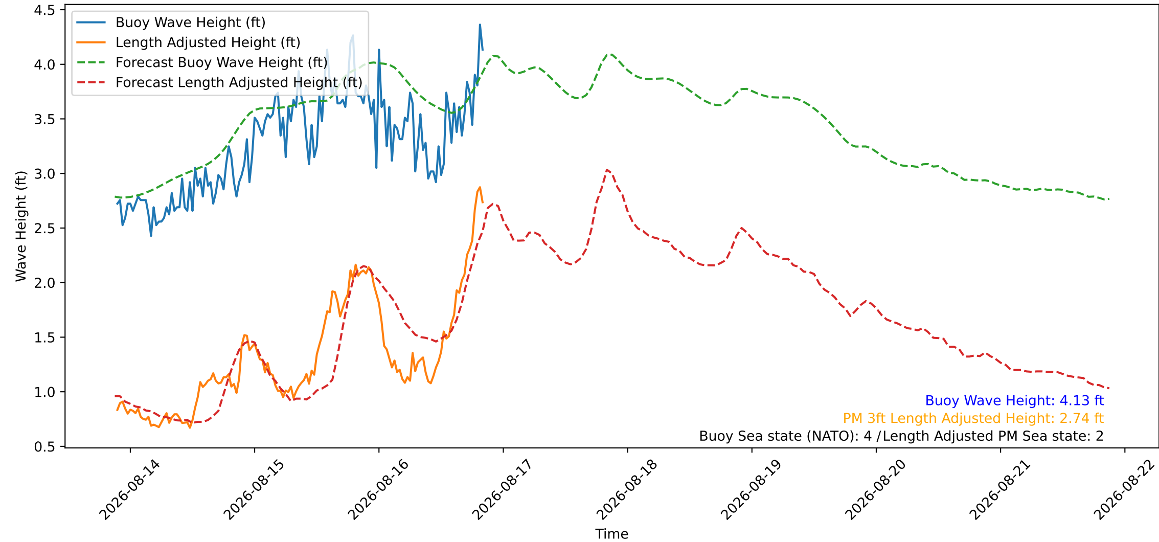
Wave Heights over Time for Green Beach at 2026-08-16 21:01:08
