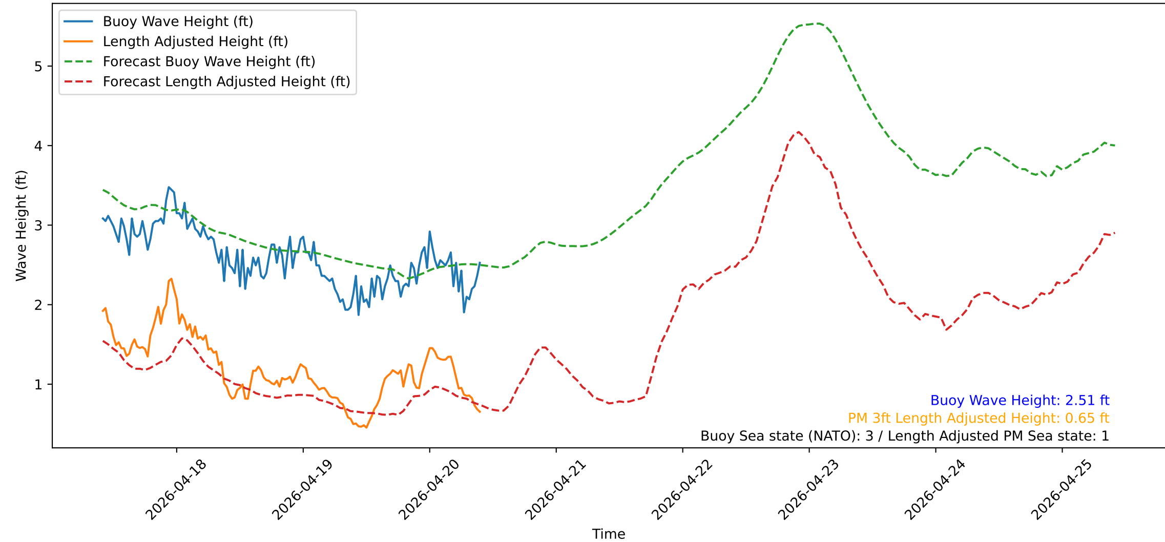
Wave Heights over Time for Green Beach at 2026-04-20 10:11:13
