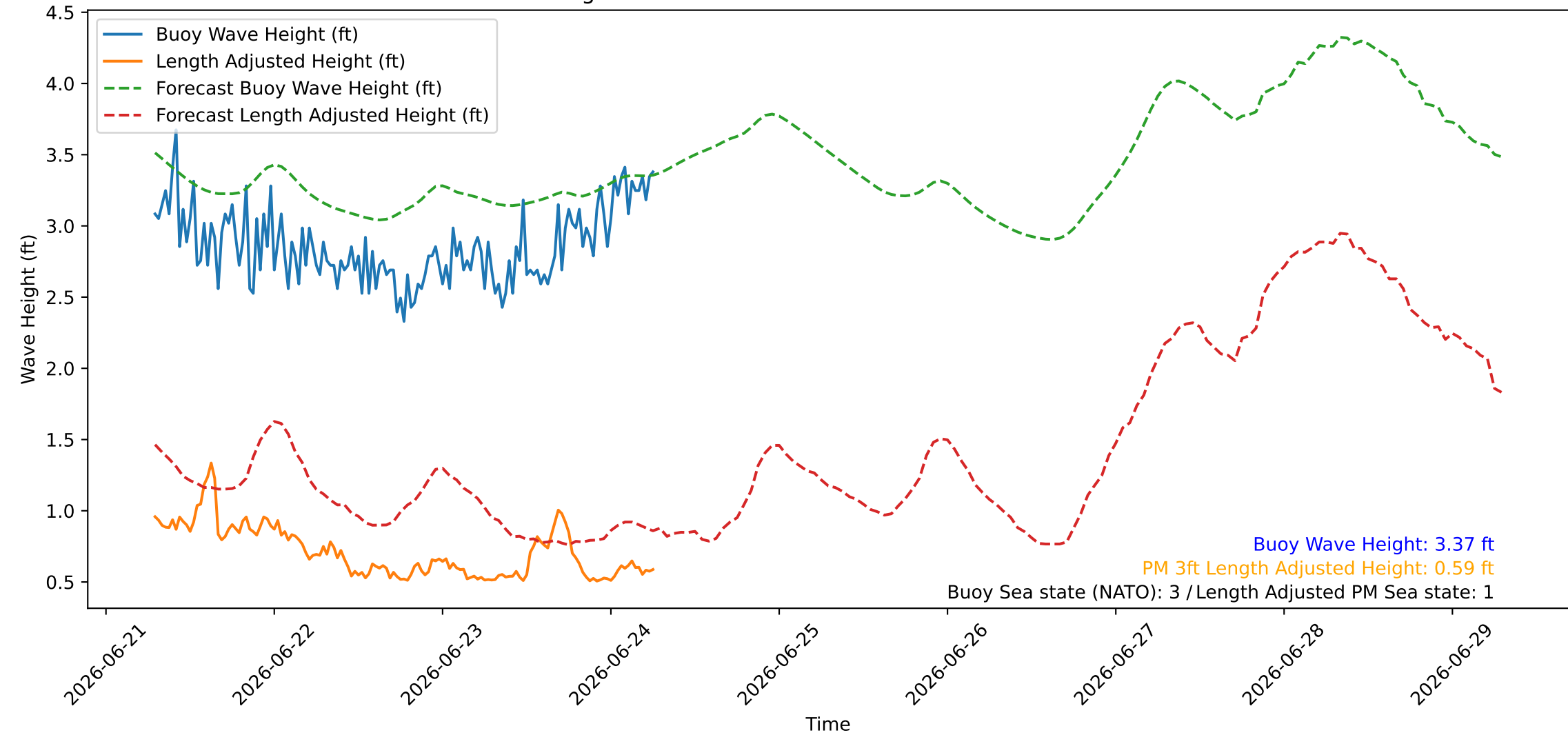
Wave Heights over Time for Red Beach at 2026-06-24 06:50:46
