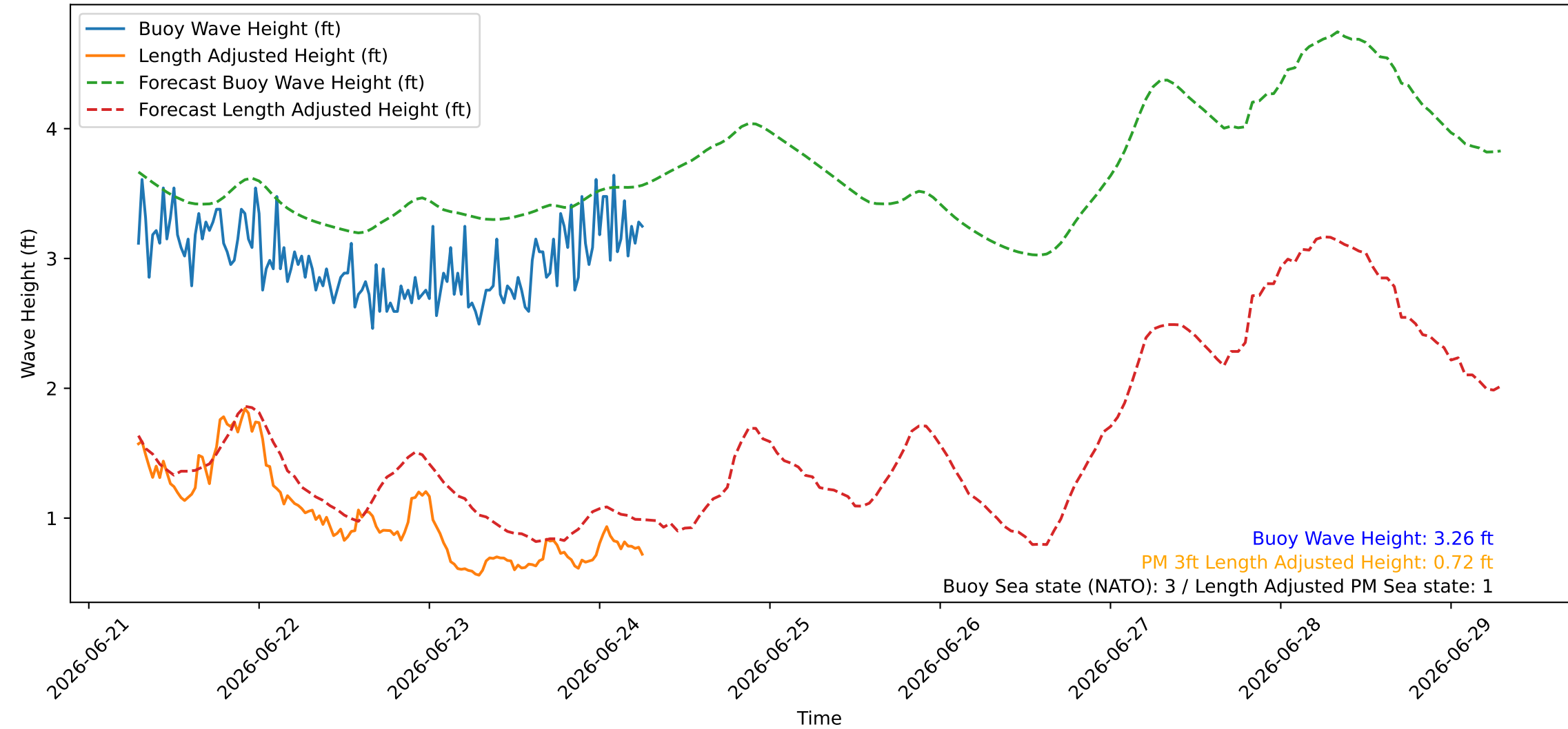
Wave Heights over Time for Green Beach at 2026-06-24 06:51:08
