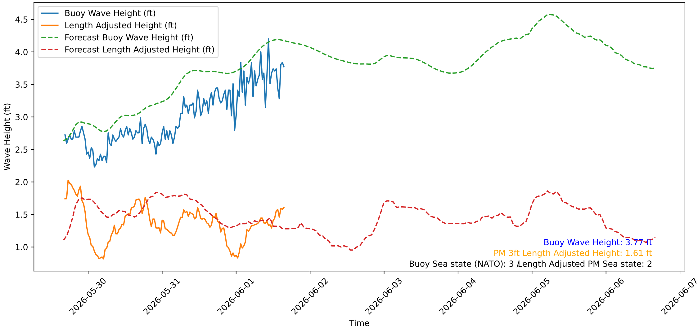
Wave Heights over Time for Red Beach at 2026-06-01 16:20:46
