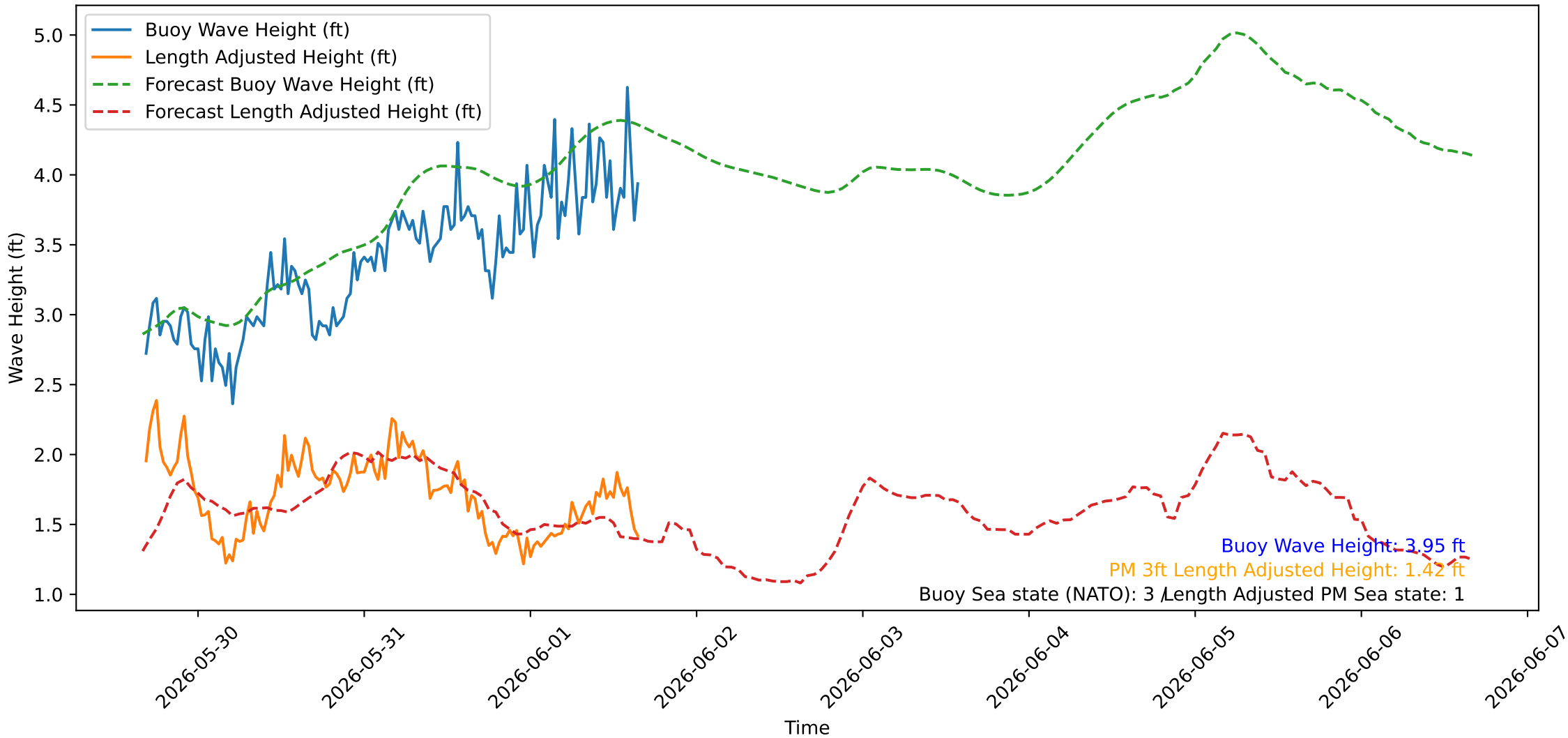
Wave Heights over Time for Oceanside Harbor at 2026-06-01 16:20:26
