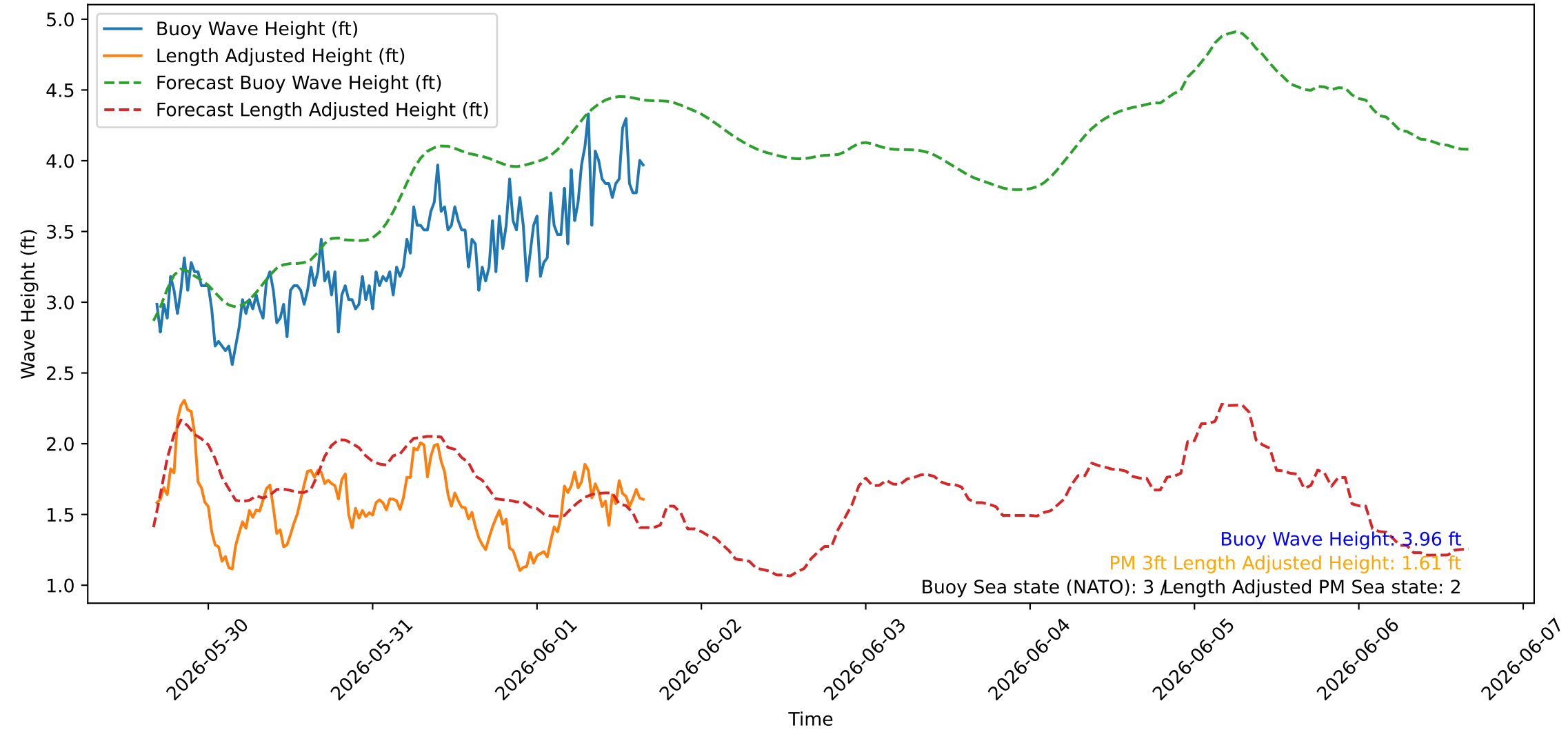
Wave Heights over Time for Green Beach at 2026-06-01 16:21:09
