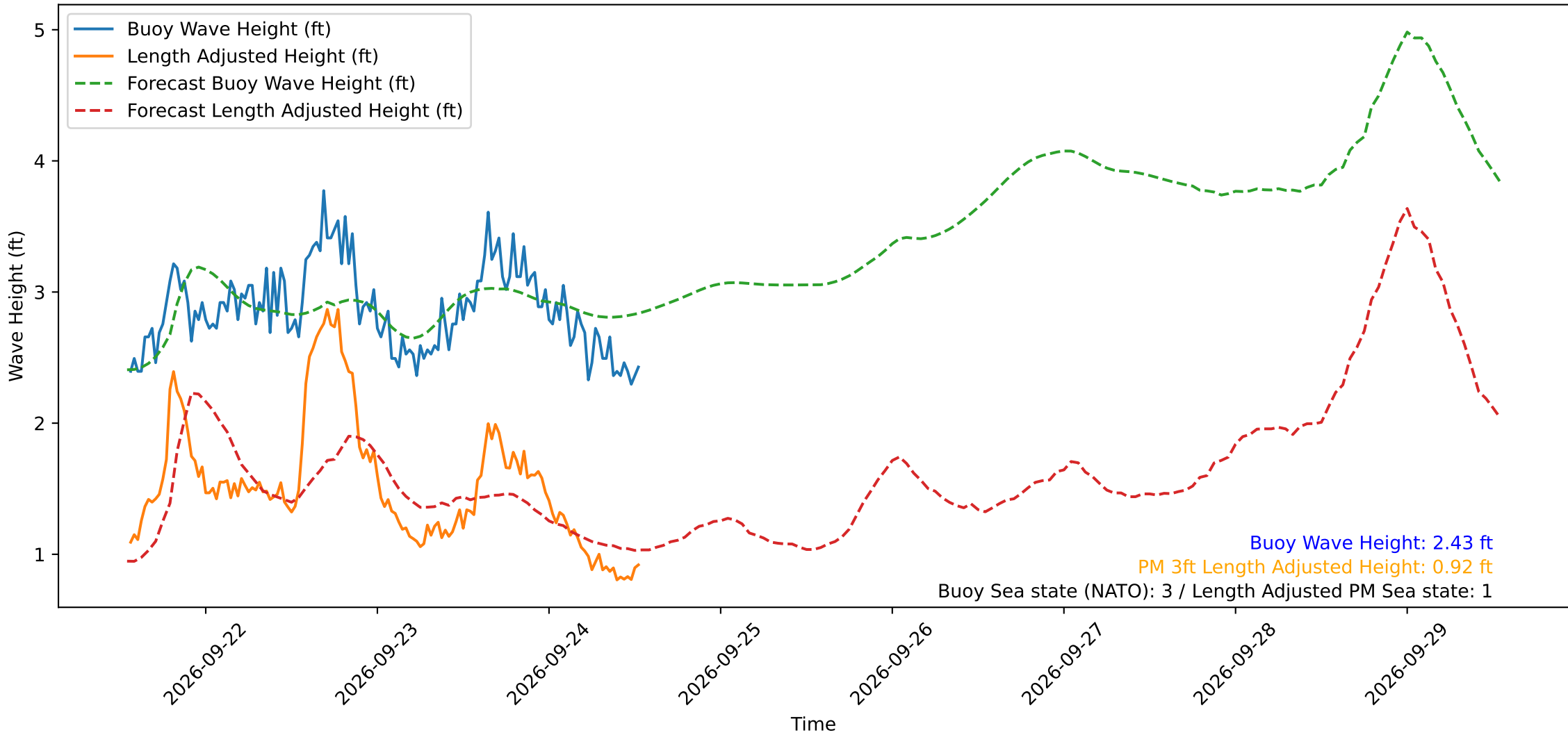
Wave Heights over Time for Oceanside Harbor at 2026-09-24 13:20:31
