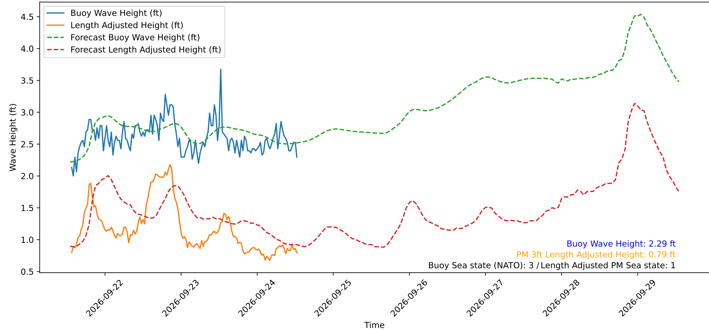
Wave Heights over Time for Red Beach at 2026-09-24 13:20:53
