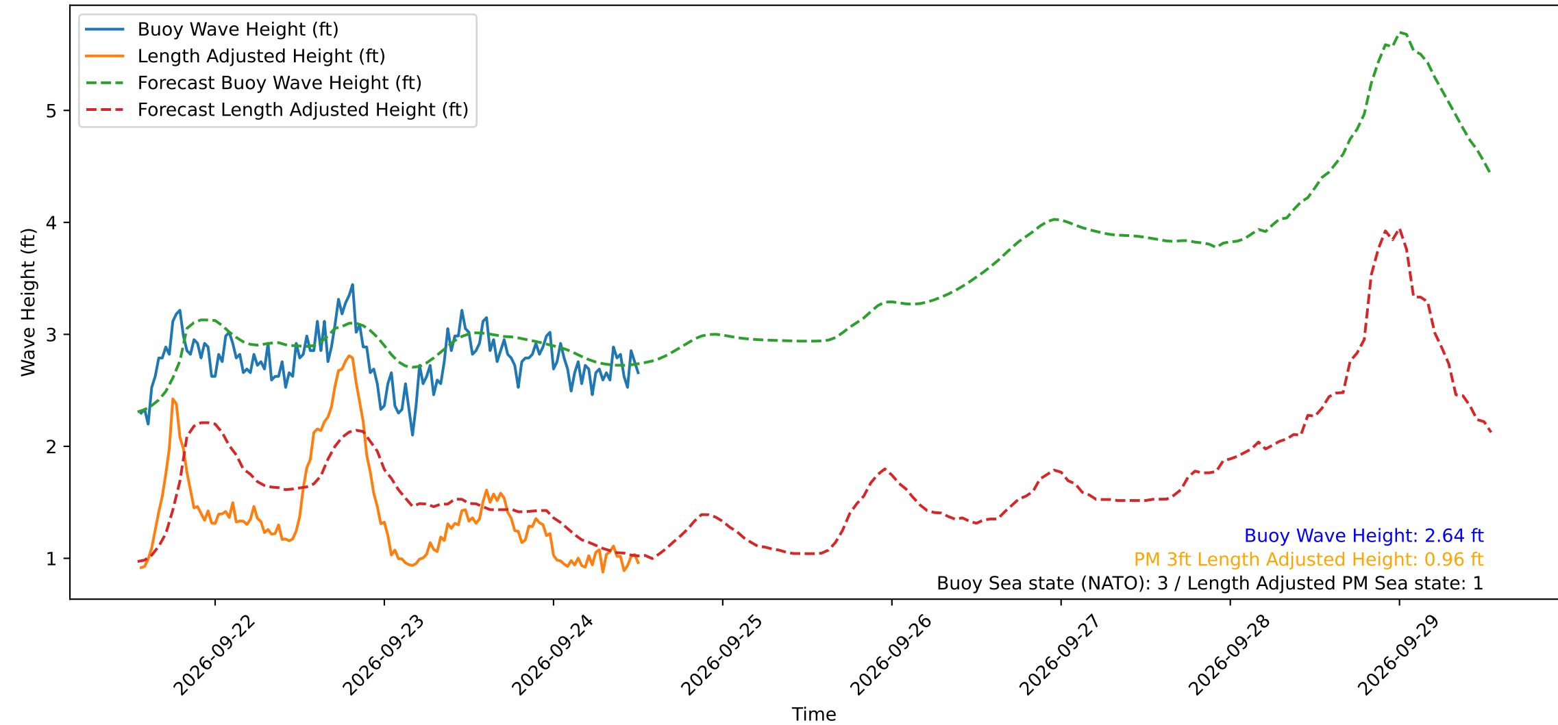
Wave Heights over Time for Green Beach at 2026-09-24 13:21:19
