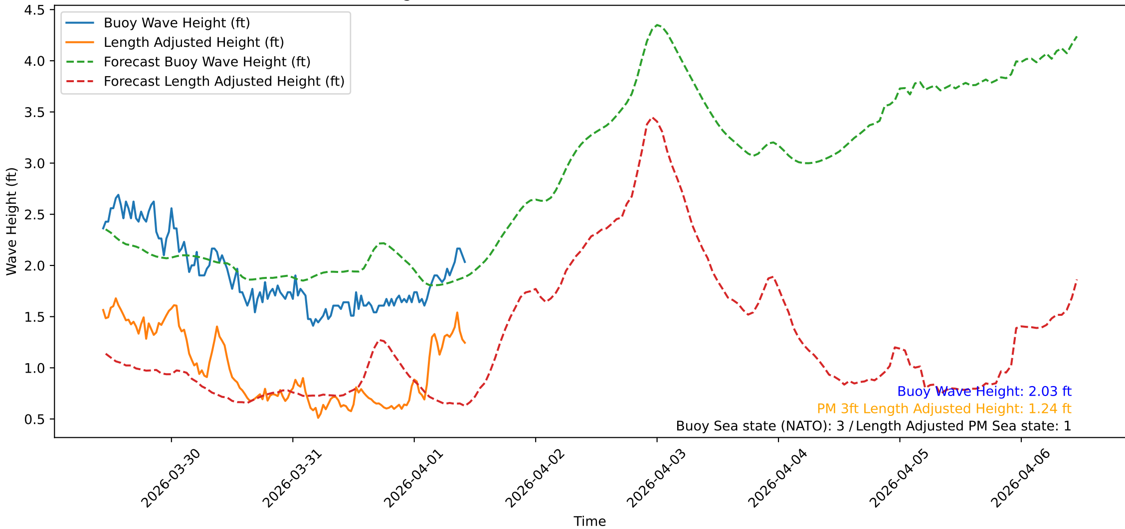
Wave Heights over Time for Green Beach at 2026-04-01 10:41:11
