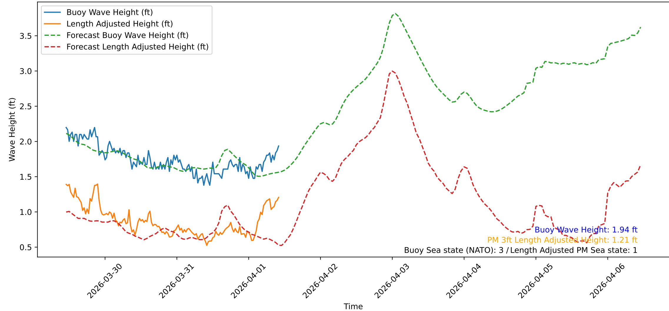
Wave Heights over Time for Red Beach at 2026-04-01 10:40:48
