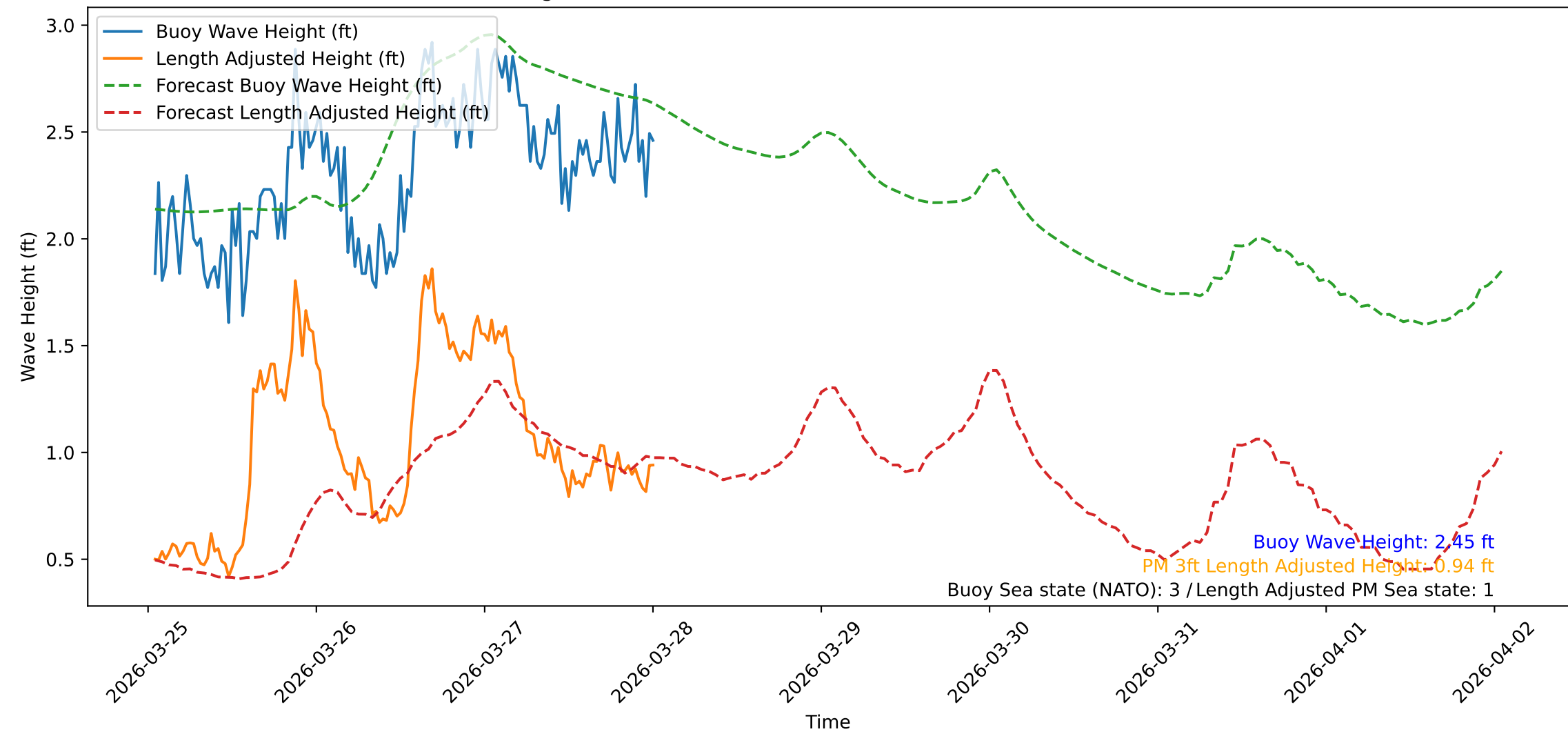
Wave Heights over Time for Oceanside Harbor at 2026-03-28 01:00:31
