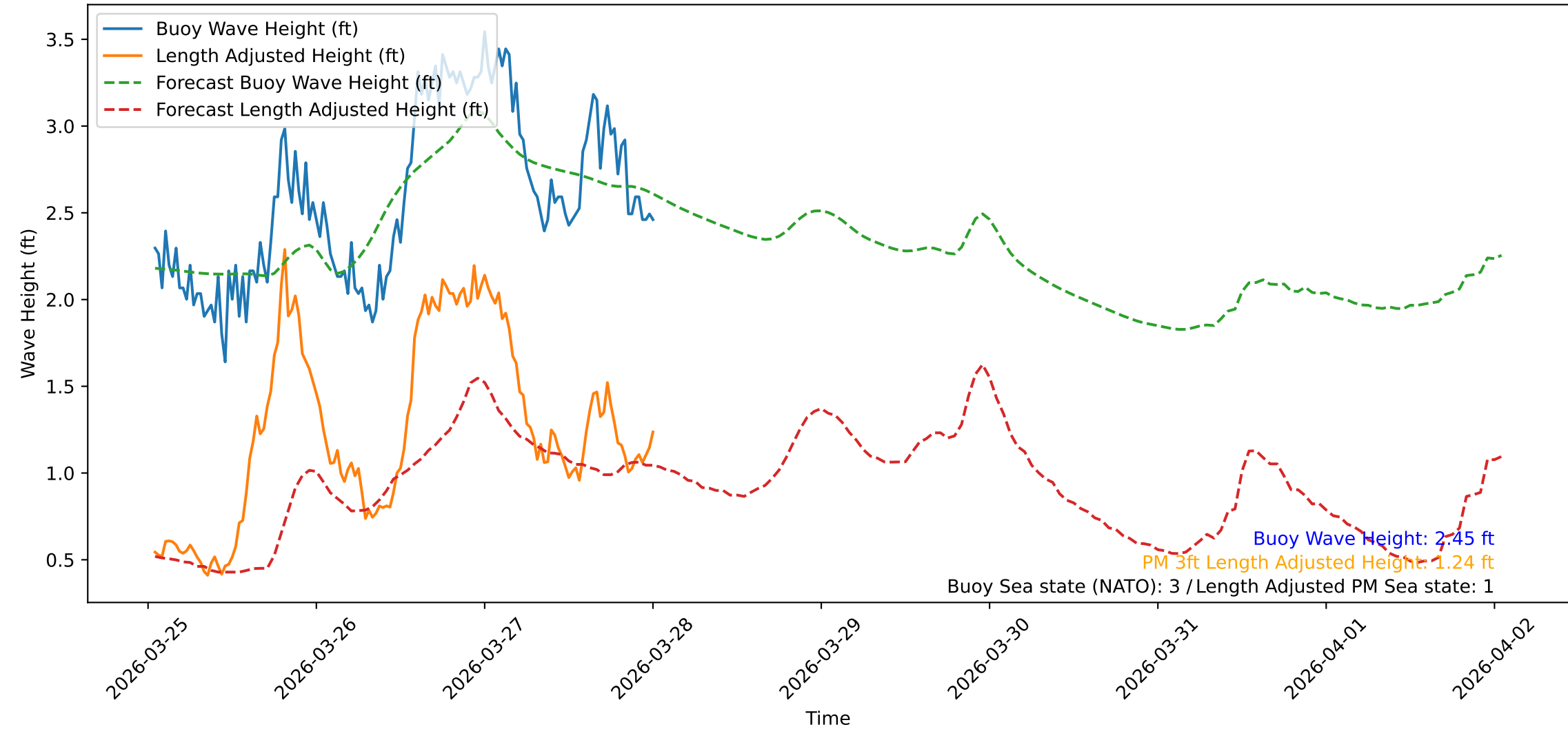
Wave Heights over Time for Green Beach at 2026-03-28 01:01:09
