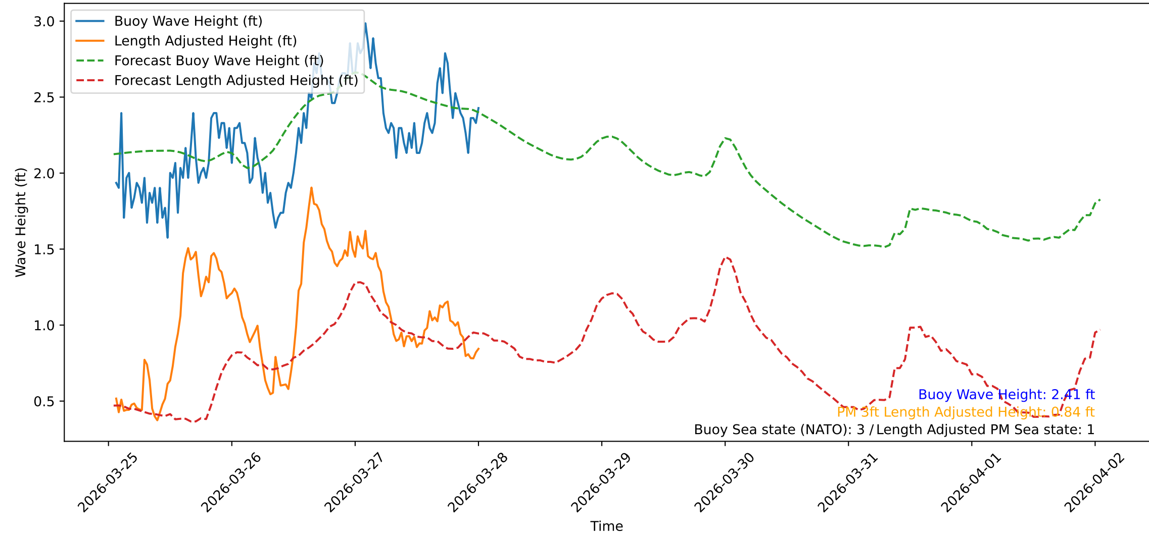
Wave Heights over Time for Red Beach at 2026-03-28 01:00:47
