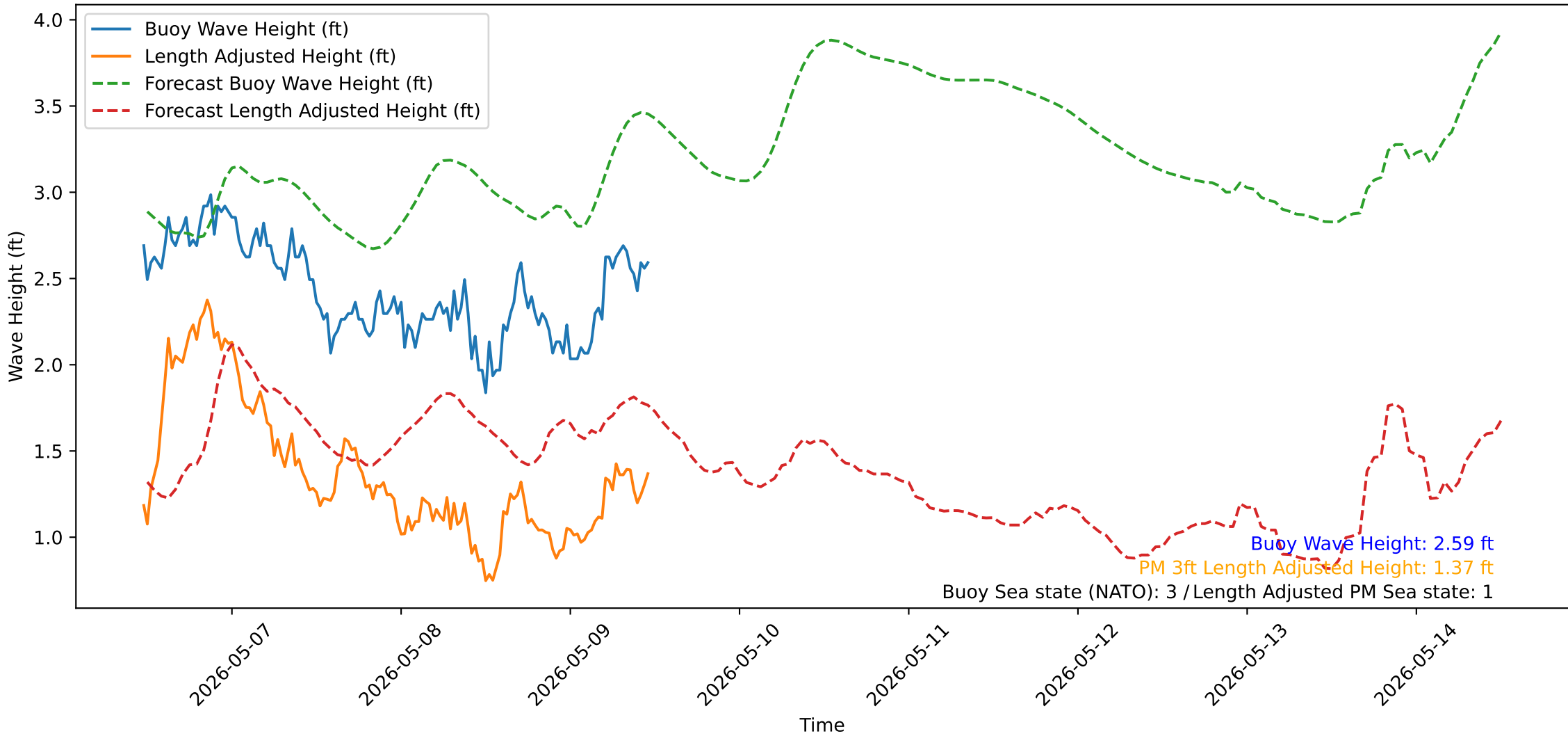
Wave Heights over Time for Green Beach at 2026-05-09 11:41:14
