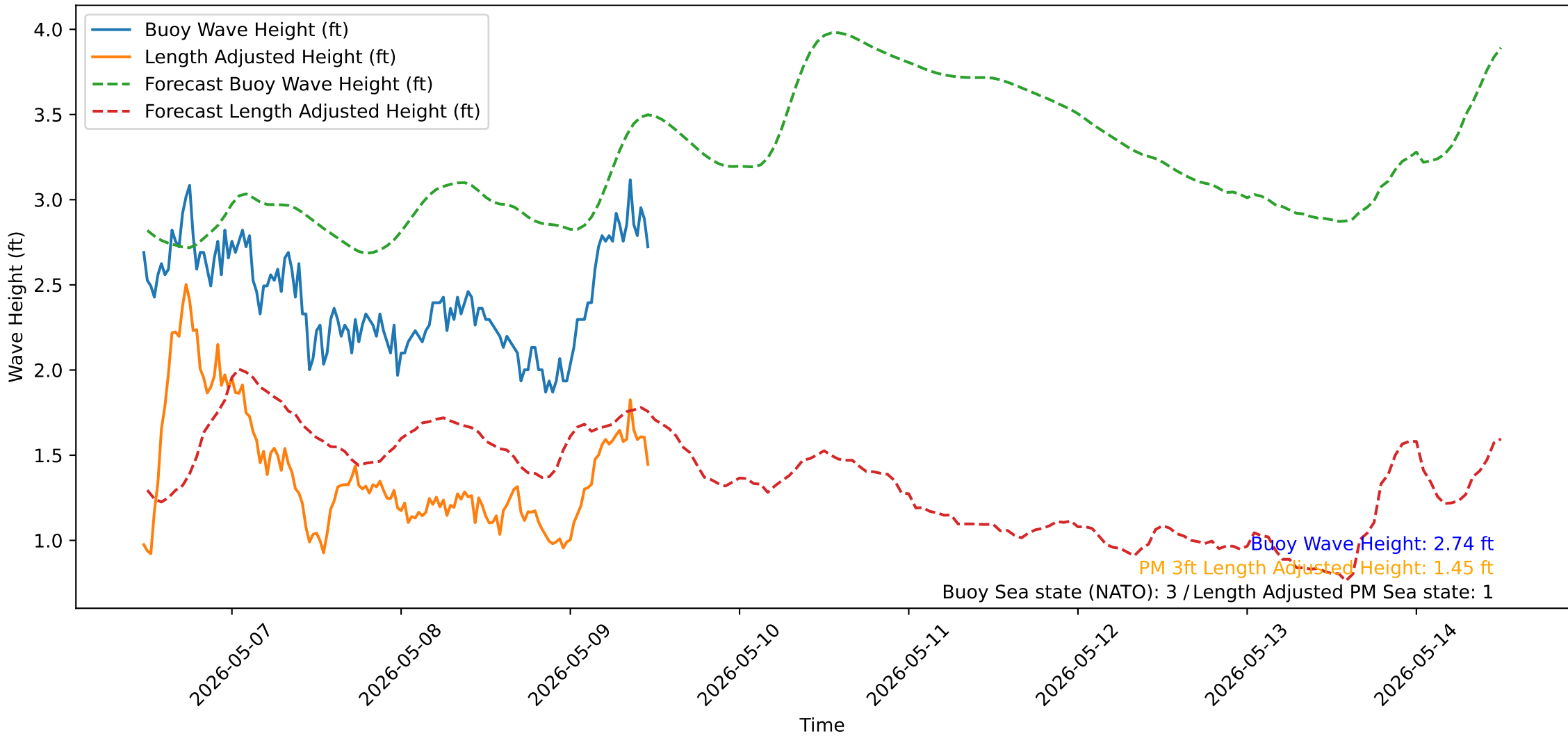
Wave Heights over Time for Oceanside Harbor at 2026-05-09 11:40:31
