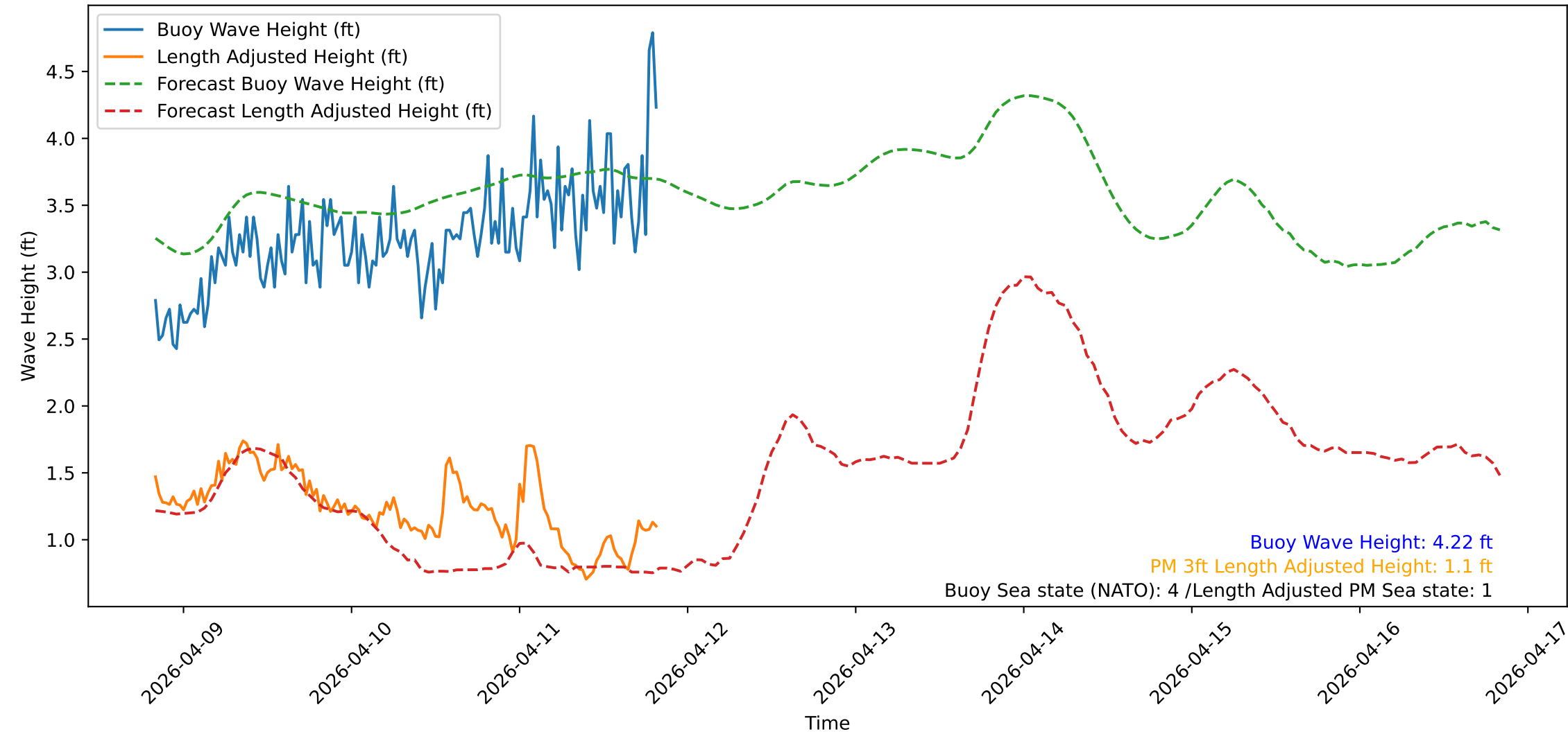
Wave Heights over Time for Oceanside Harbor at 2026-04-11 20:10:31
