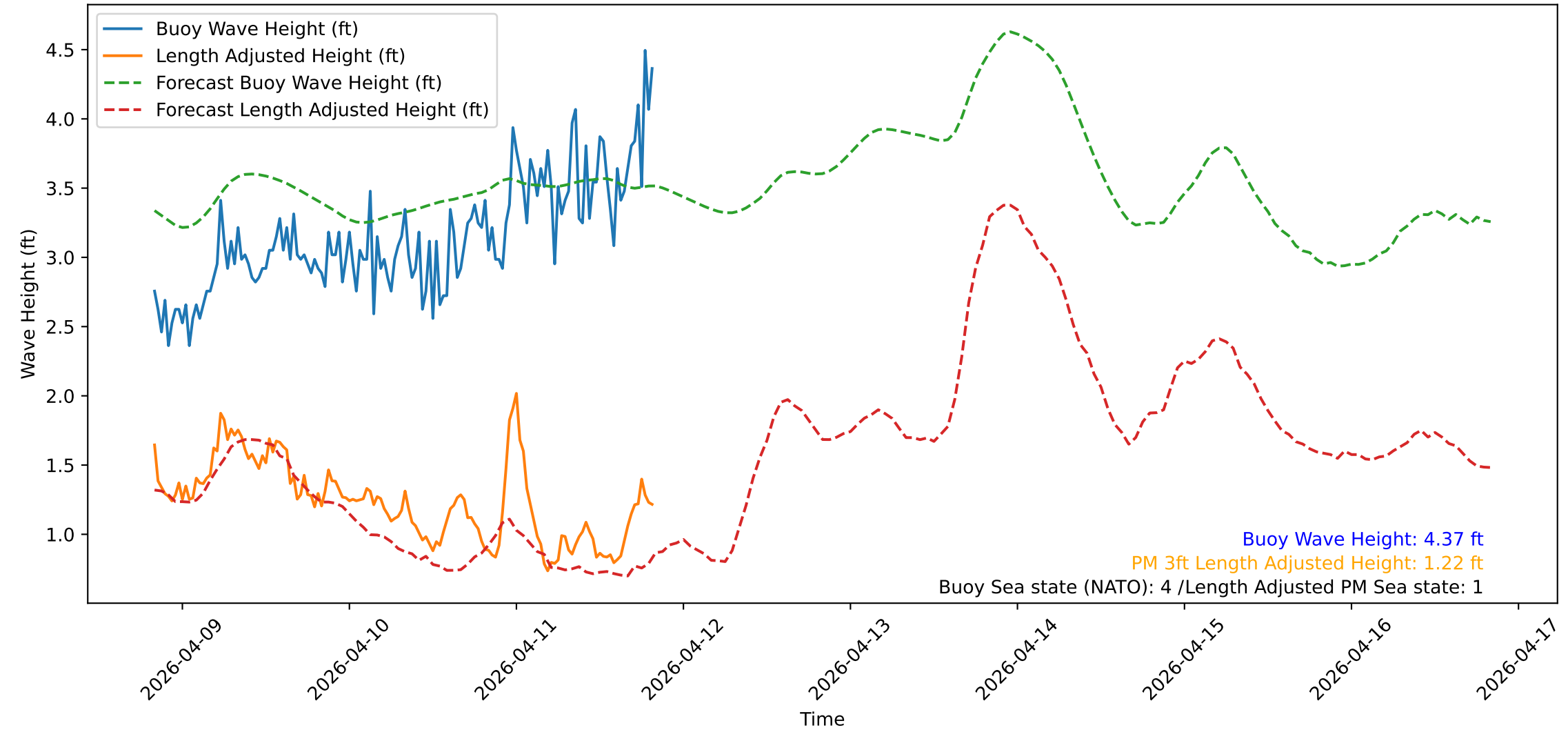
Wave Heights over Time for Green Beach at 2026-04-11 20:11:12
