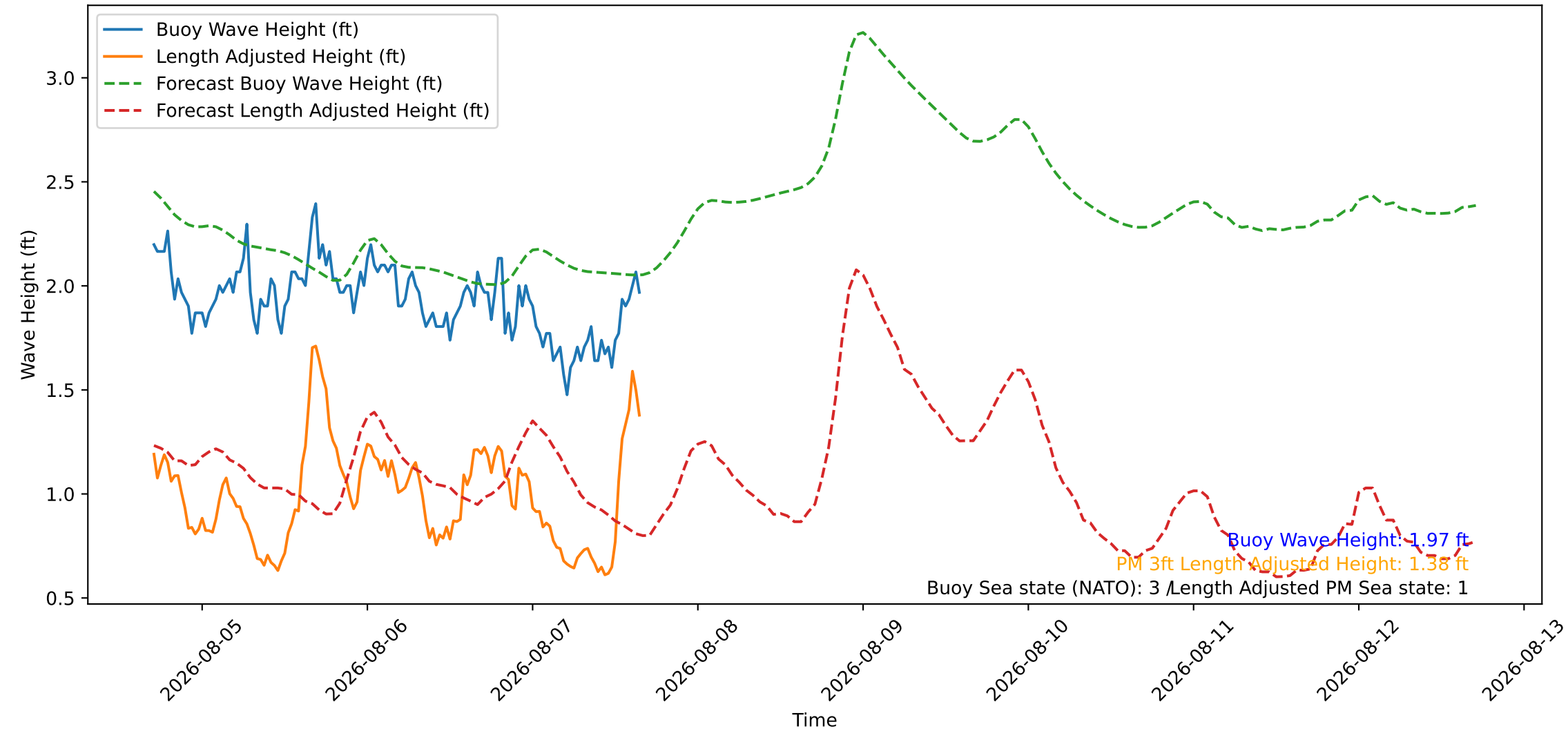
Wave Heights over Time for Red Beach at 2026-08-07 16:30:46
