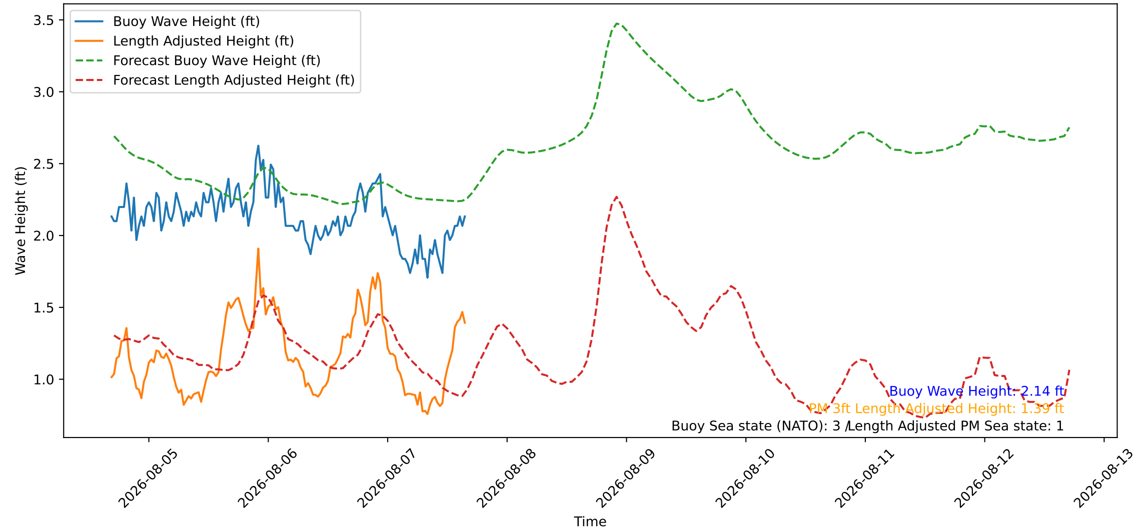
Wave Heights over Time for Green Beach at 2026-08-07 16:31:08
