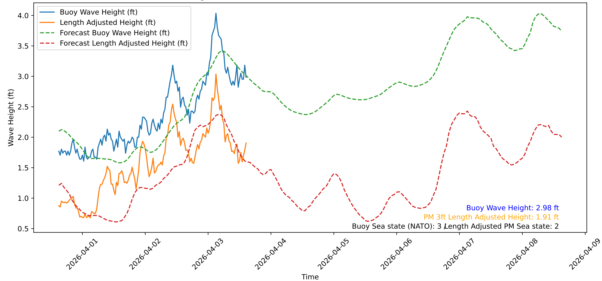
Wave Heights over Time for Oceanside Harbor at 2026-04-03 15:10:32
