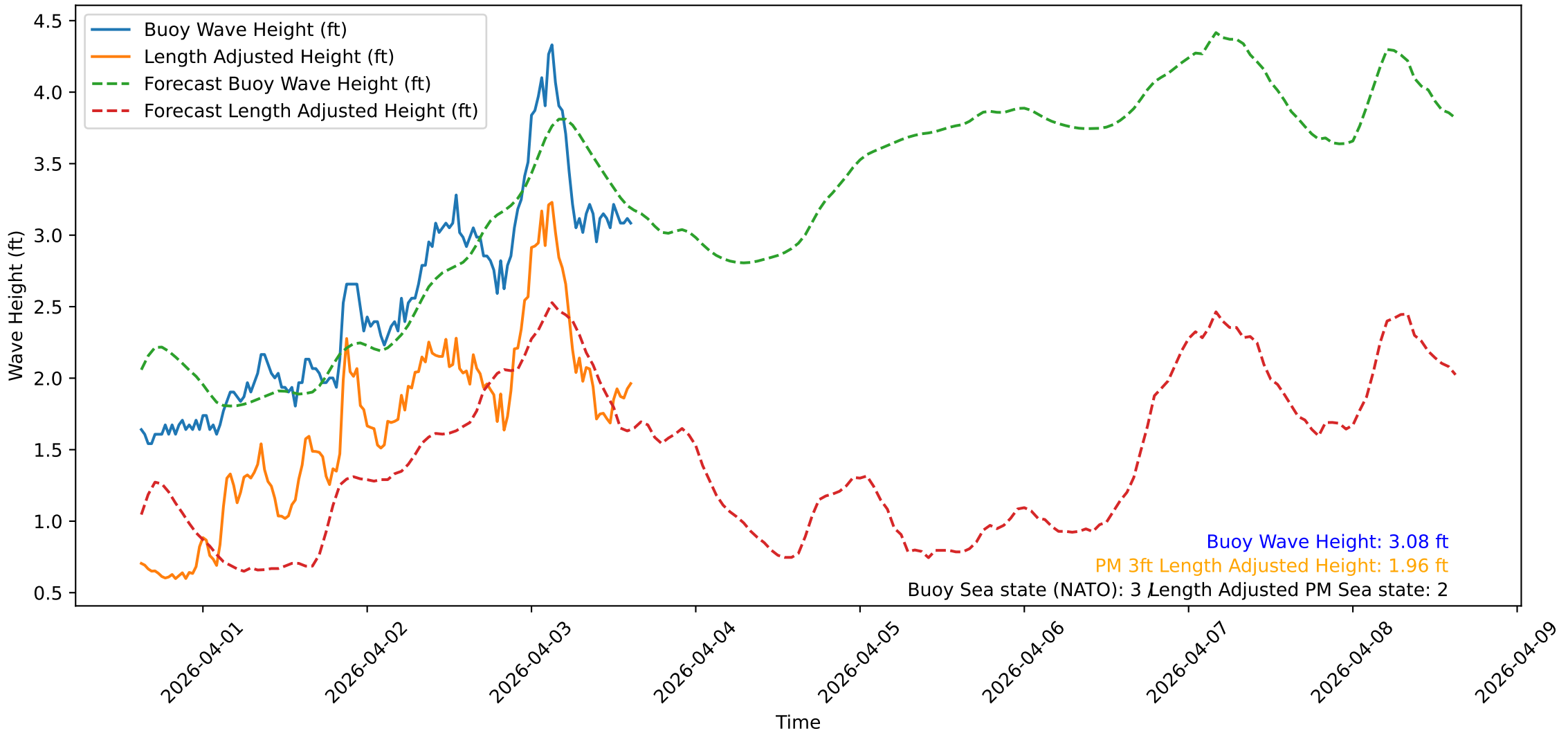
Wave Heights over Time for Green Beach at 2026-04-03 15:11:10
