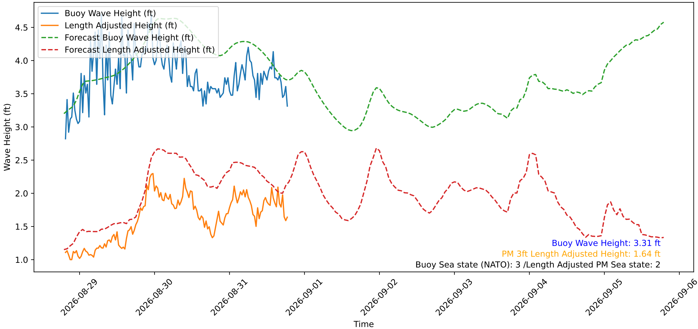
Wave Heights over Time for Red Beach at 2026-08-31 19:20:50
