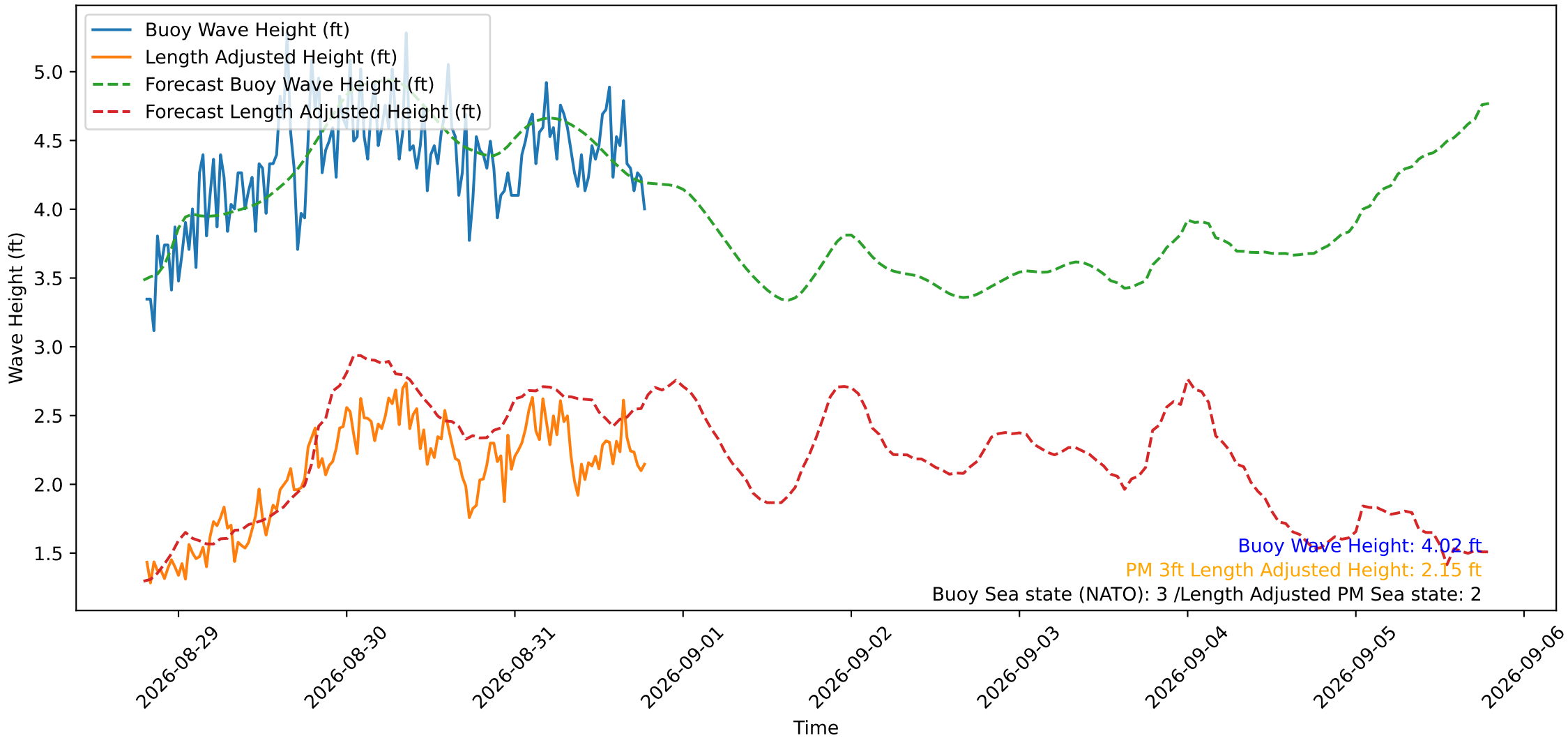
Wave Heights over Time for Oceanside Harbor at 2026-08-31 19:20:29
