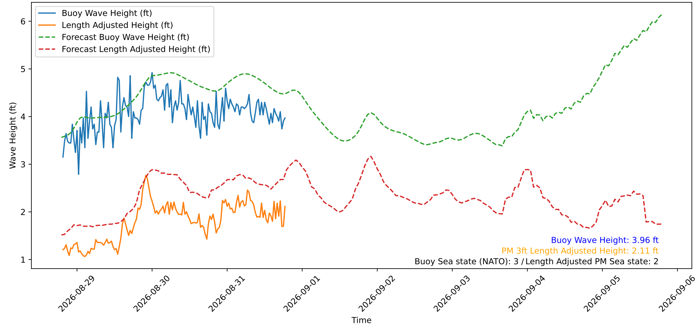
Wave Heights over Time for Green Beach at 2026-08-31 19:21:14
