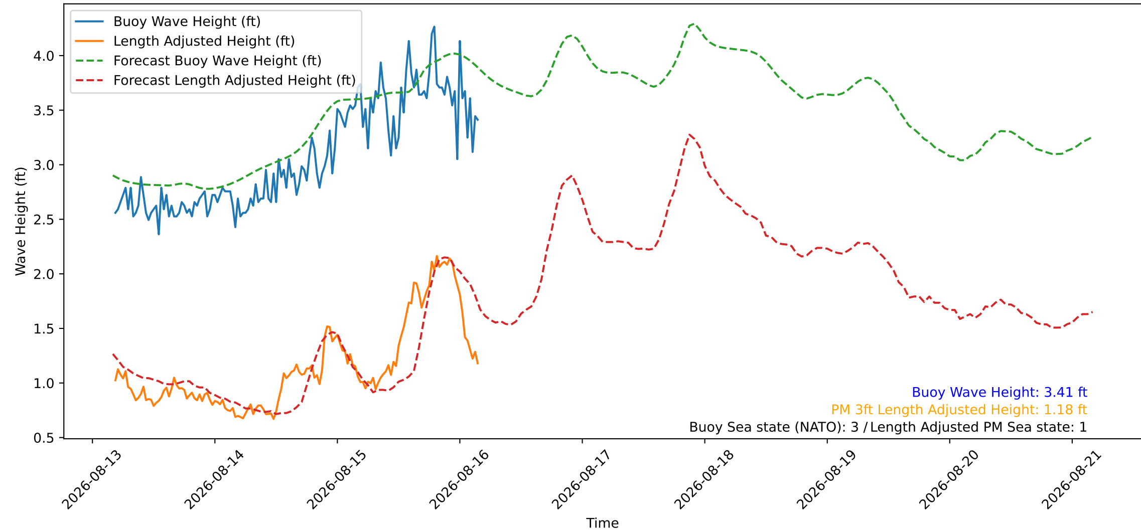
Wave Heights over Time for Green Beach at 2026-08-16 04:11:08
