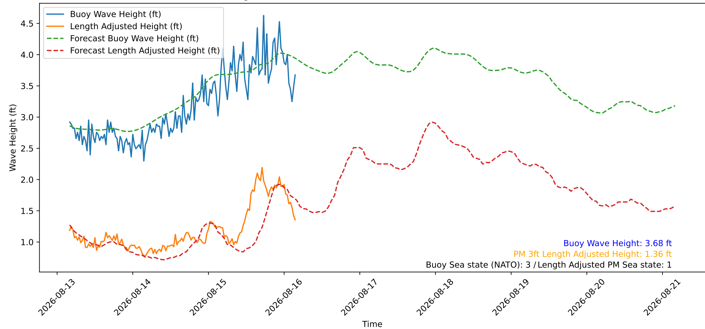
Wave Heights over Time for Oceanside Harbor at 2026-08-16 04:10:26
