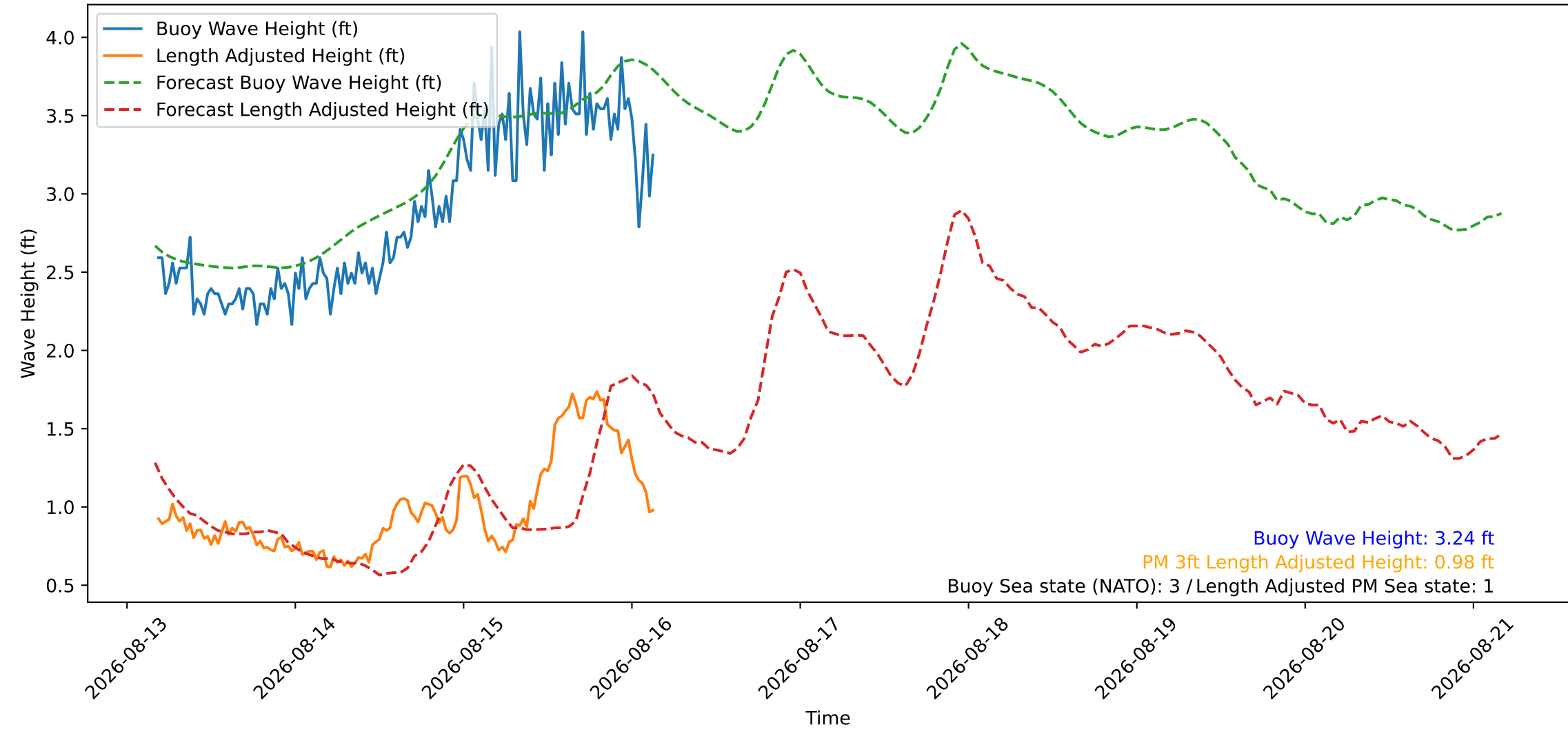
Wave Heights over Time for Red Beach at 2026-08-16 04:10:46
