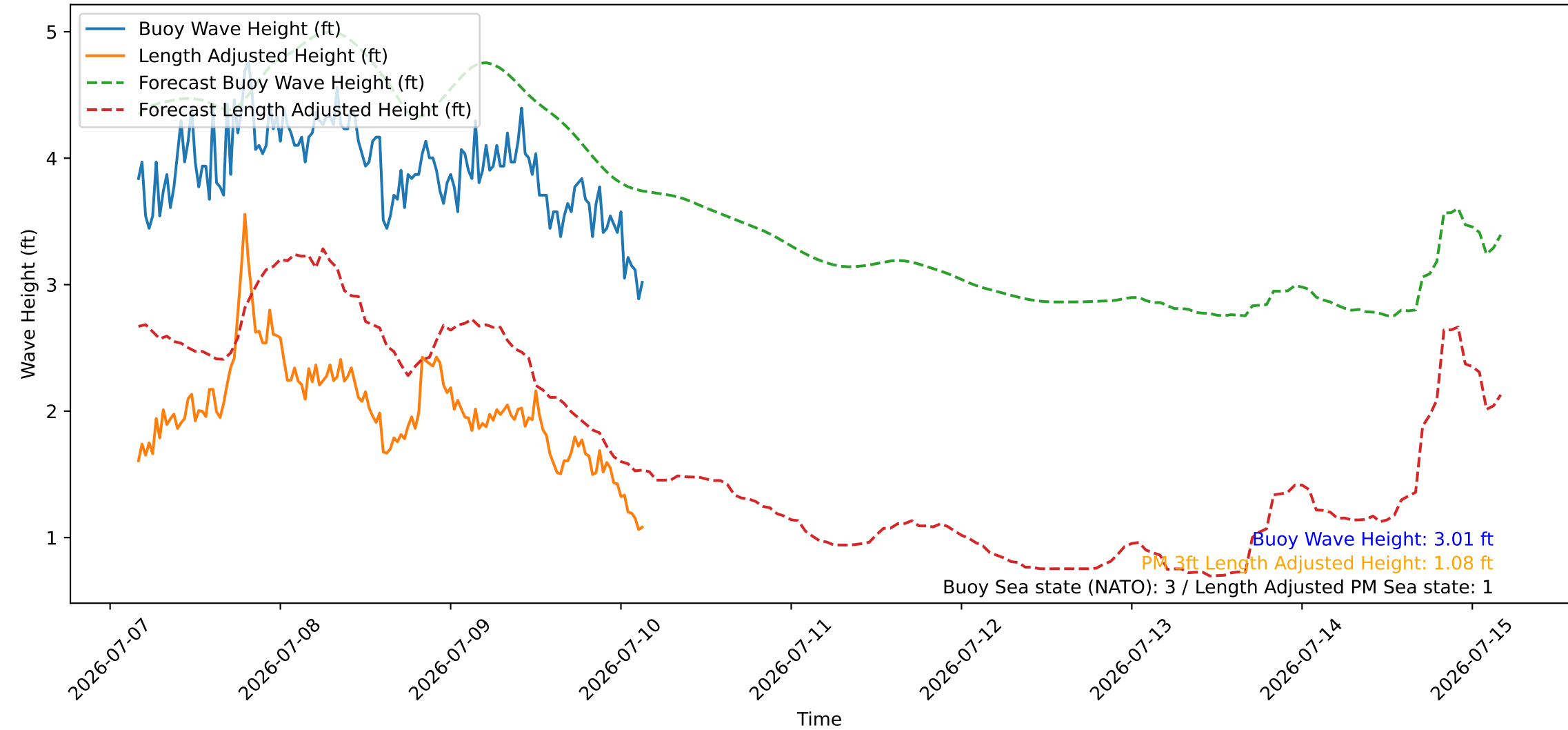
Wave Heights over Time for Green Beach at 2026-07-10 04:01:08
