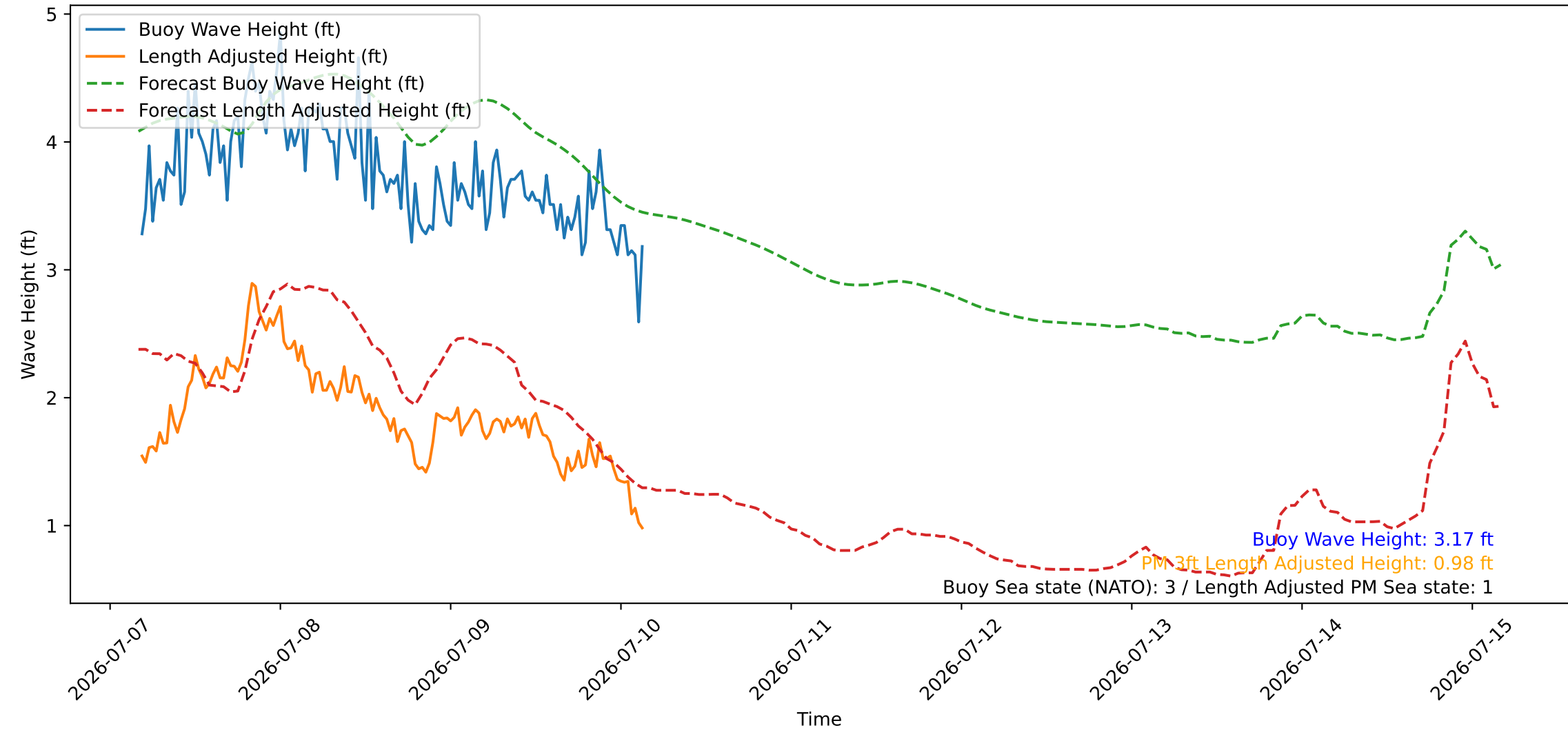
Wave Heights over Time for Red Beach at 2026-07-10 04:00:46
