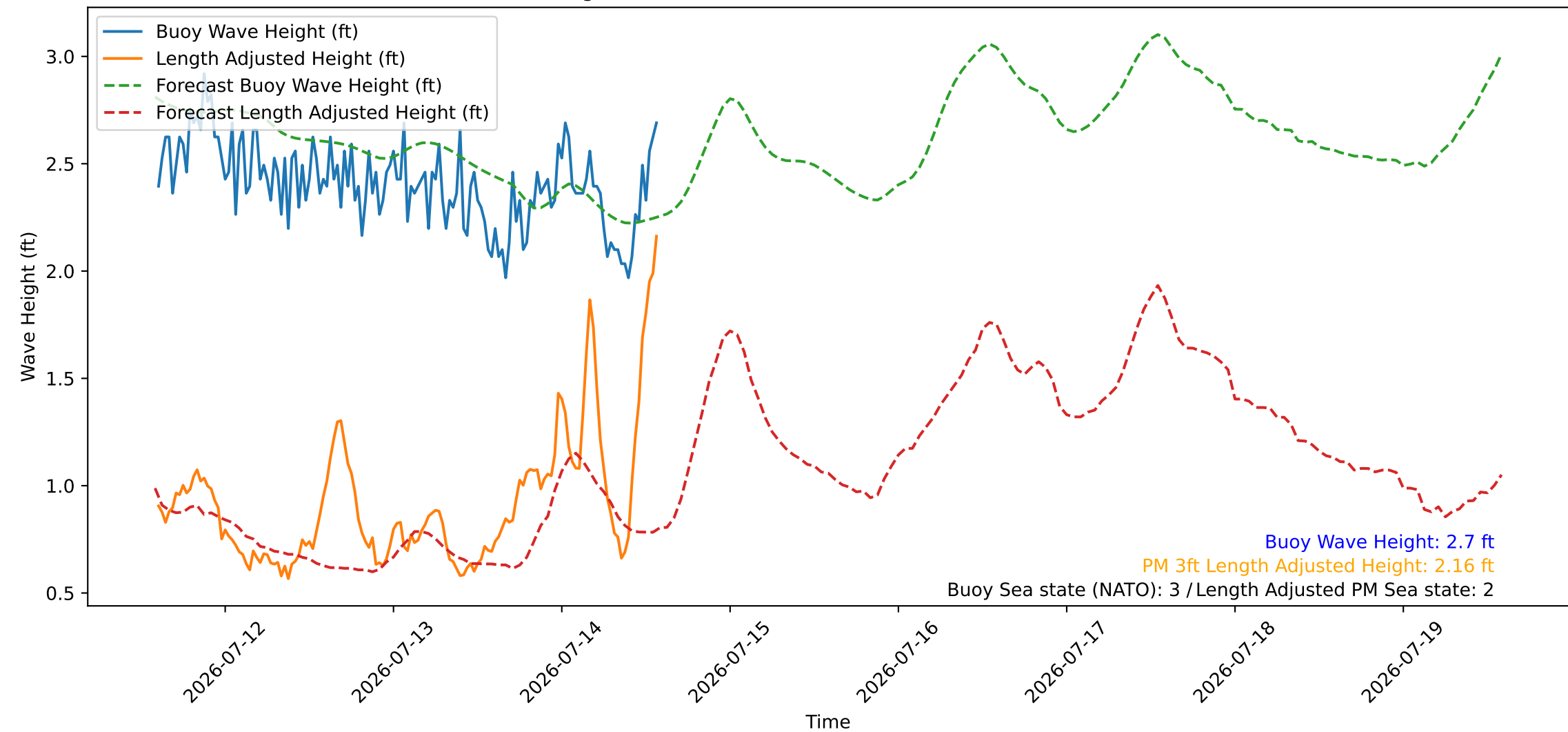
Wave Heights over Time for Red Beach at 2026-07-14 14:20:46
