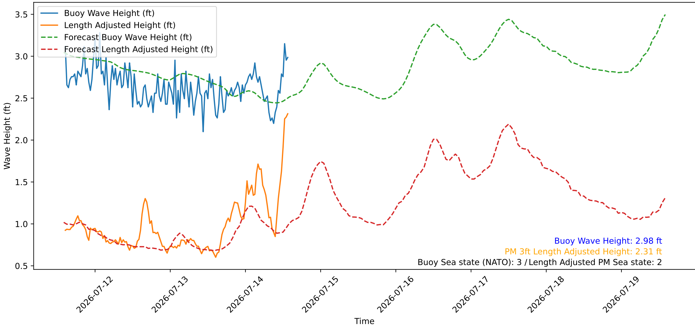
Wave Heights over Time for Oceanside Harbor at 2026-07-14 14:20:26
