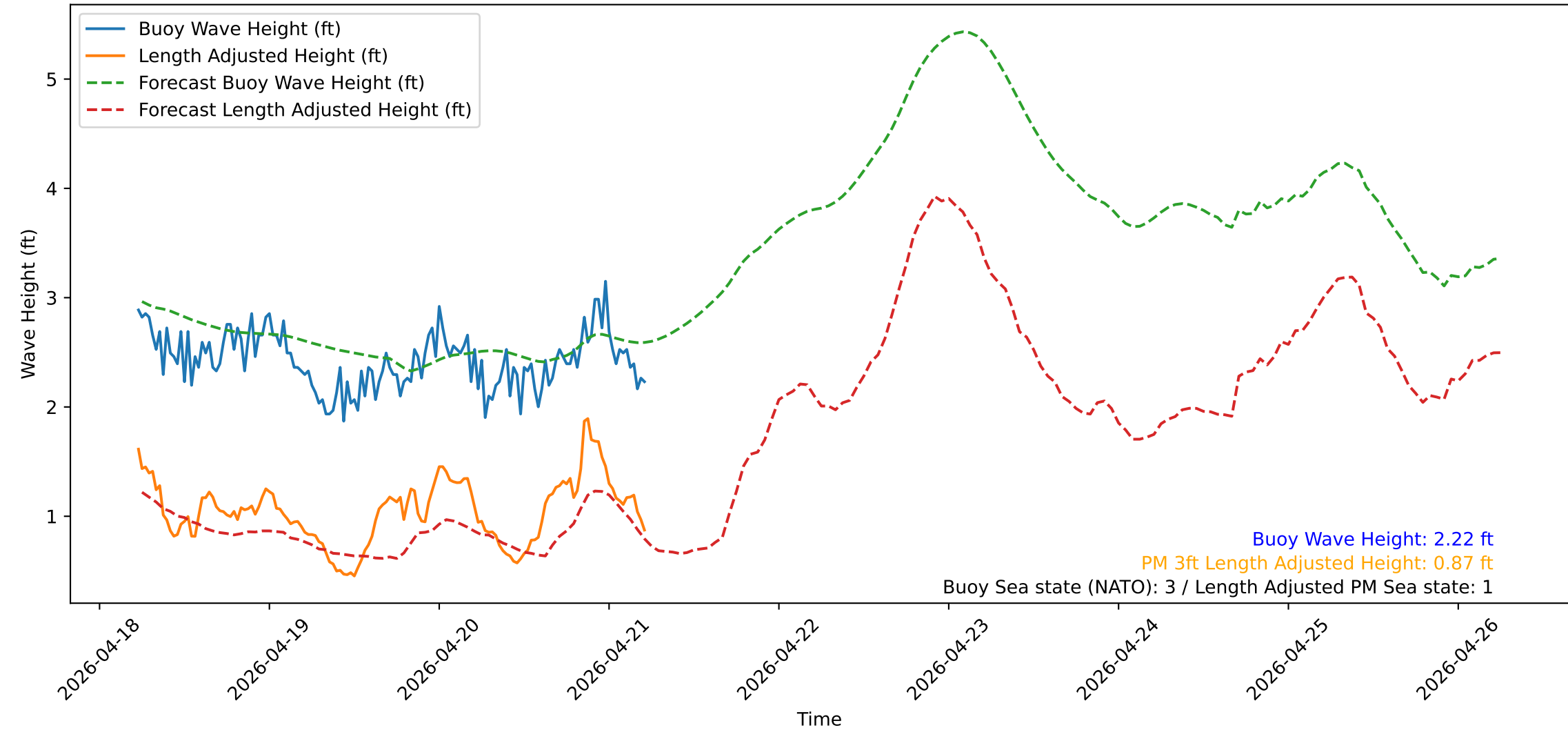
Wave Heights over Time for Green Beach at 2026-04-21 05:41:13
