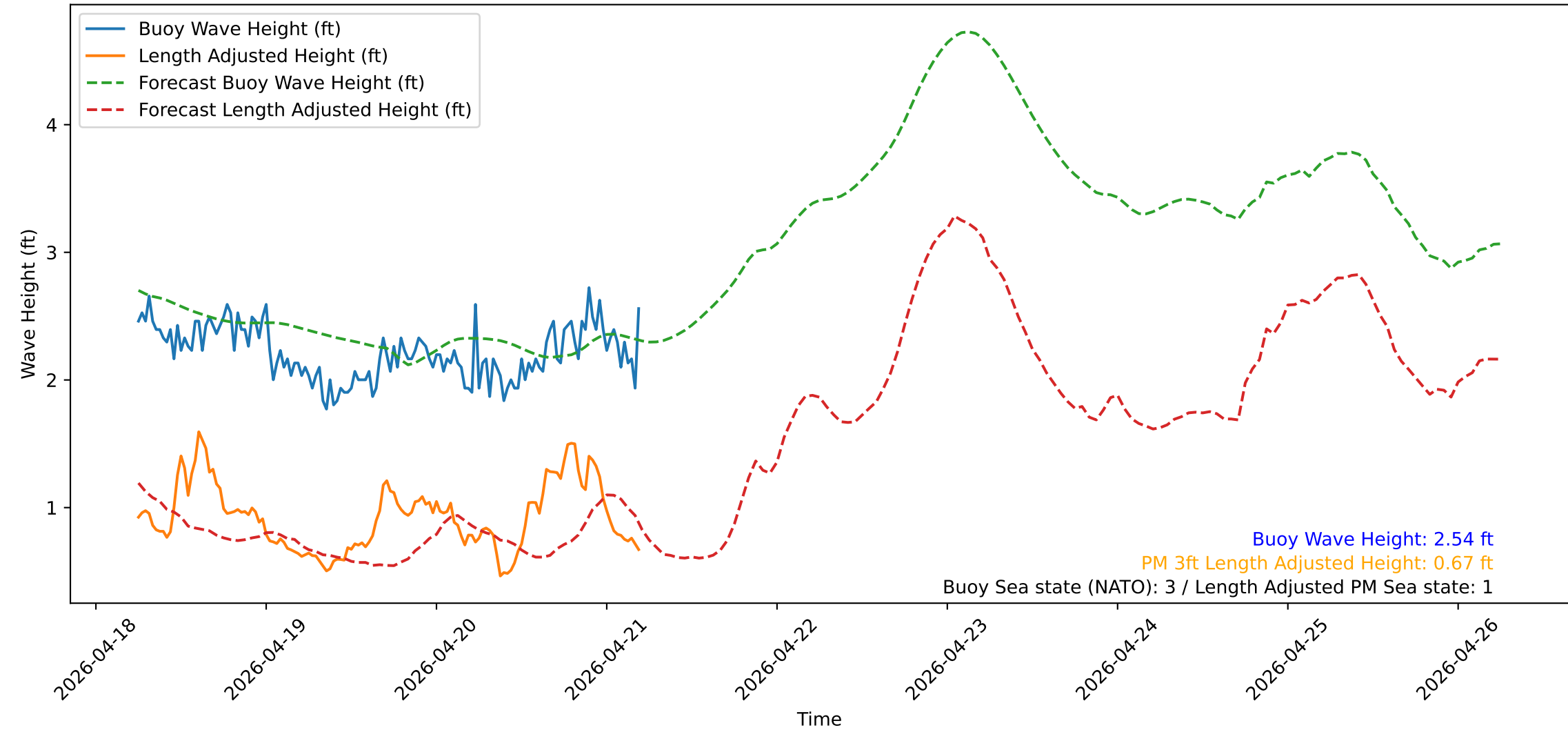
Wave Heights over Time for Red Beach at 2026-04-21 05:40:51
