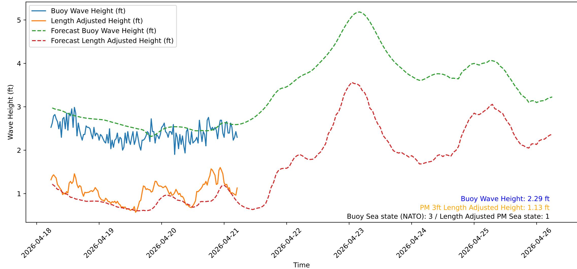
Wave Heights over Time for Oceanside Harbor at 2026-04-21 05:40:31
