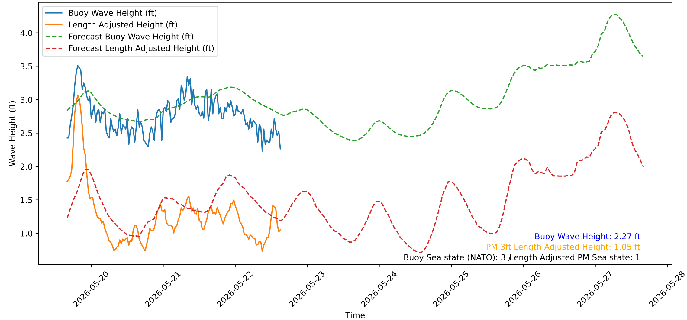
Wave Heights over Time for Red Beach at 2026-05-22 15:40:51
