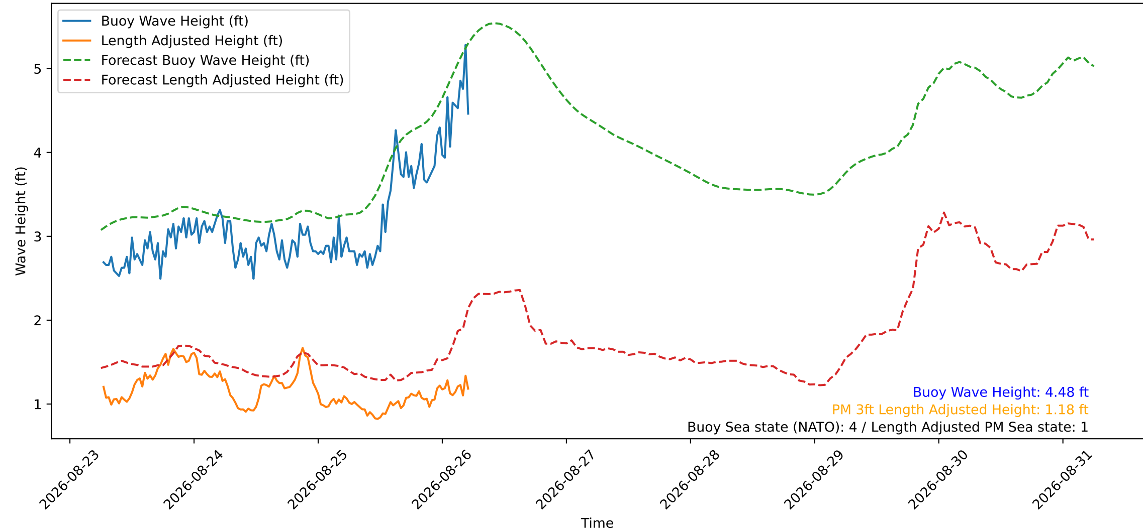
Wave Heights over Time for Green Beach at 2026-08-26 06:01:13
