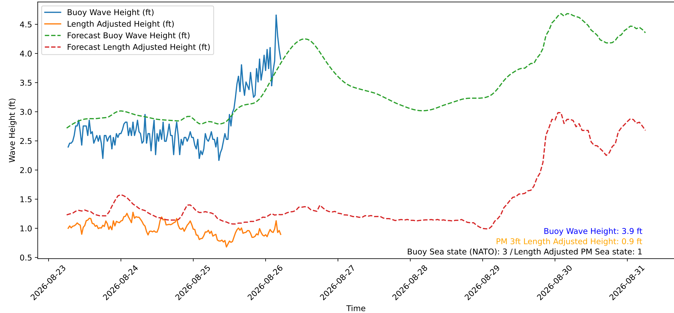
Wave Heights over Time for Red Beach at 2026-08-26 06:00:50
