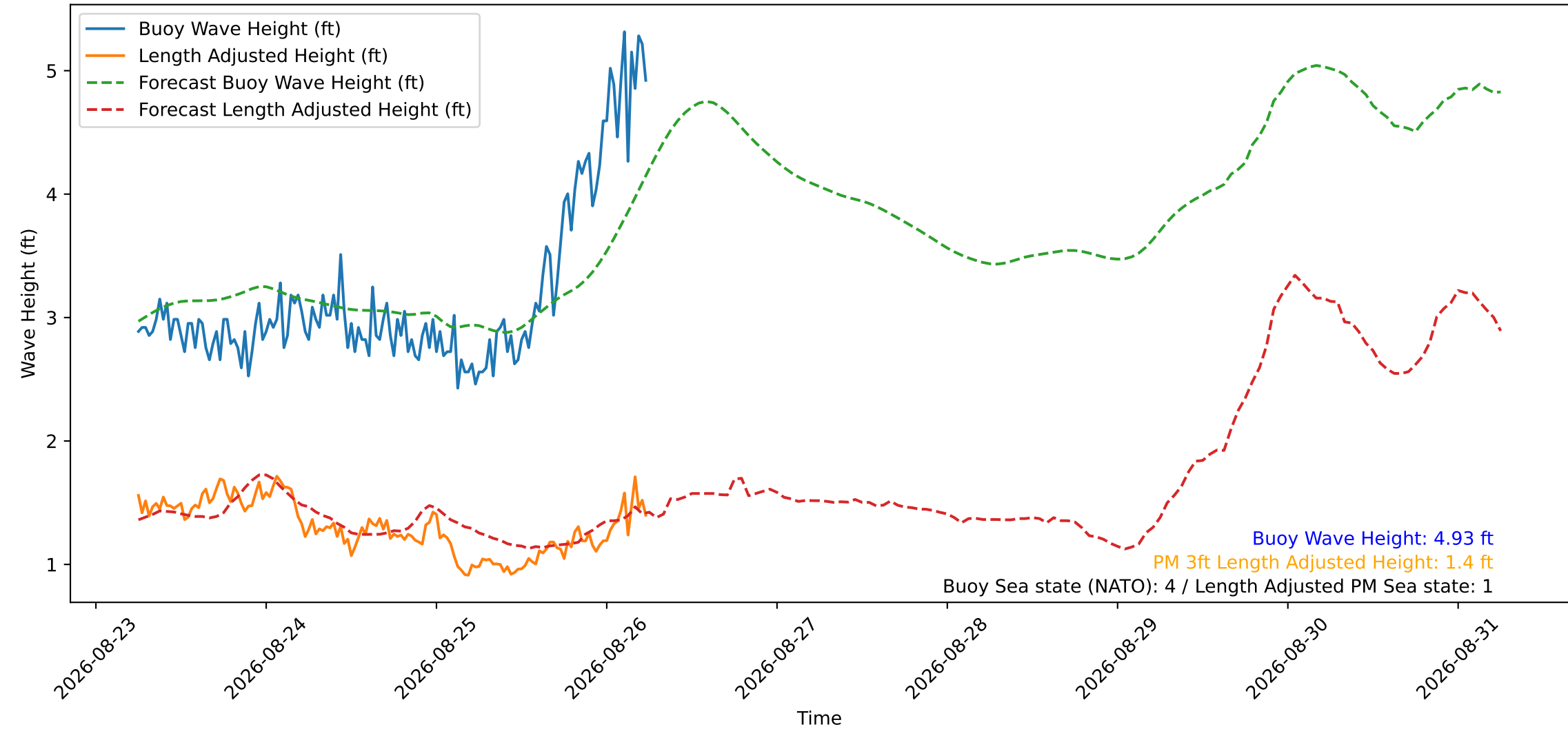
Wave Heights over Time for Oceanside Harbor at 2026-08-26 06:00:30
