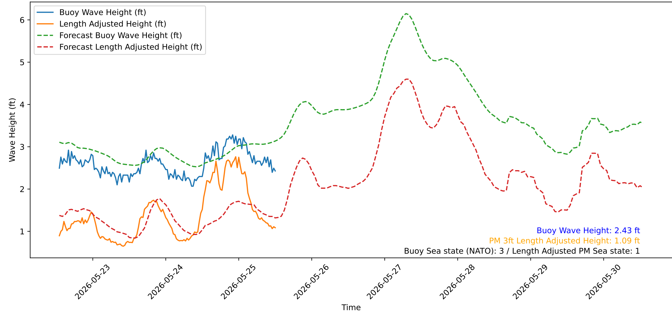
Wave Heights over Time for Green Beach at 2026-05-25 13:11:13
