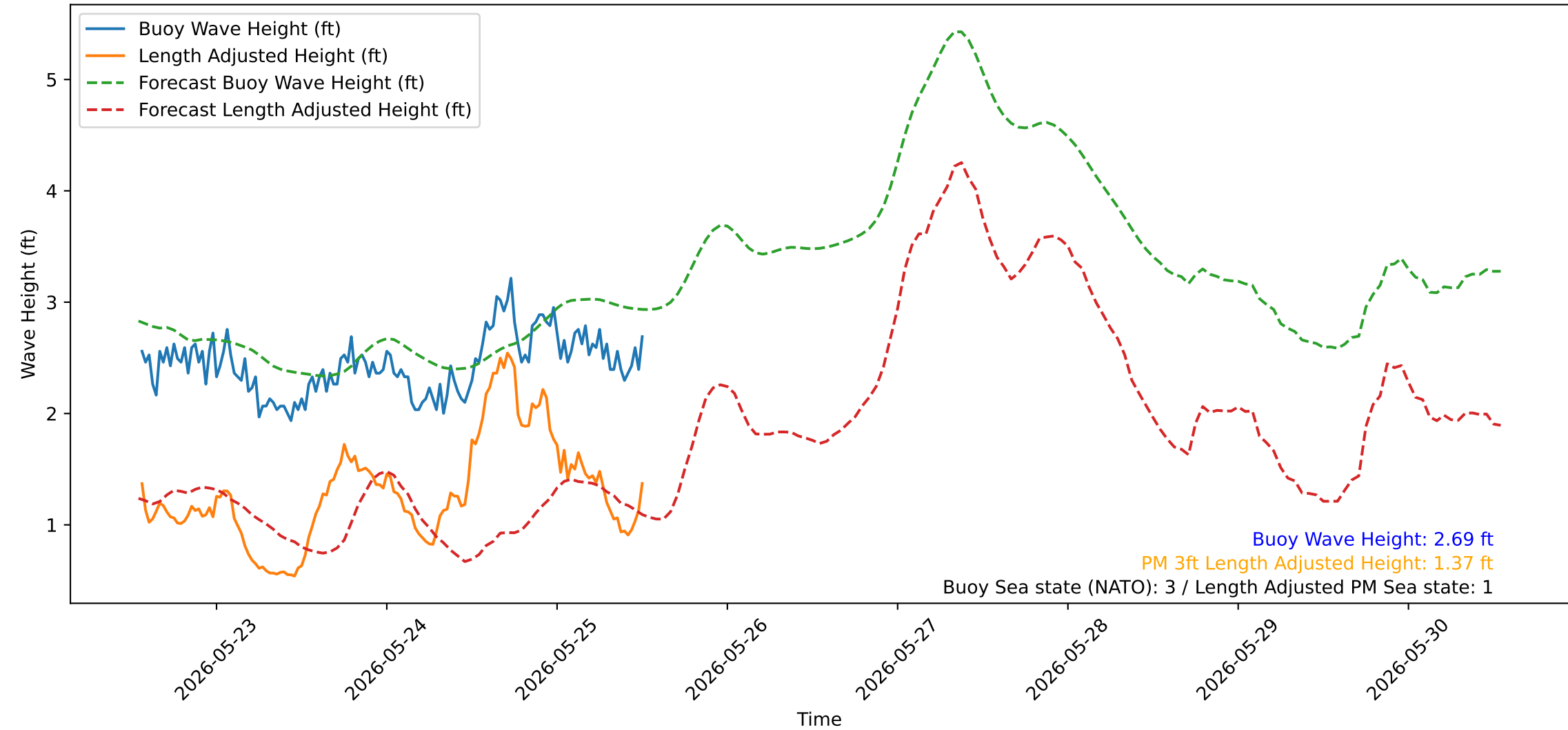
Wave Heights over Time for Red Beach at 2026-05-25 13:10:50
