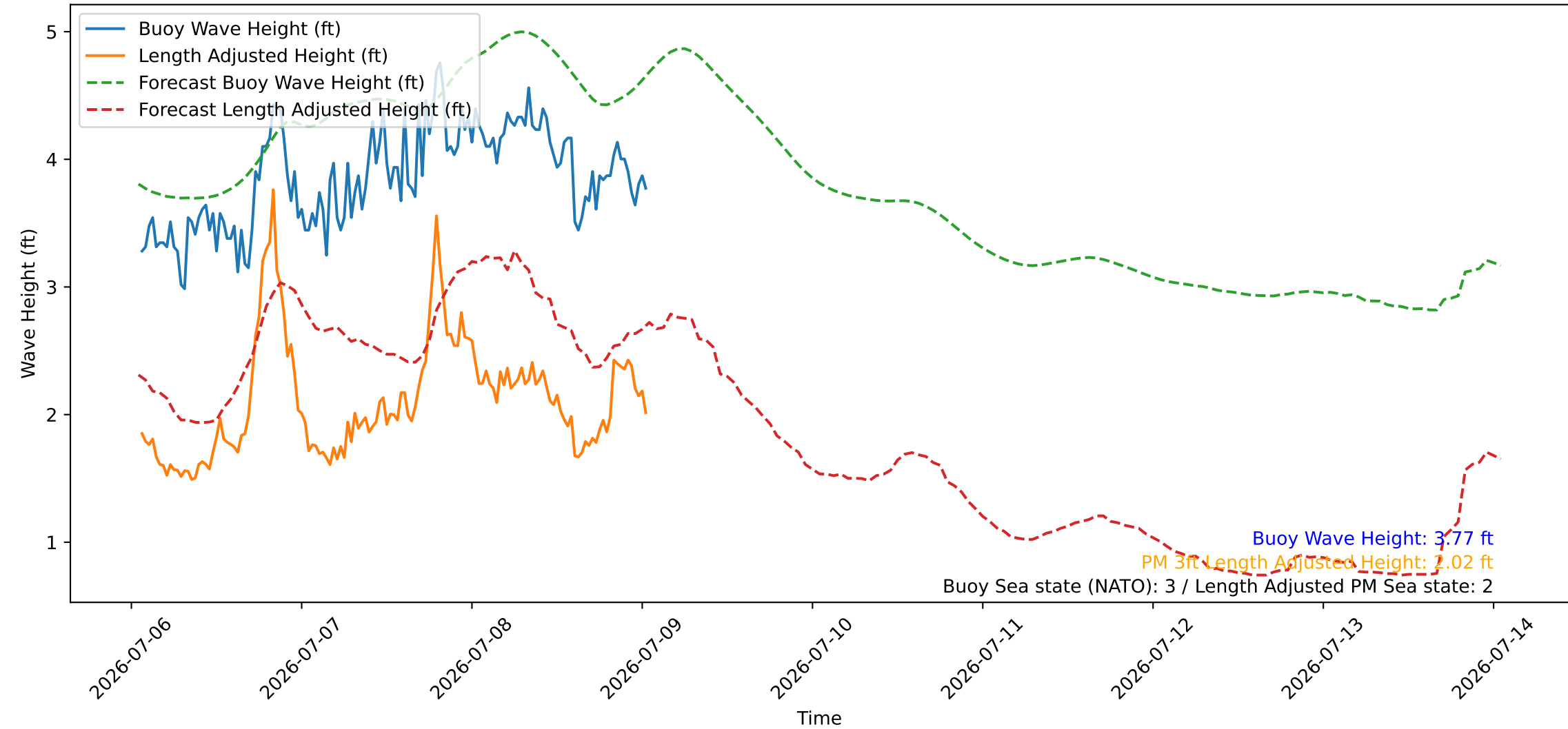
Wave Heights over Time for Green Beach at 2026-07-09 01:21:09
