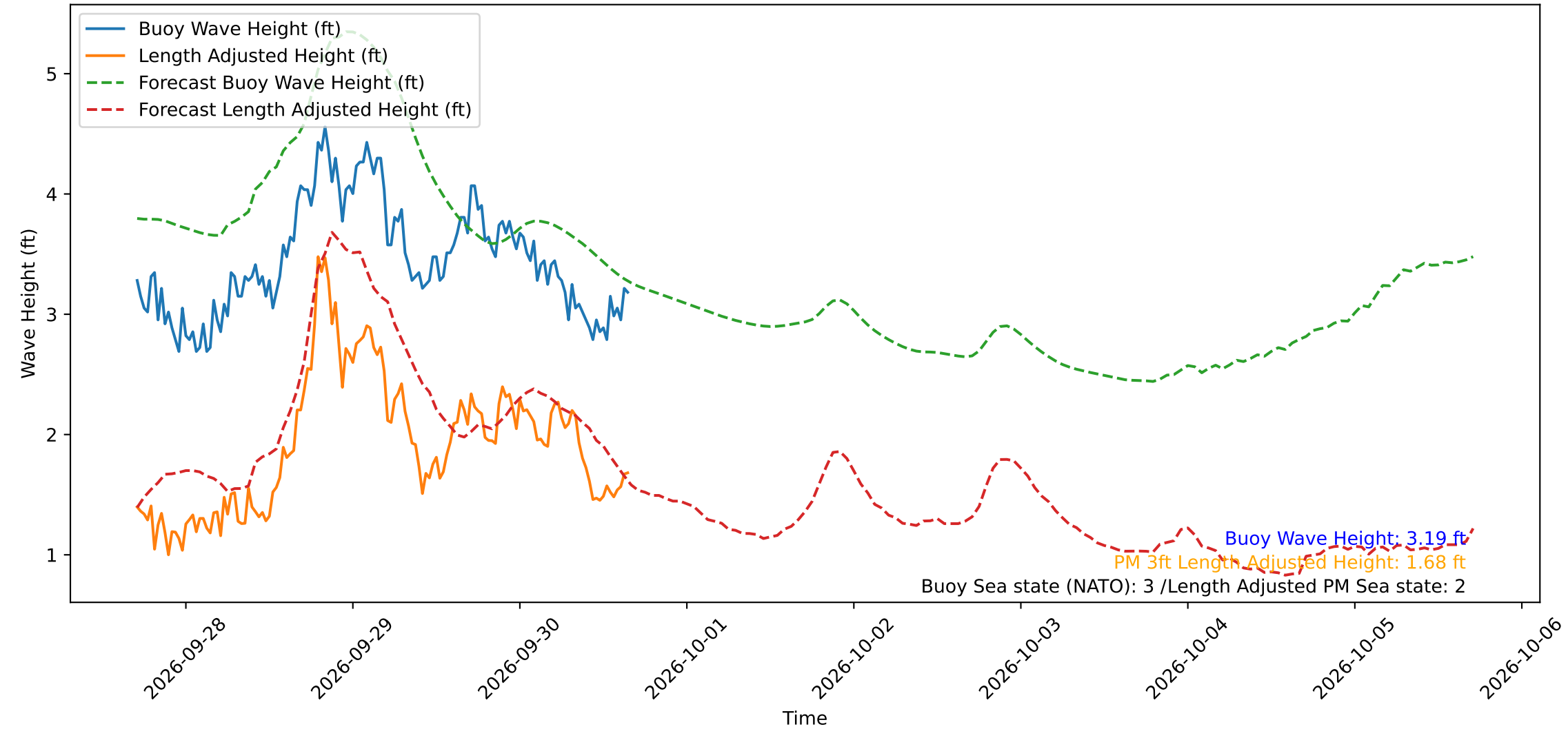
Wave Heights over Time for Green Beach at 2026-09-30 16:31:12
