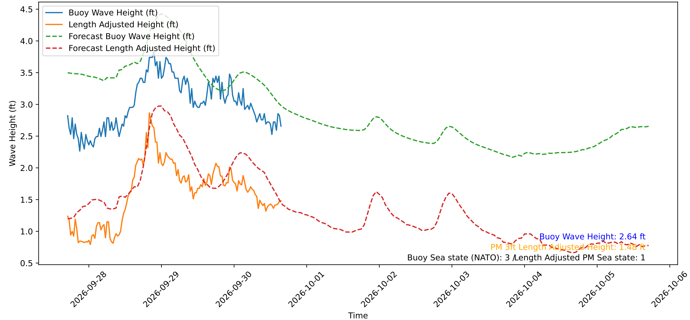
Wave Heights over Time for Red Beach at 2026-09-30 16:30:50
