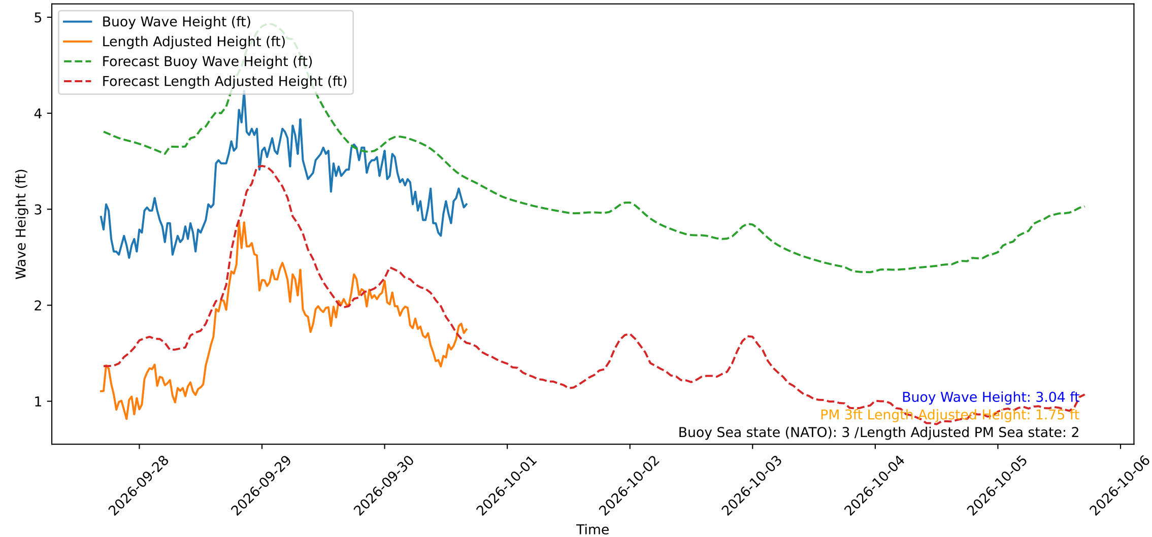
Wave Heights over Time for Oceanside Harbor at 2026-09-30 16:30:30
