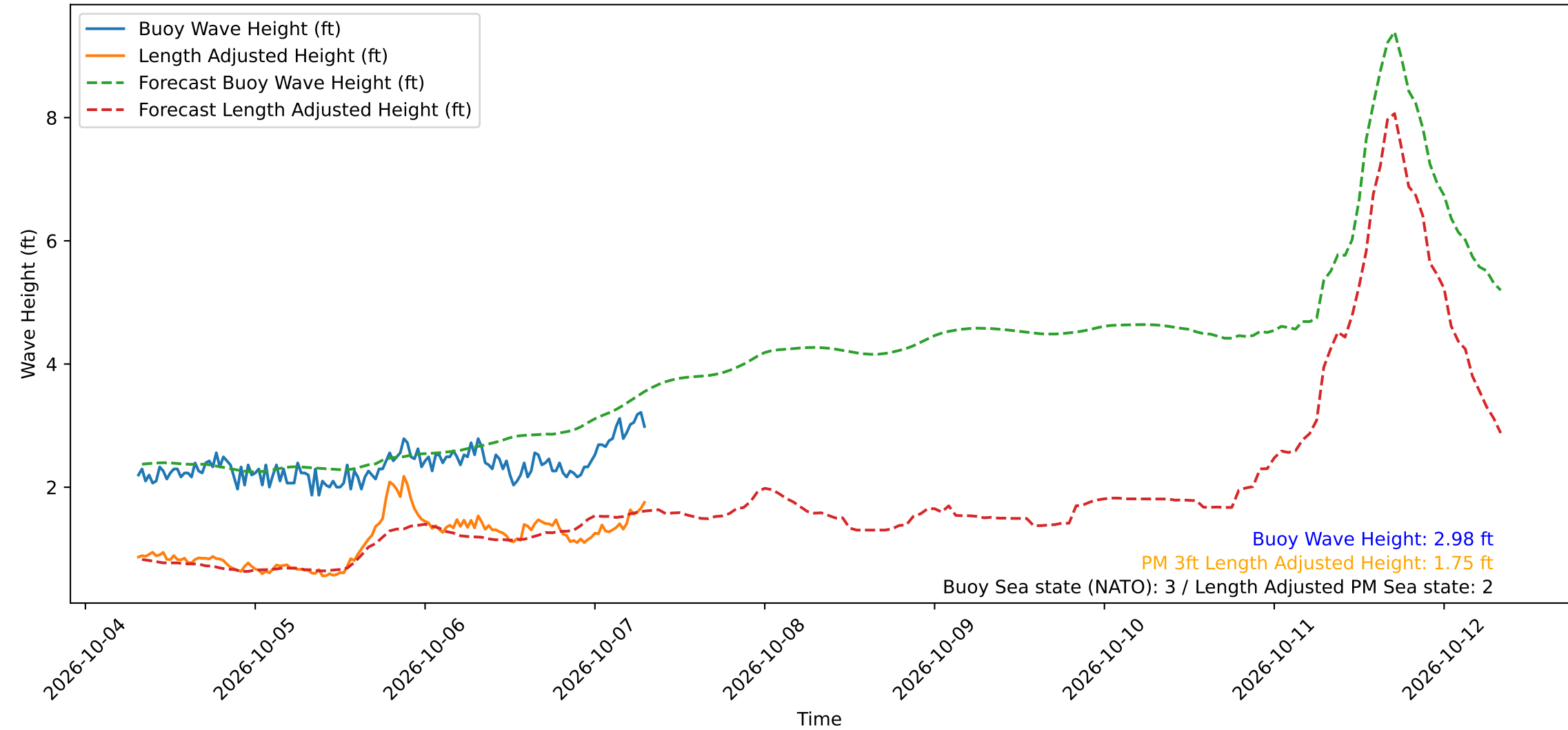
Wave Heights over Time for Oceanside Harbor at 2026-10-07 07:30:30
