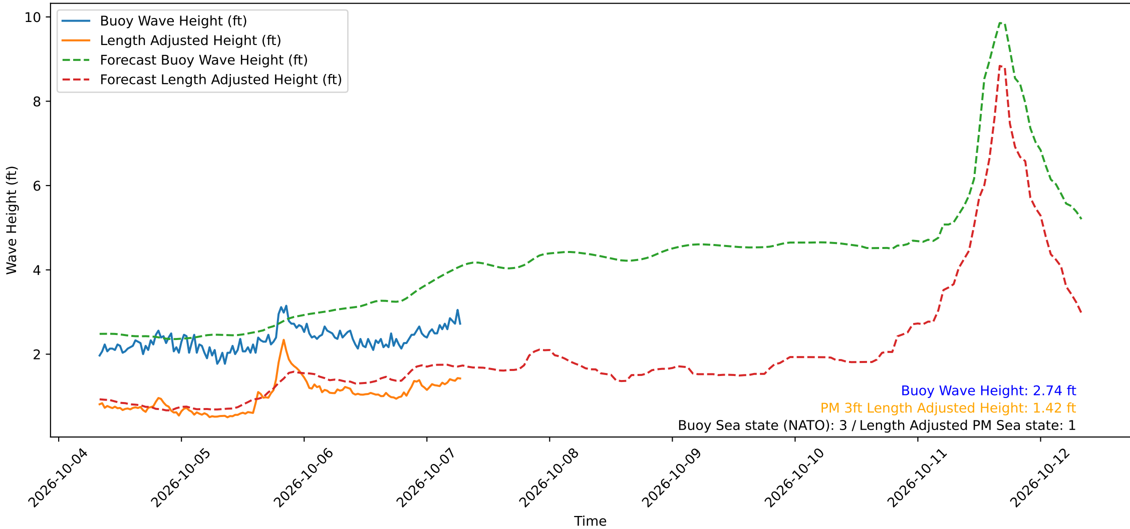
Wave Heights over Time for Green Beach at 2026-10-07 07:31:11
