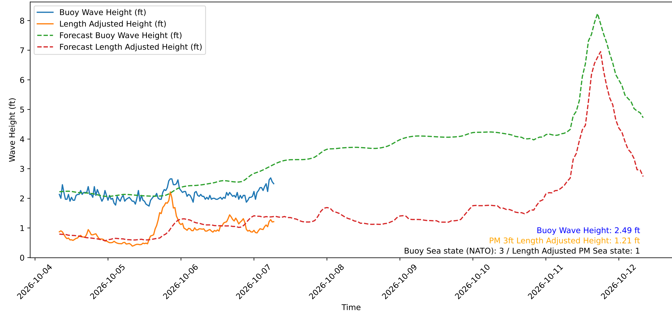
Wave Heights over Time for Red Beach at 2026-10-07 07:30:49
