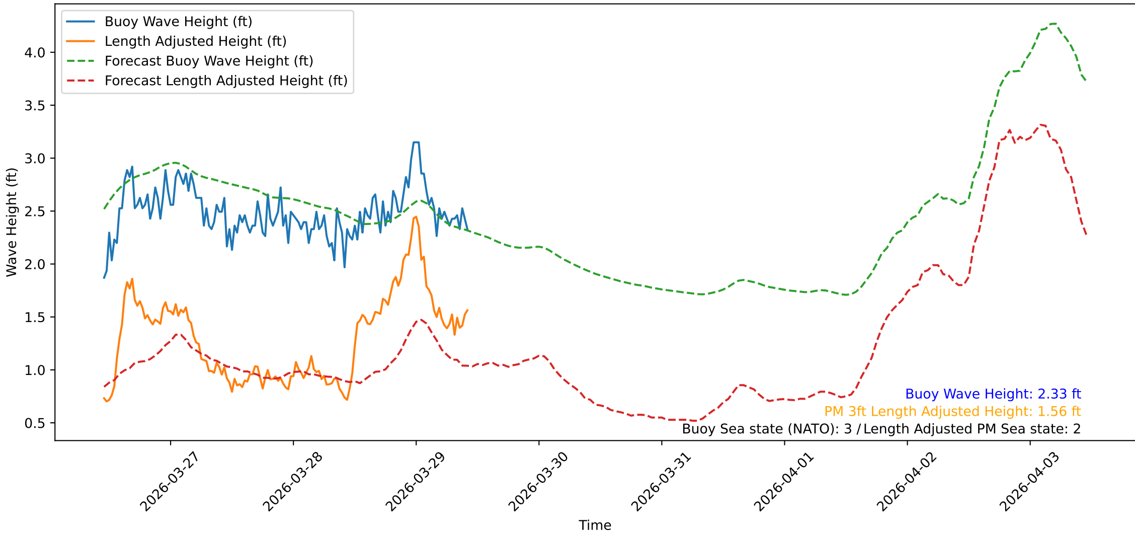
Wave Heights over Time for Oceanside Harbor at 2026-03-29 10:50:32
