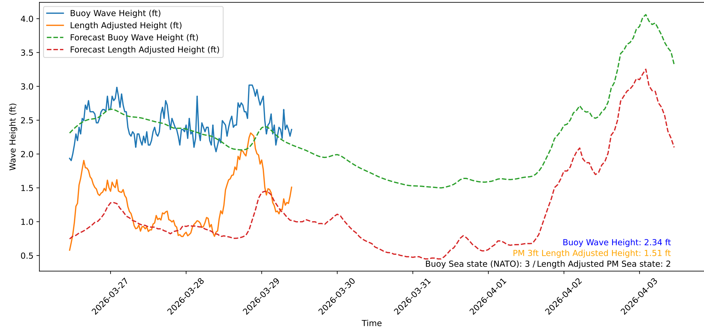
Wave Heights over Time for Red Beach at 2026-03-29 10:50:48
