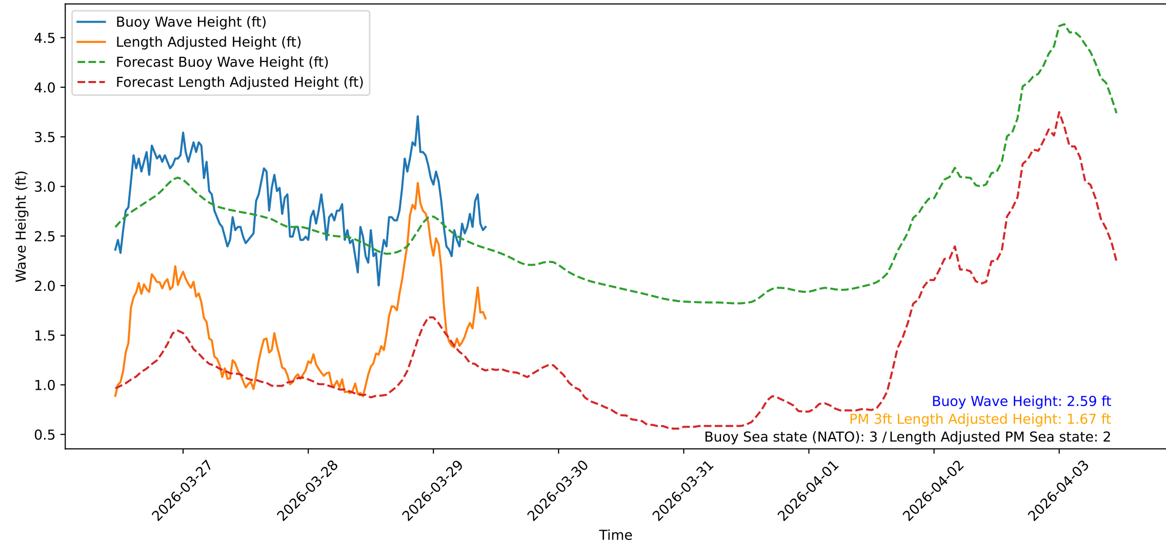
Wave Heights over Time for Green Beach at 2026-03-29 10:51:10
