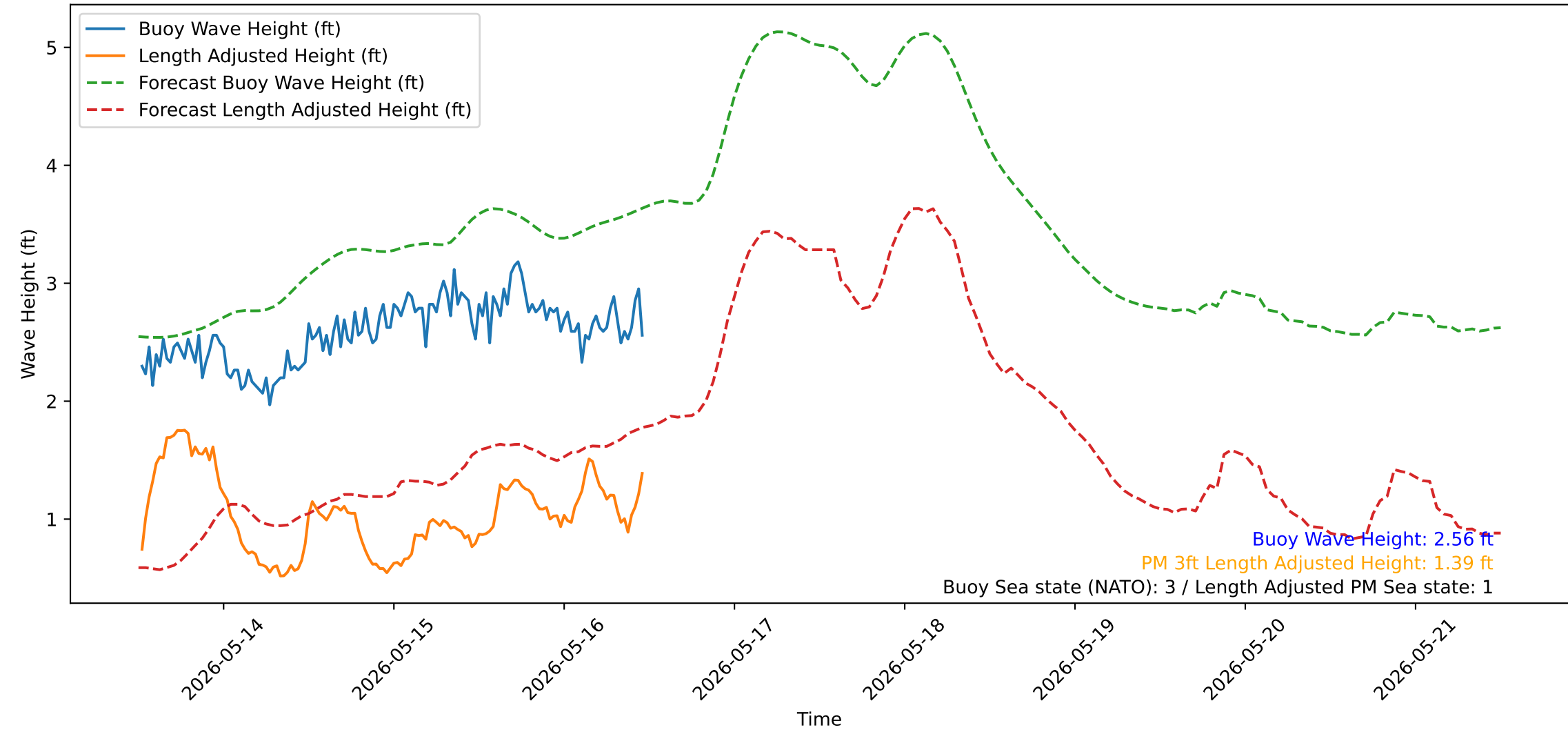
Wave Heights over Time for Red Beach at 2026-05-16 12:00:50
