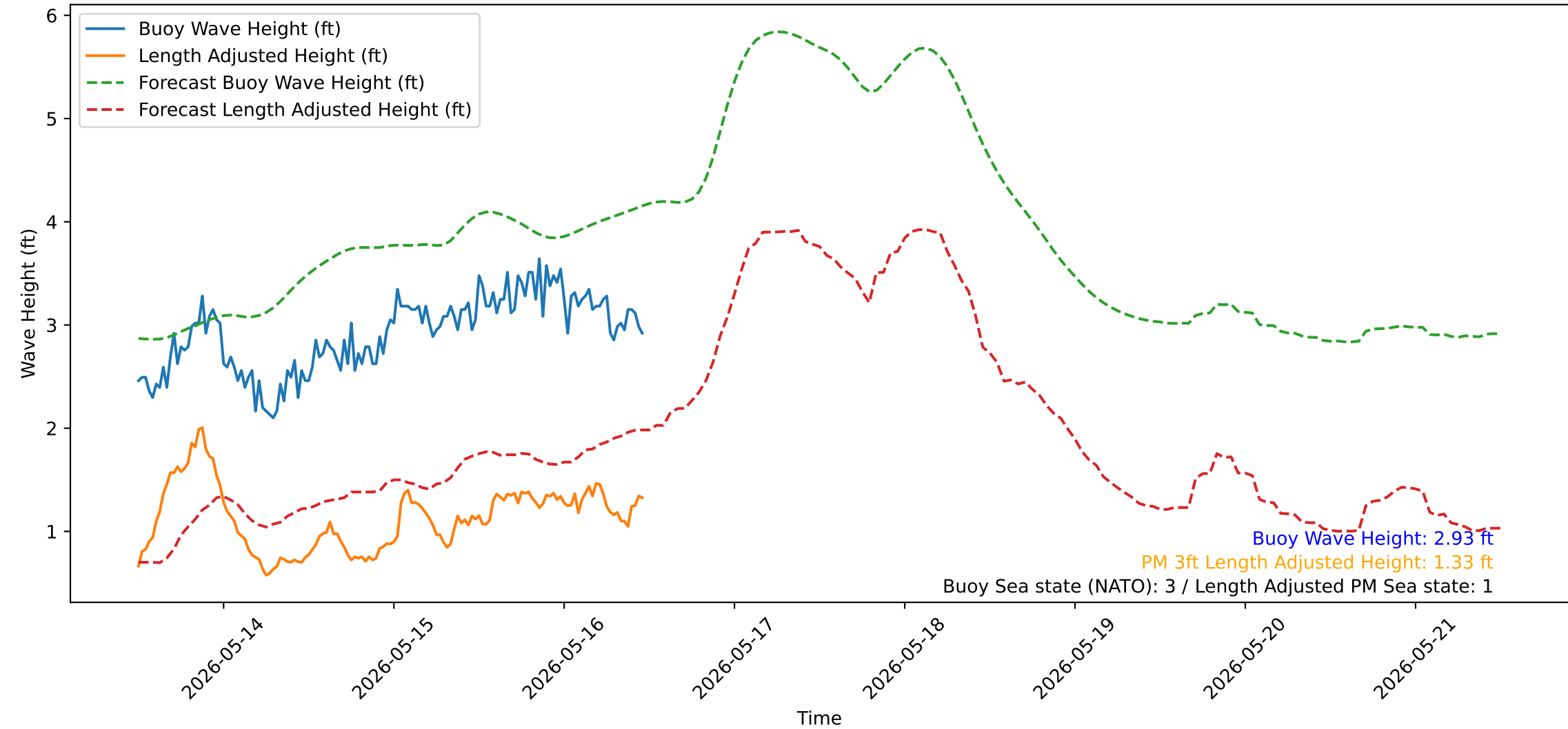
Wave Heights over Time for Green Beach at 2026-05-16 12:01:13
