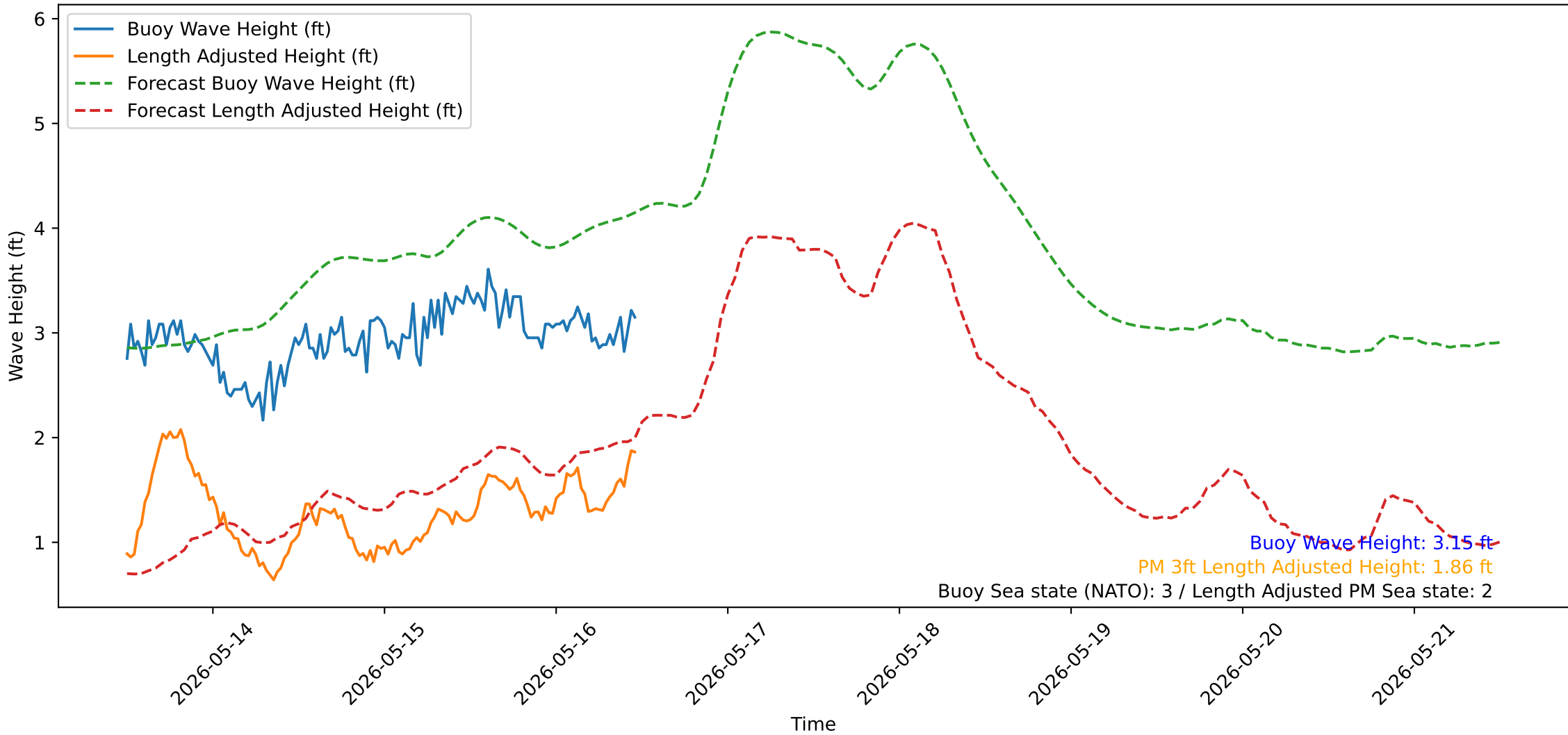
Wave Heights over Time for Oceanside Harbor at 2026-05-16 12:00:31
