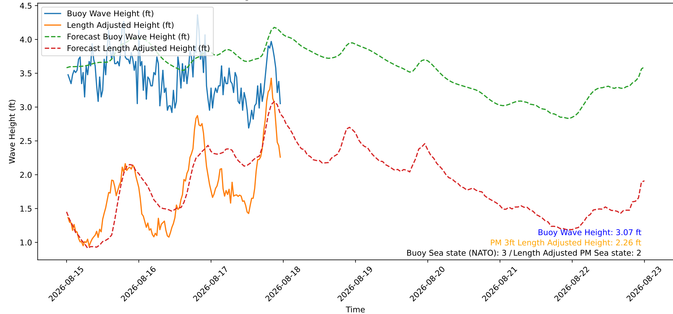
Wave Heights over Time for Green Beach at 2026-08-18 00:01:08
