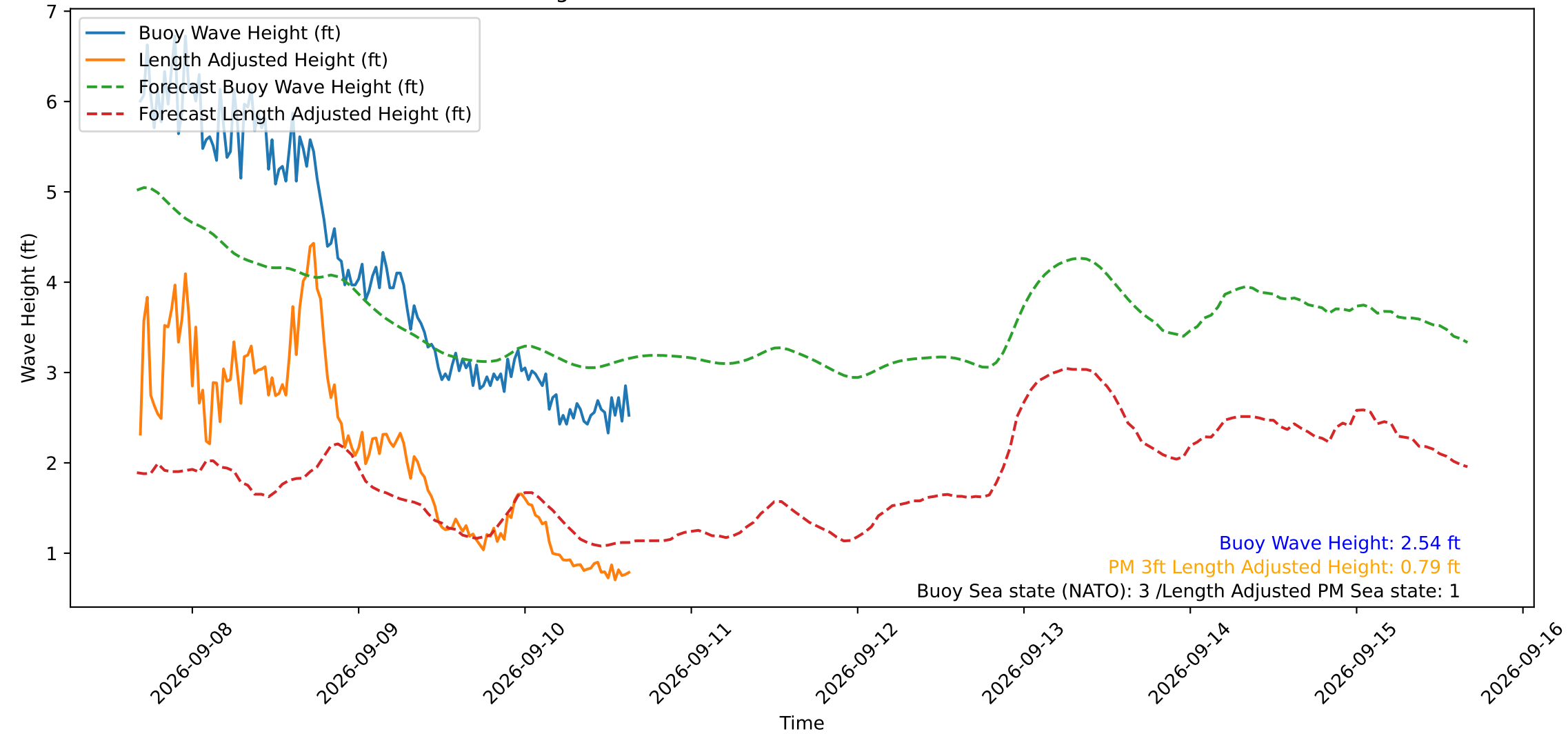
Wave Heights over Time for Red Beach at 2026-09-10 16:10:50
