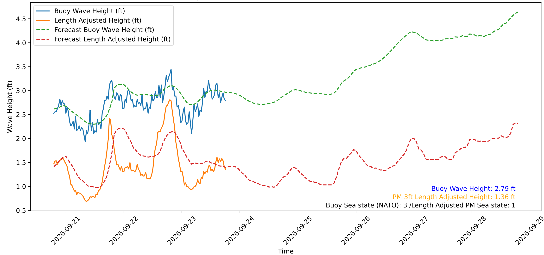
Wave Heights over Time for Green Beach at 2026-09-23 18:41:11
