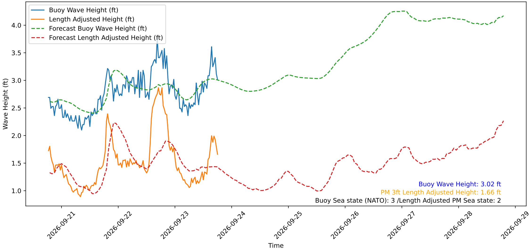
Wave Heights over Time for Oceanside Harbor at 2026-09-23 18:40:29
