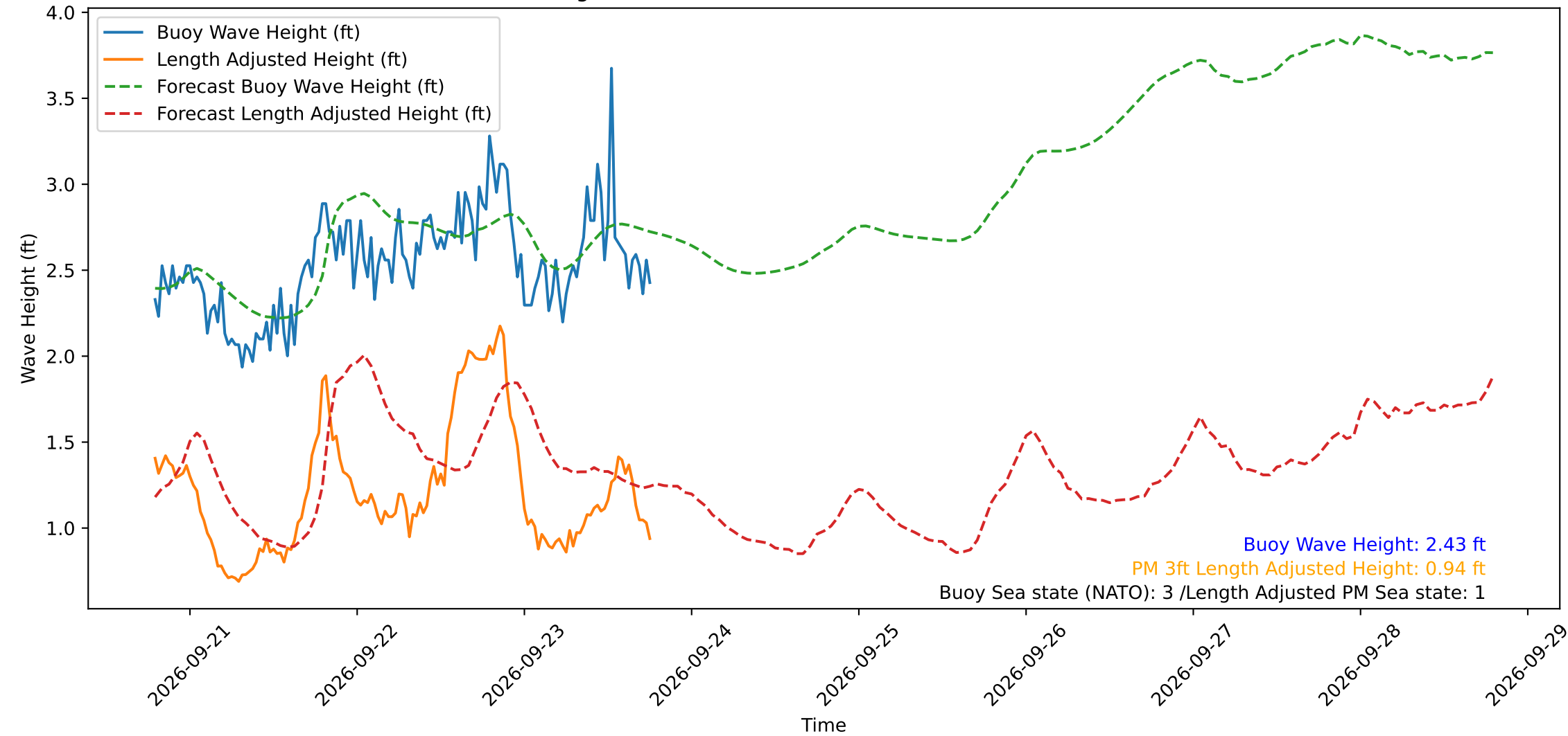
Wave Heights over Time for Red Beach at 2026-09-23 18:40:49
