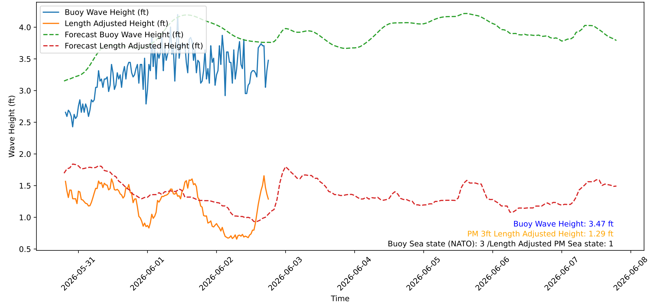
Wave Heights over Time for Red Beach at 2026-06-02 19:00:45
