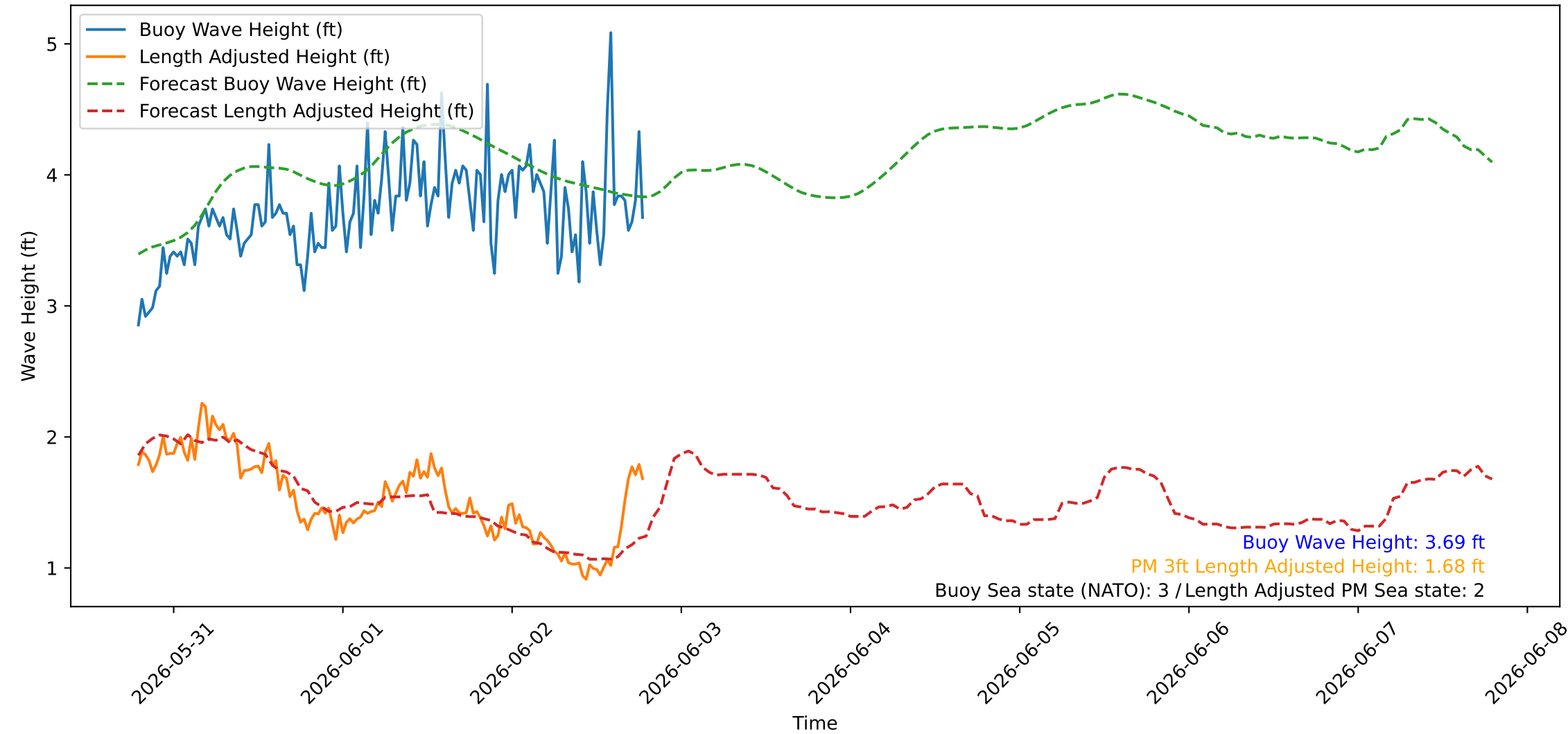
Wave Heights over Time for Oceanside Harbor at 2026-06-02 19:00:26
