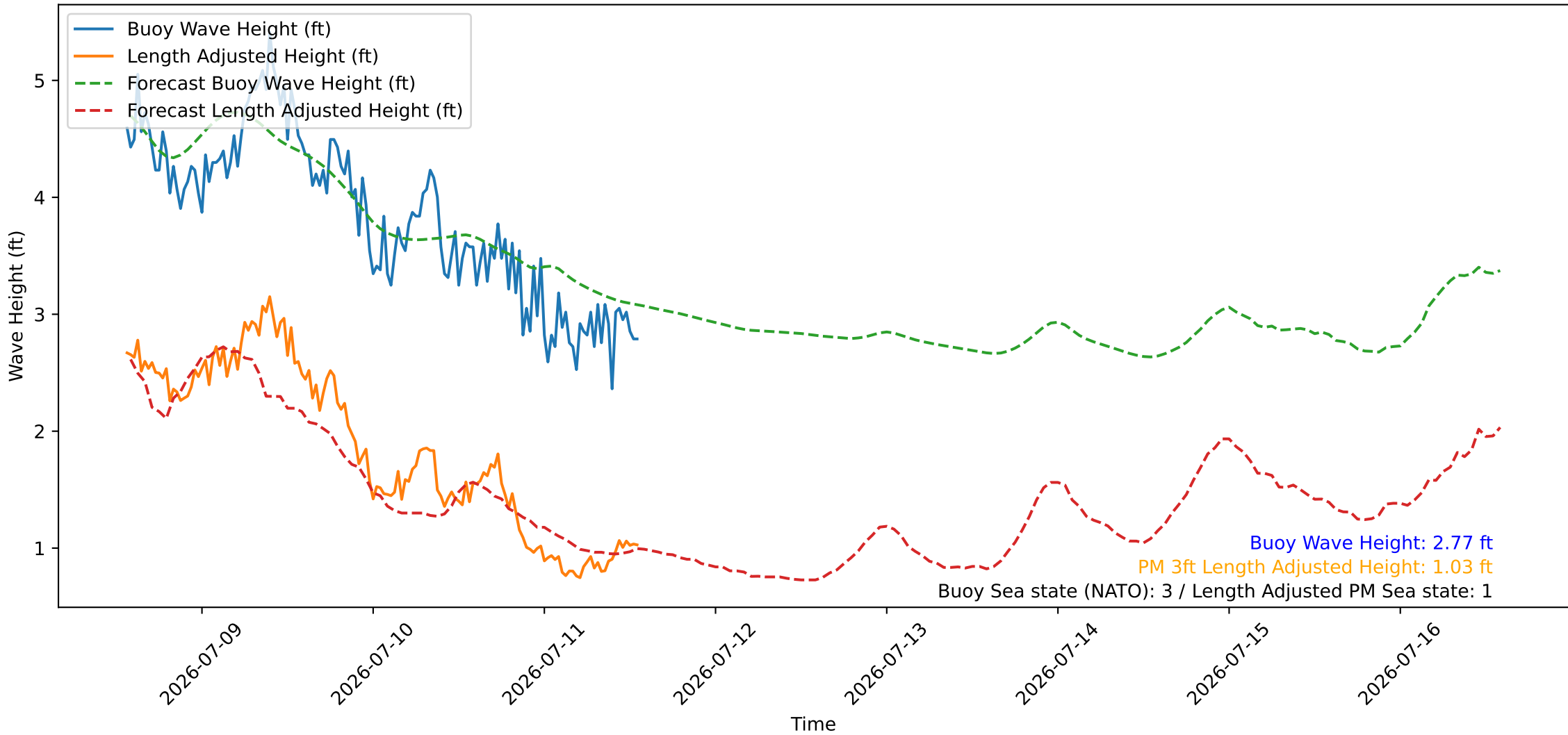
Wave Heights over Time for Oceanside Harbor at 2026-07-11 13:40:26
