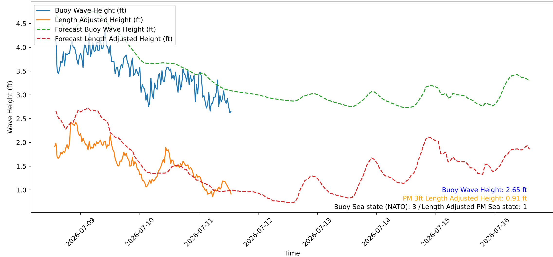
Wave Heights over Time for Green Beach at 2026-07-11 13:41:08
