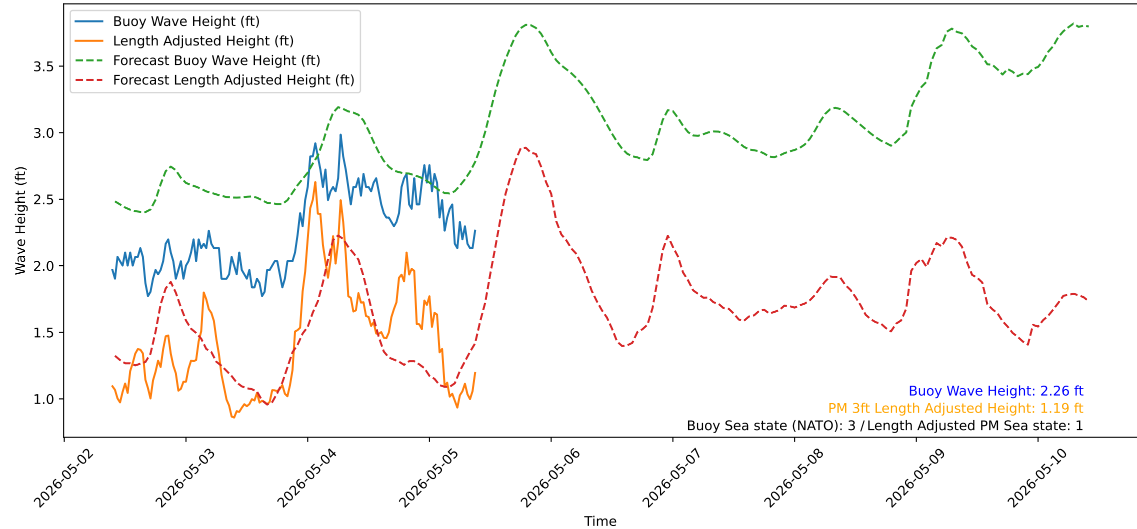
Wave Heights over Time for Green Beach at 2026-05-05 09:41:14
