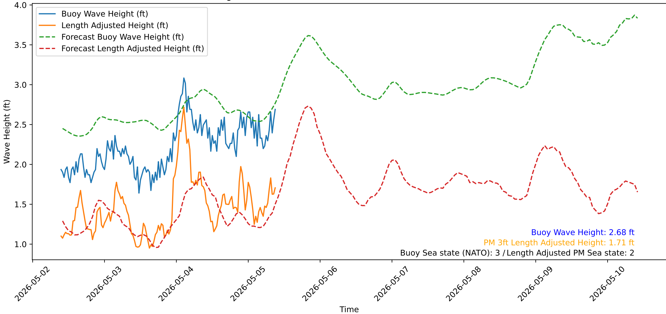
Wave Heights over Time for Oceanside Harbor at 2026-05-05 09:40:32
