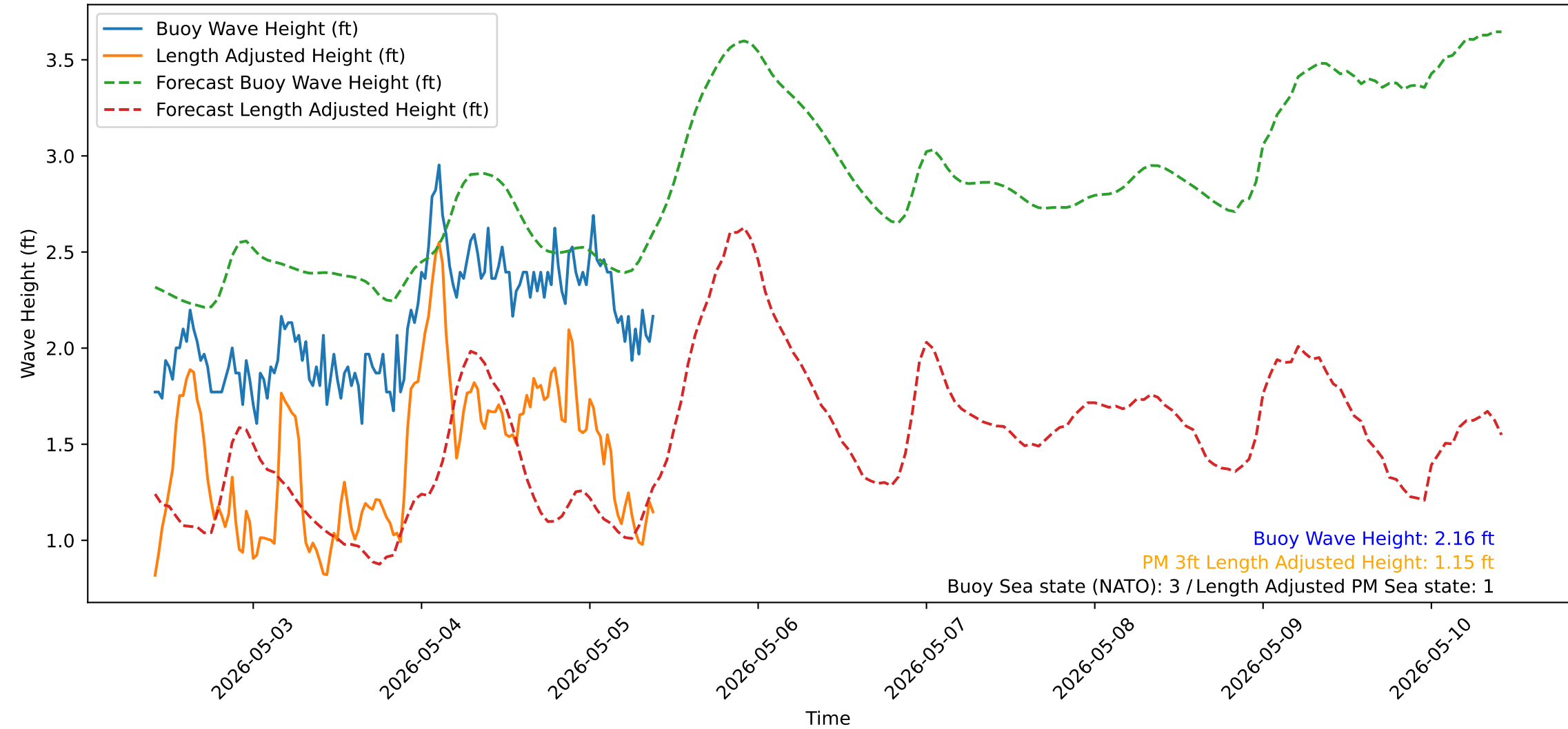
Wave Heights over Time for Red Beach at 2026-05-05 09:40:51
