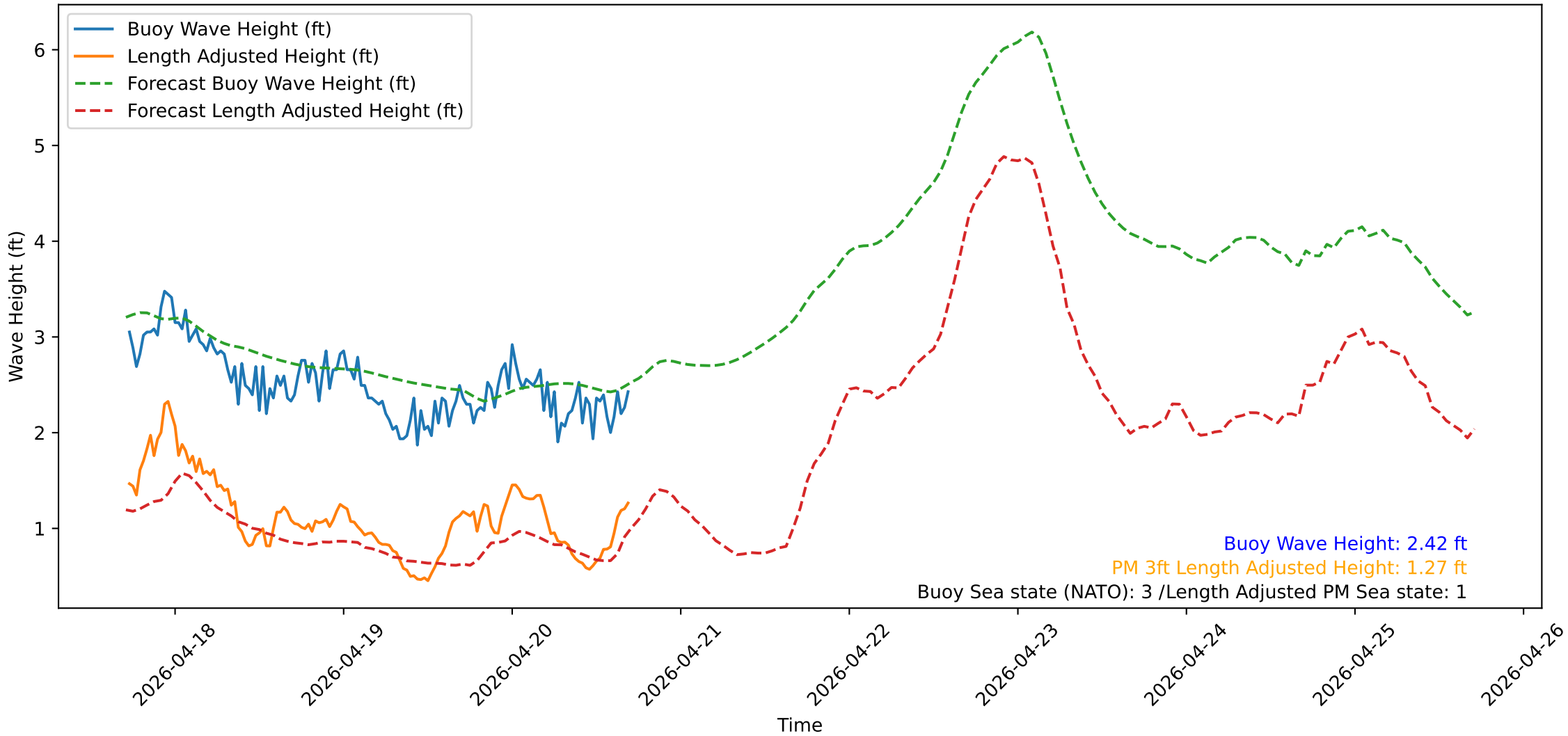
Wave Heights over Time for Green Beach at 2026-04-20 17:21:14
