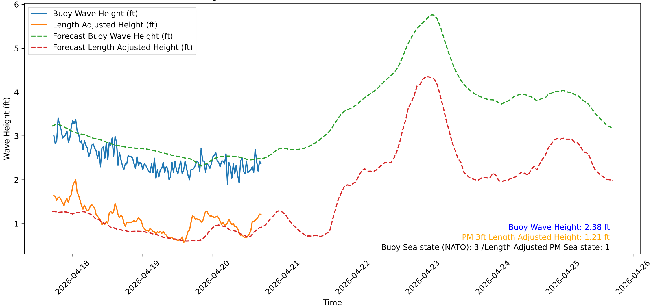
Wave Heights over Time for Oceanside Harbor at 2026-04-20 17:20:31
