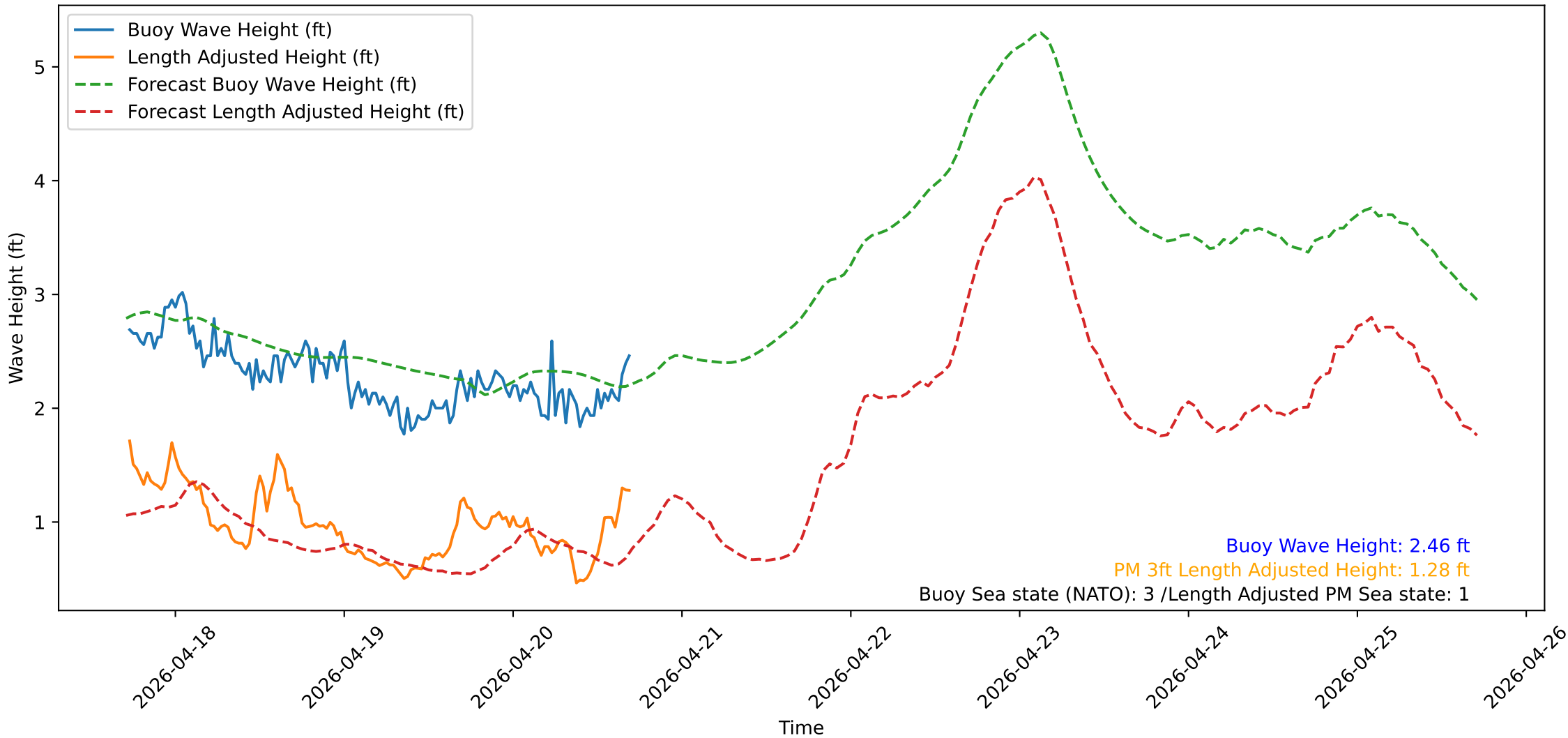
Wave Heights over Time for Red Beach at 2026-04-20 17:20:51
