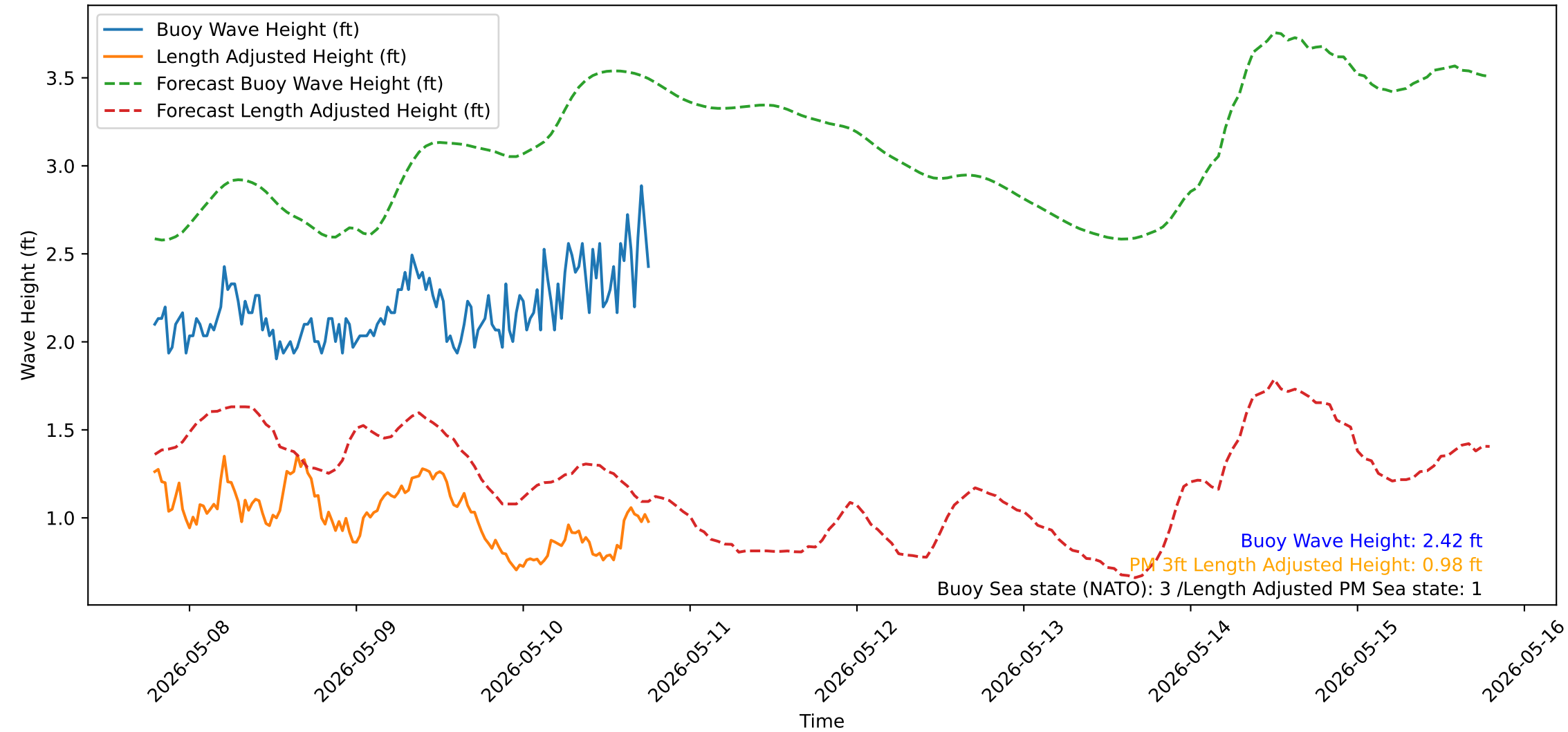
Wave Heights over Time for Red Beach at 2026-05-10 18:40:50
