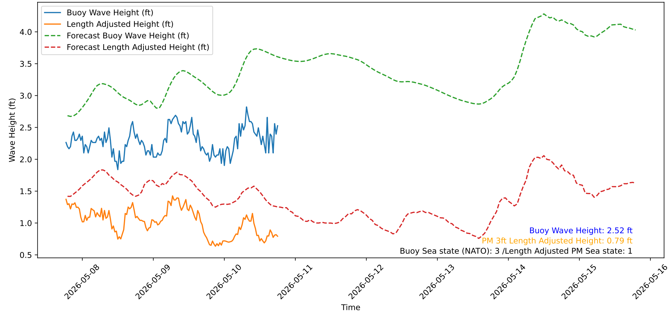
Wave Heights over Time for Green Beach at 2026-05-10 18:41:13
