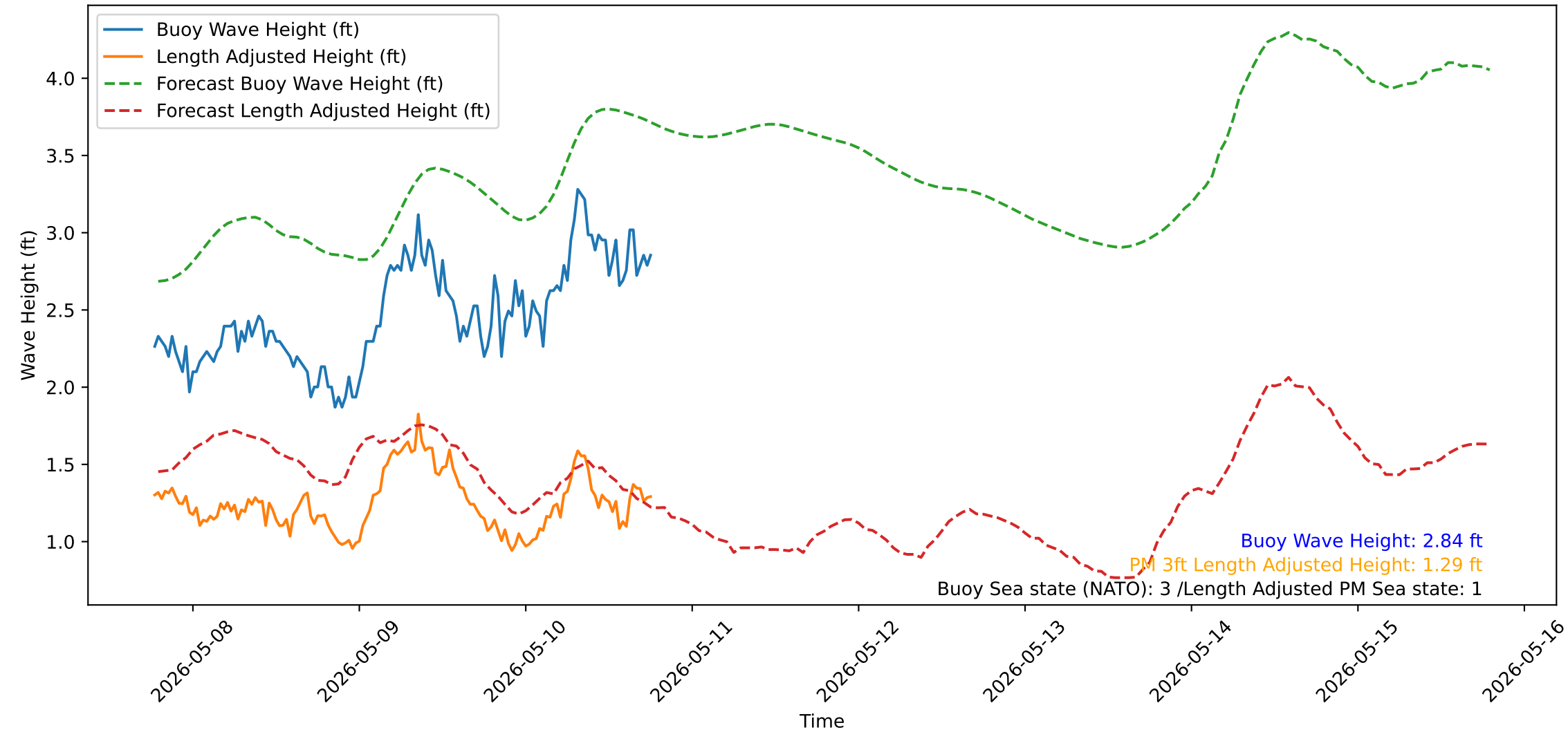
Wave Heights over Time for Oceanside Harbor at 2026-05-10 18:40:31
