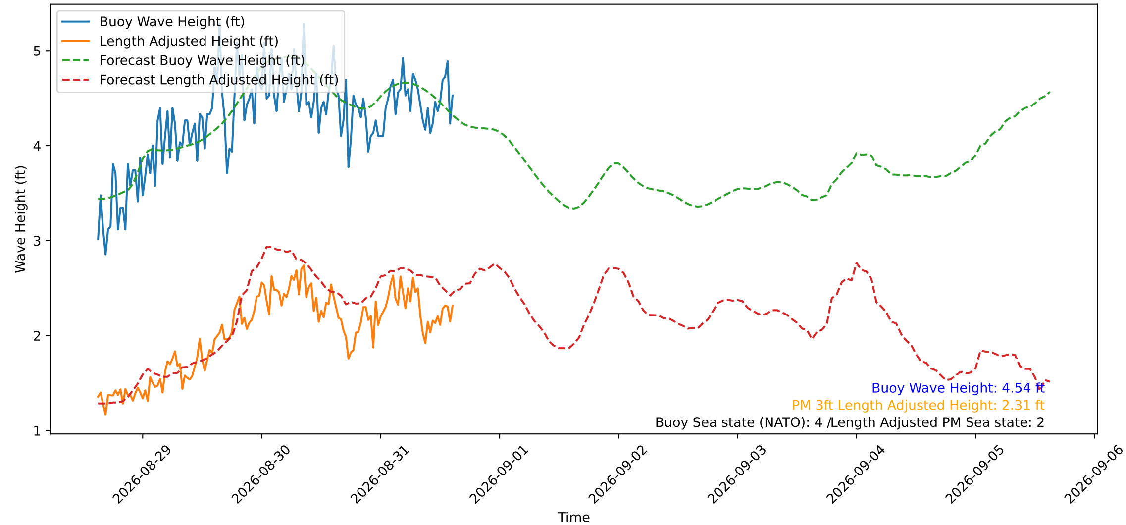
Wave Heights over Time for Oceanside Harbor at 2026-08-31 15:10:30
