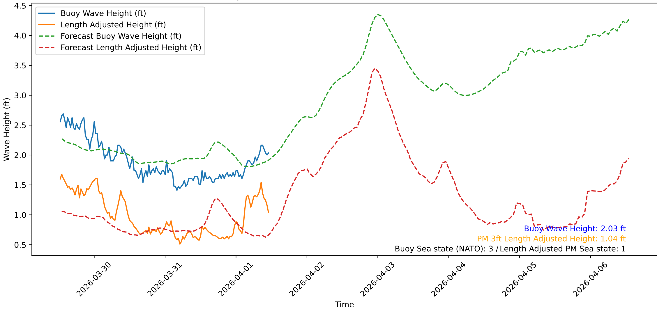
Wave Heights over Time for Green Beach at 2026-04-01 12:31:09
