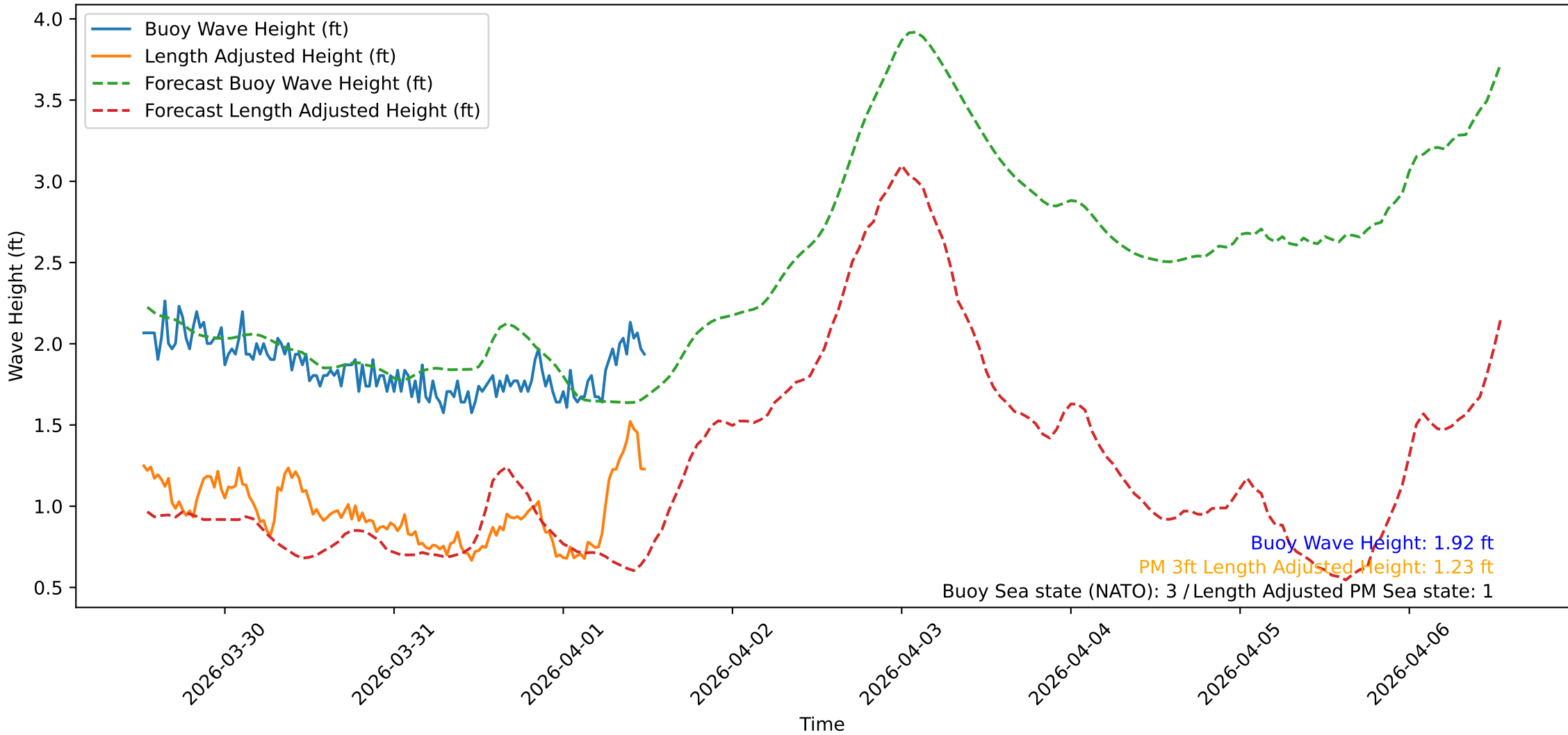
Wave Heights over Time for Oceanside Harbor at 2026-04-01 12:30:31
