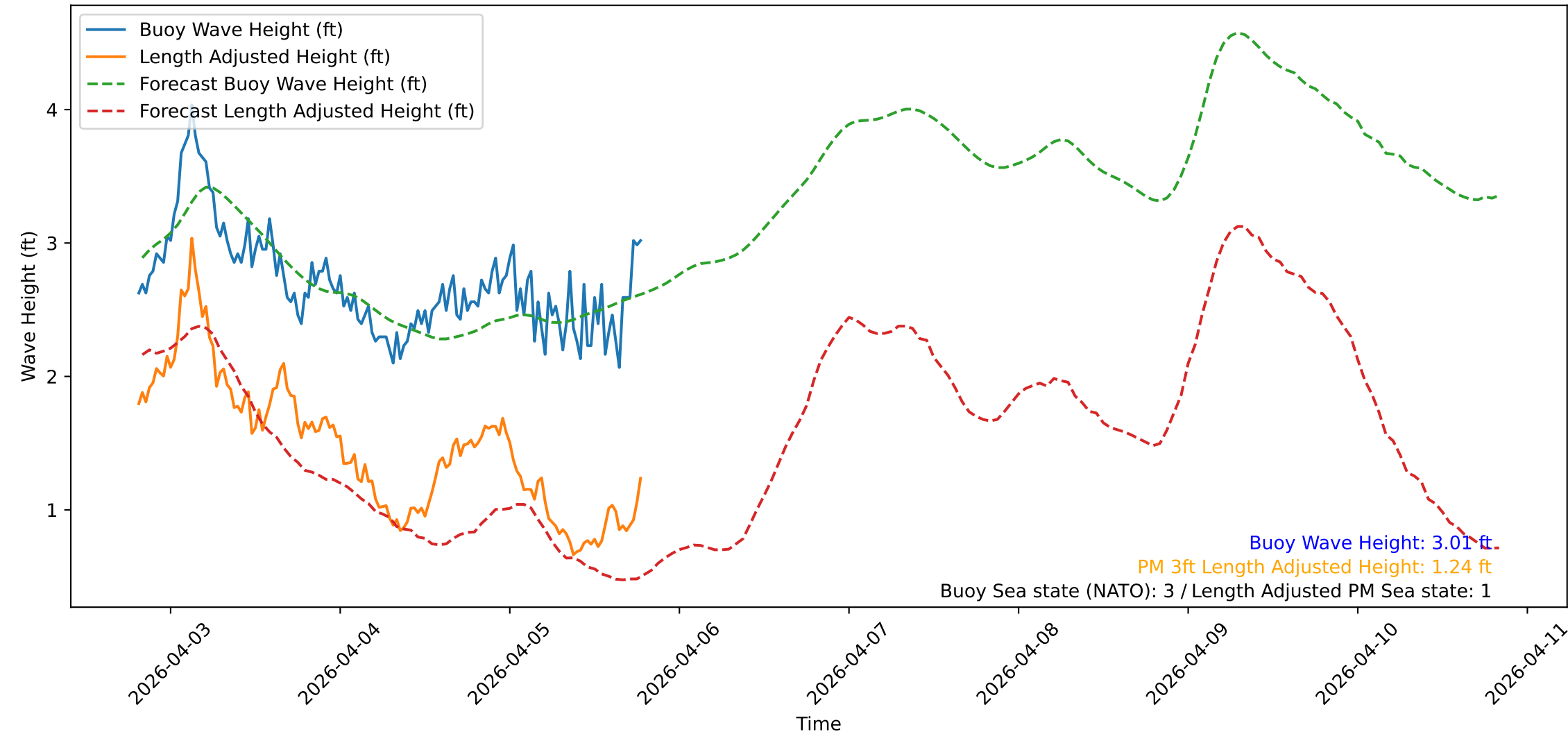
Wave Heights over Time for Oceanside Harbor at 2026-04-05 19:40:33
