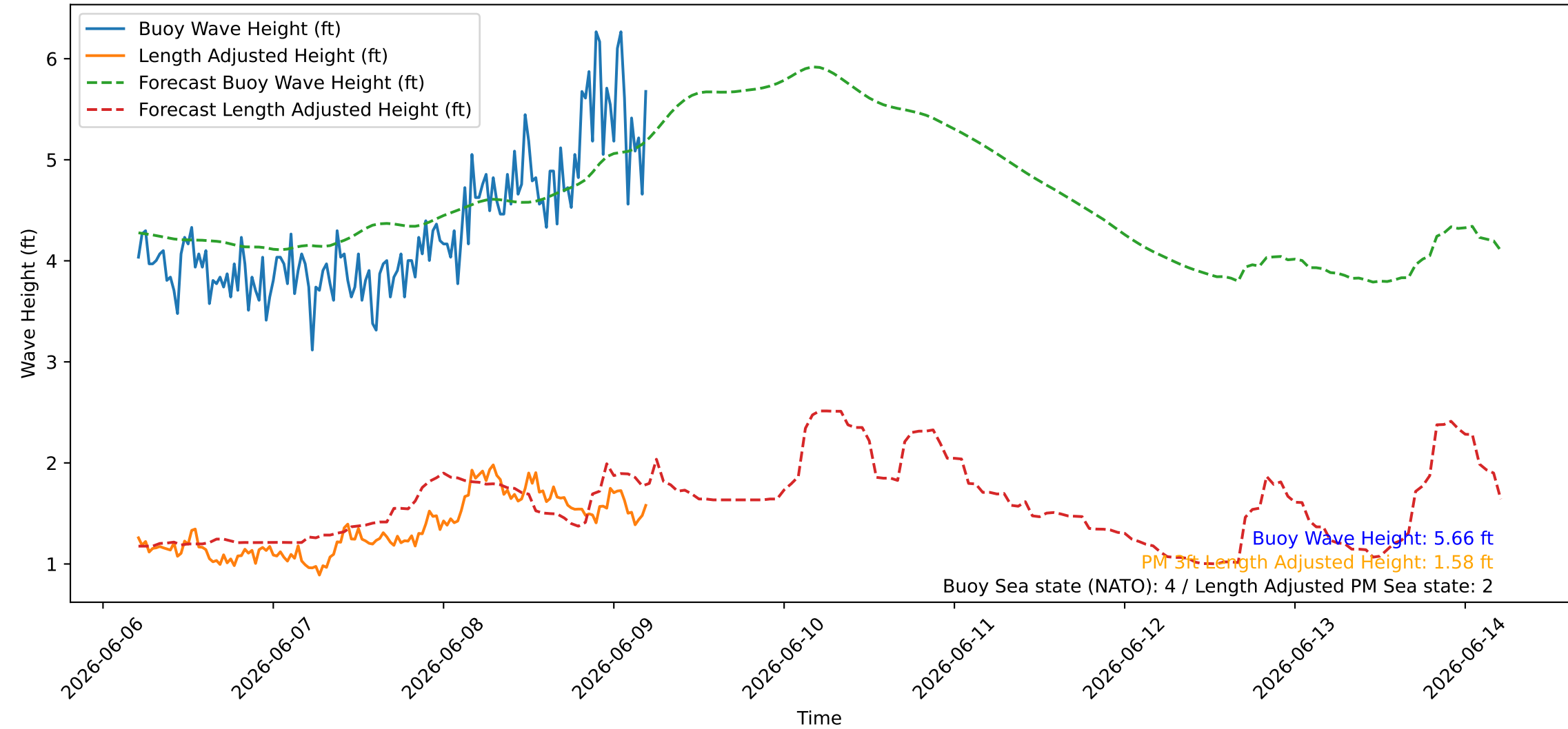
Wave Heights over Time for Green Beach at 2026-06-09 05:11:08
