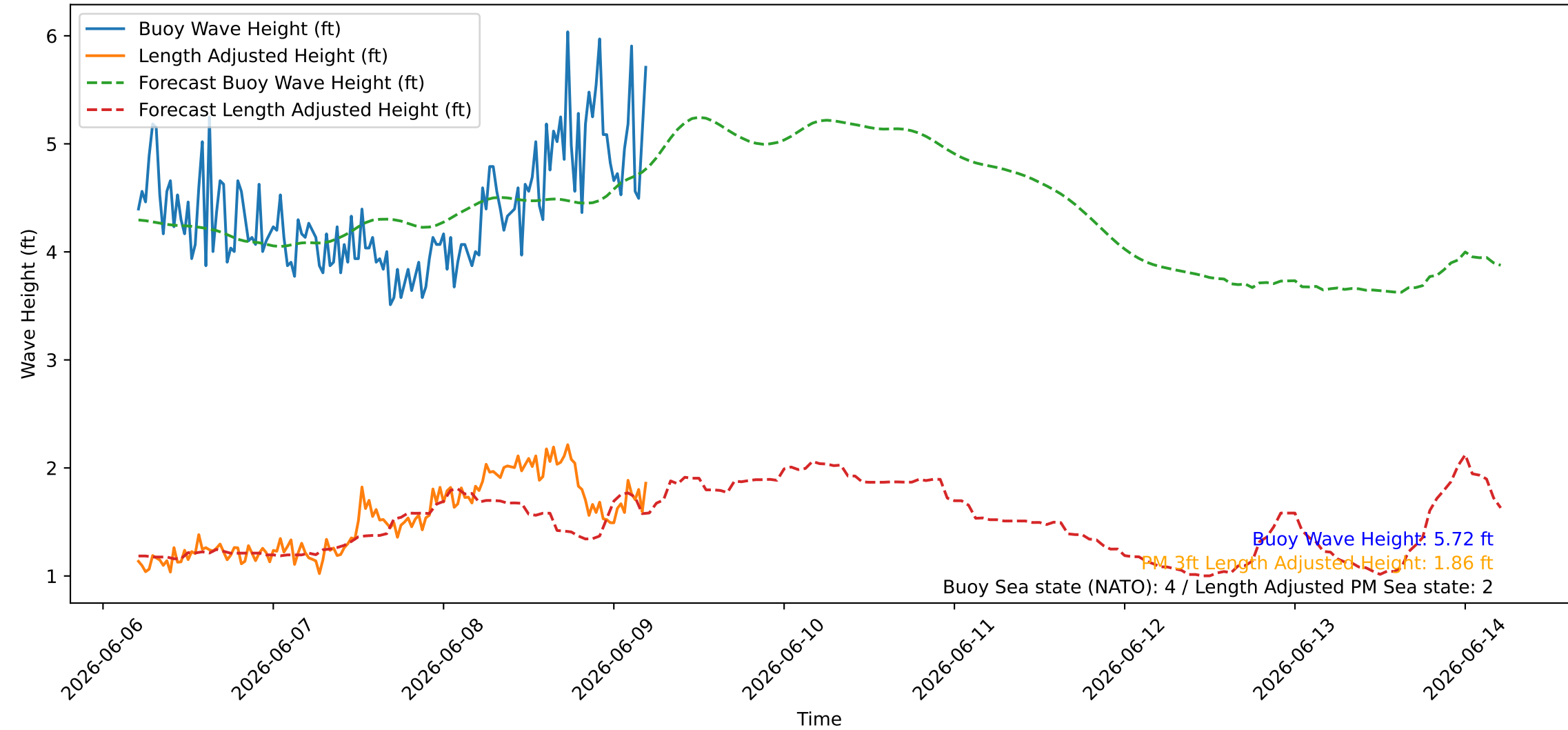
Wave Heights over Time for Oceanside Harbor at 2026-06-09 05:10:26
