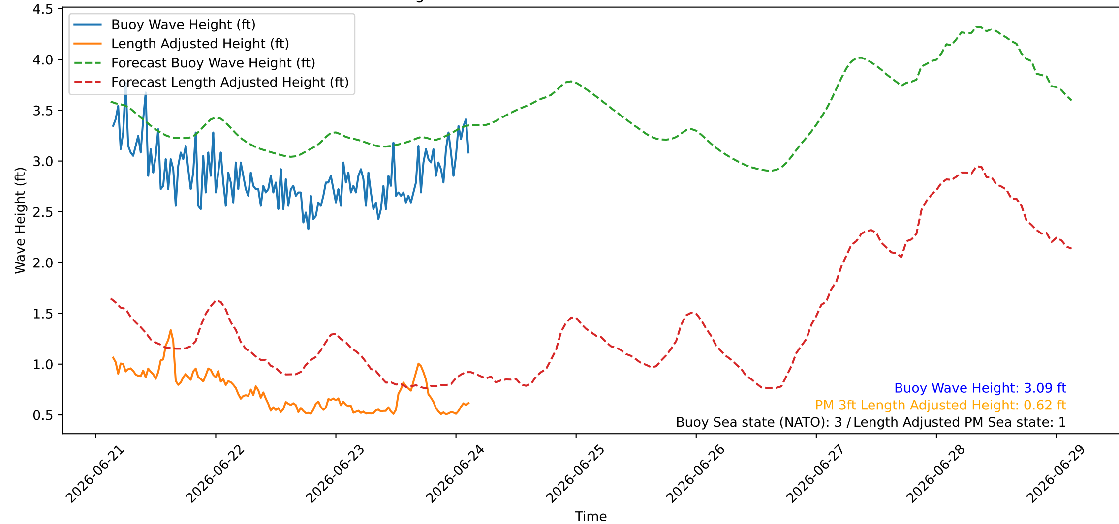
Wave Heights over Time for Red Beach at 2026-06-24 03:20:46
