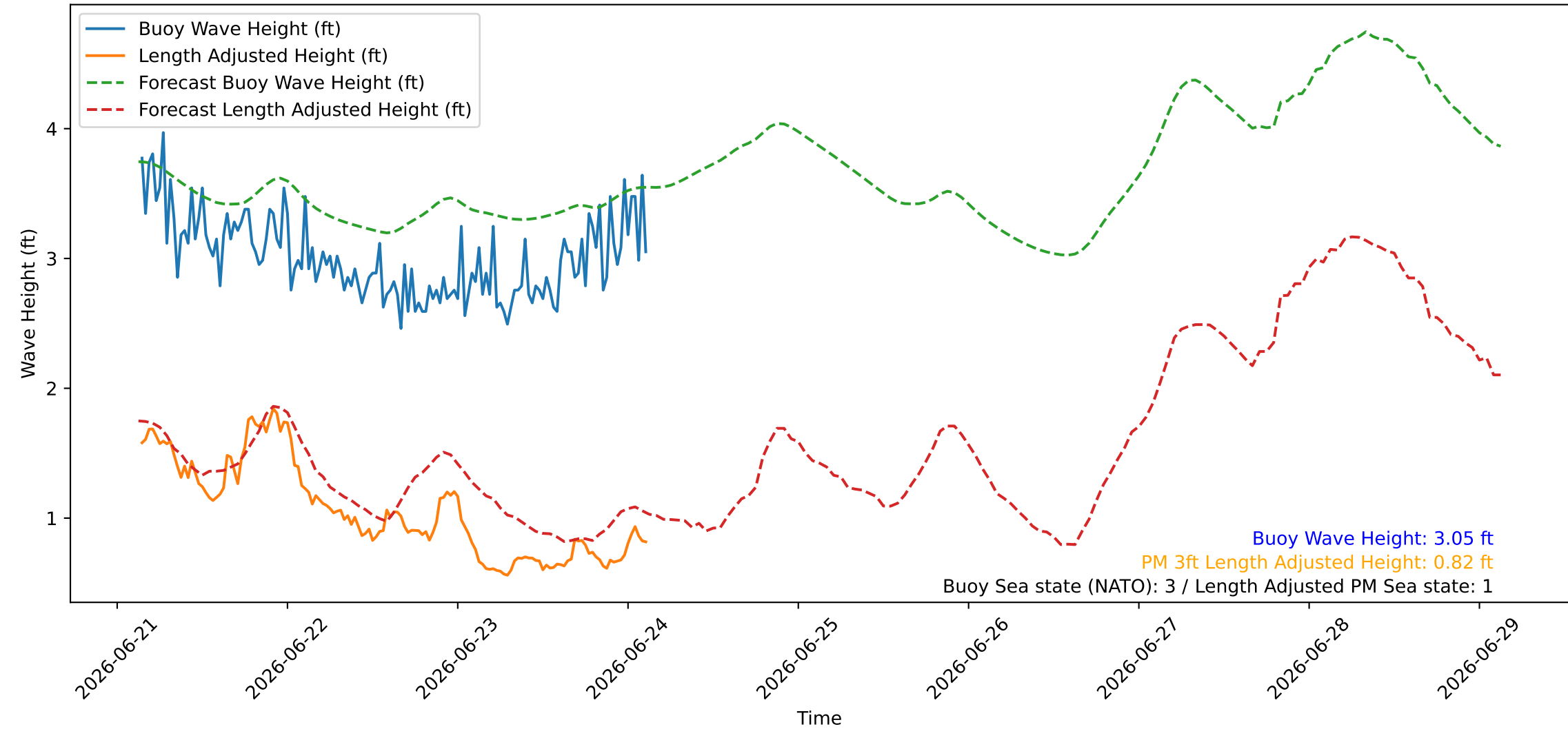
Wave Heights over Time for Green Beach at 2026-06-24 03:21:08
