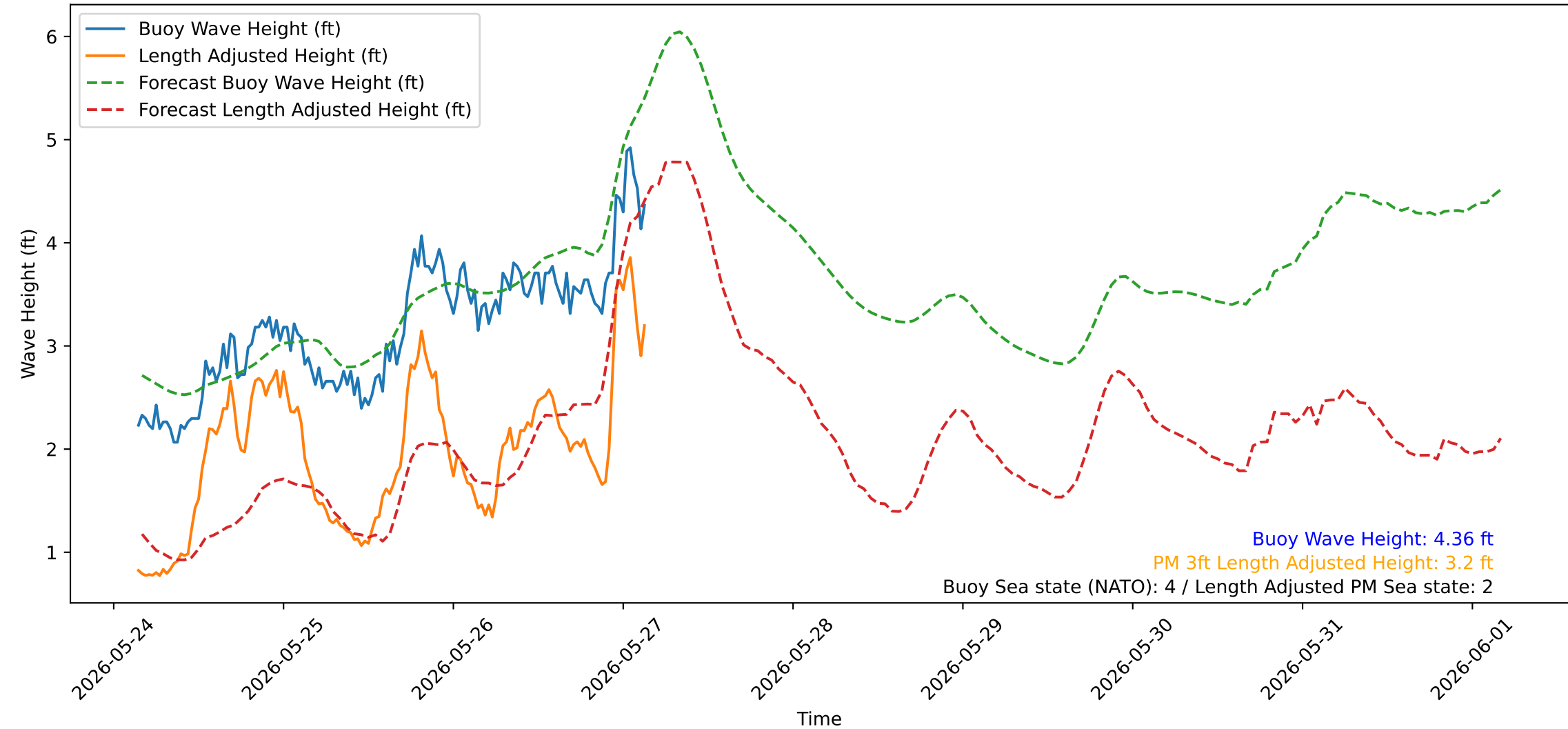
Wave Heights over Time for Green Beach at 2026-05-27 03:41:09
