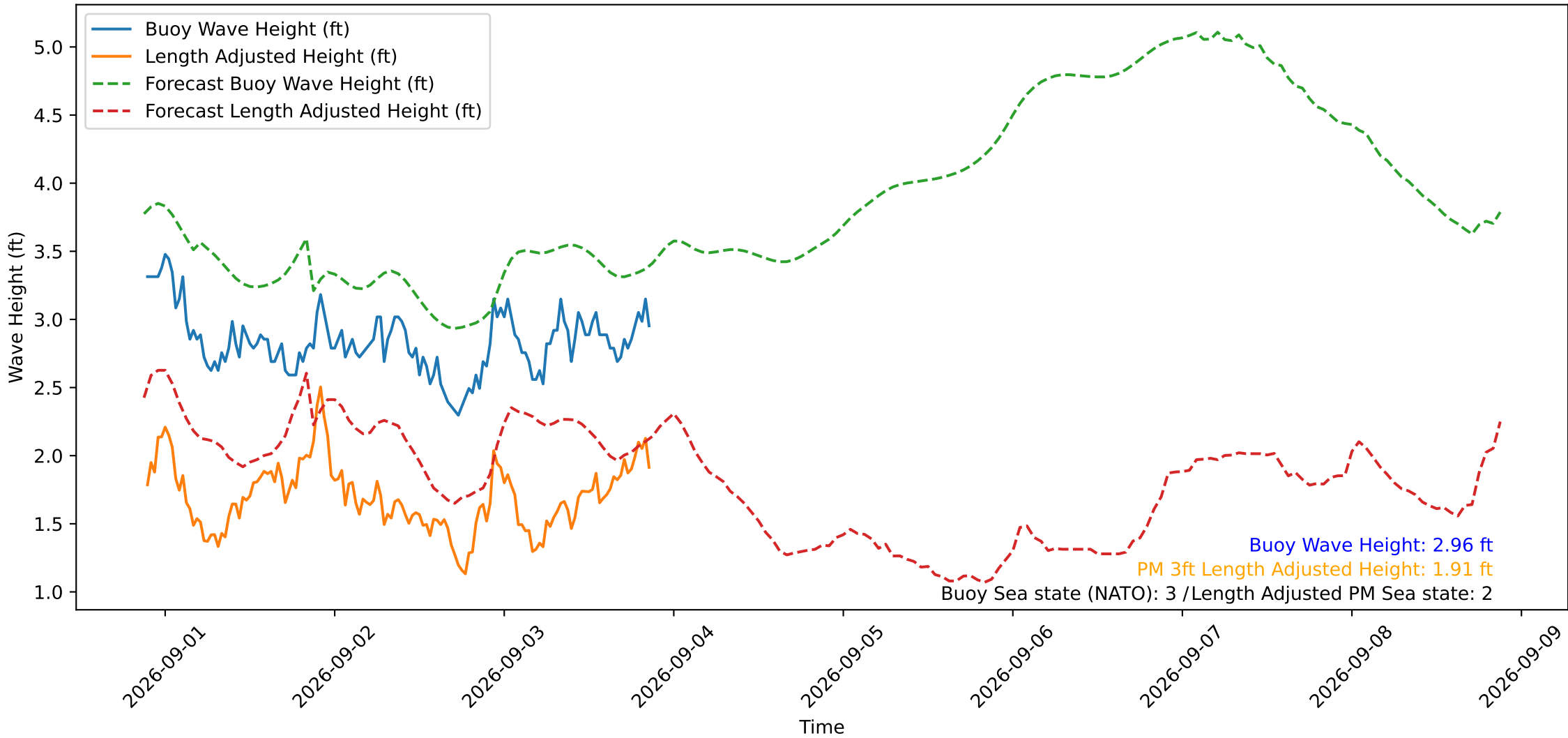
Wave Heights over Time for Red Beach at 2026-09-03 21:20:50
