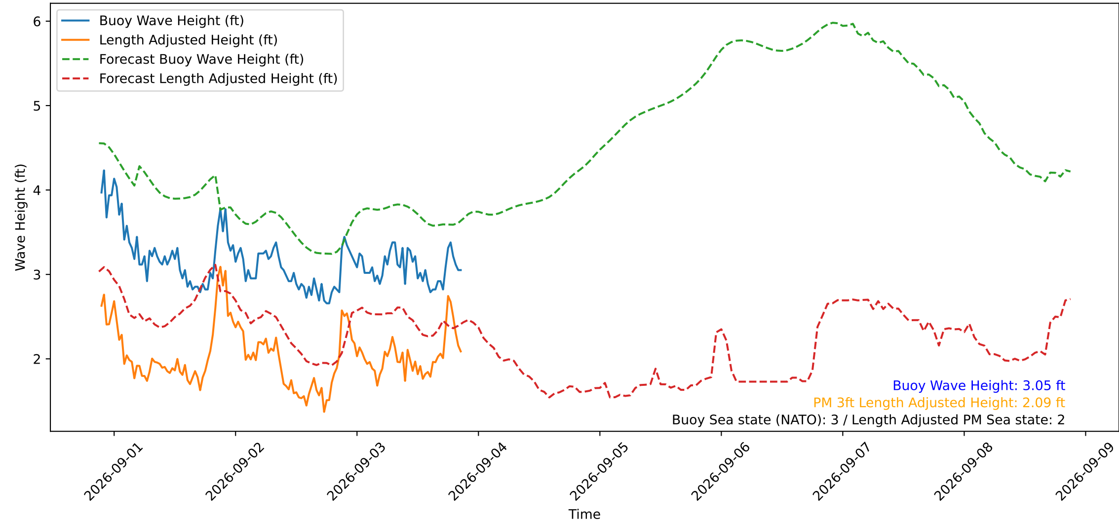
Wave Heights over Time for Green Beach at 2026-09-03 21:21:14
