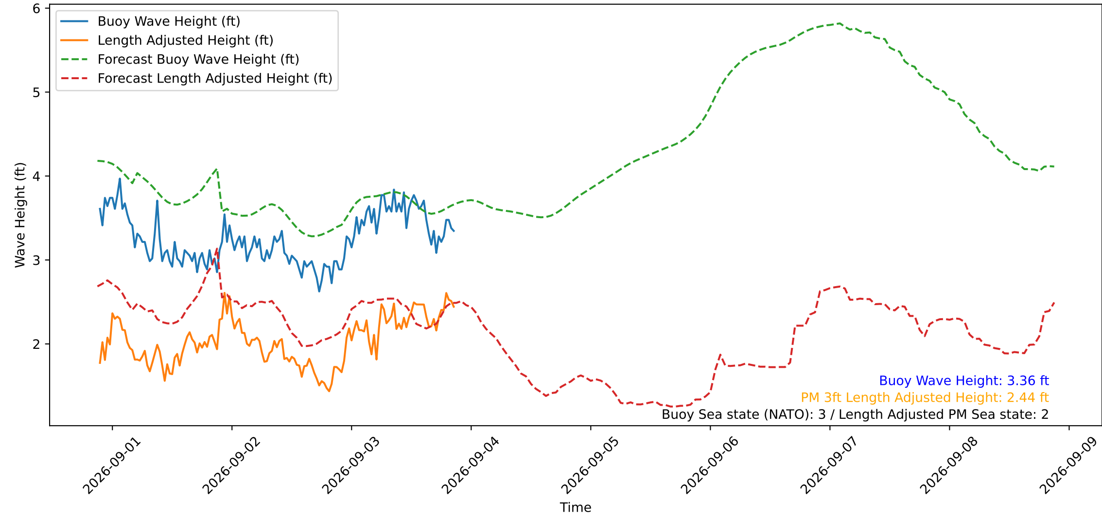
Wave Heights over Time for Oceanside Harbor at 2026-09-03 21:20:29
