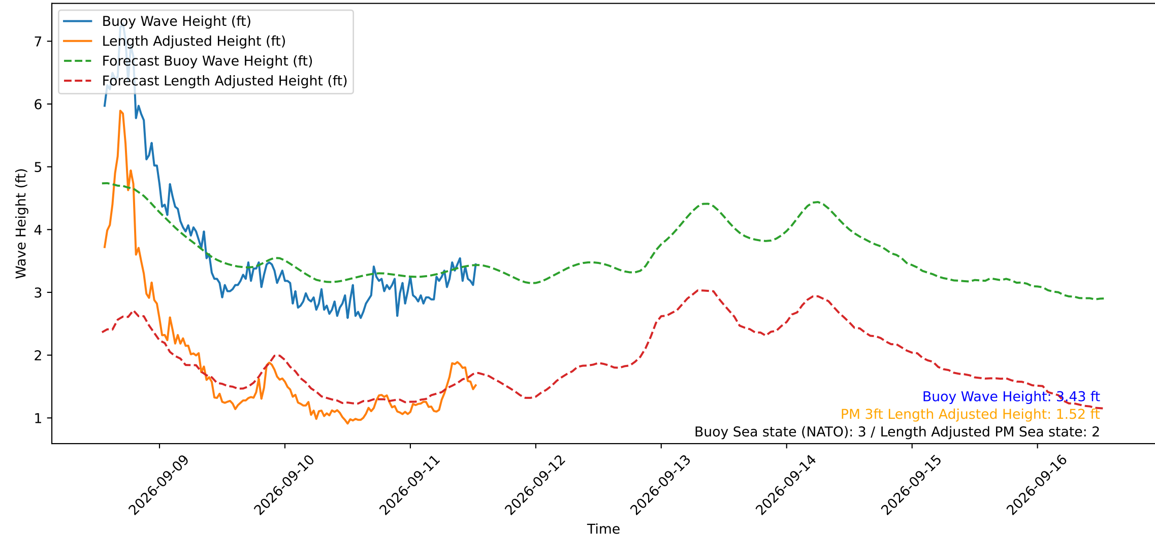
Wave Heights over Time for Green Beach at 2026-09-11 13:11:13
