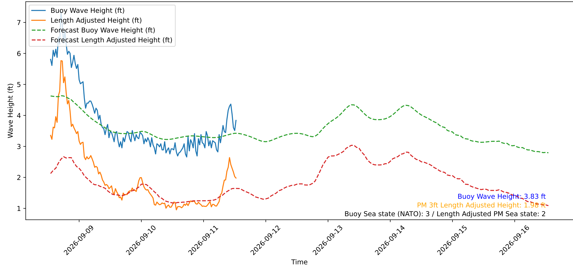
Wave Heights over Time for Oceanside Harbor at 2026-09-11 13:10:30
