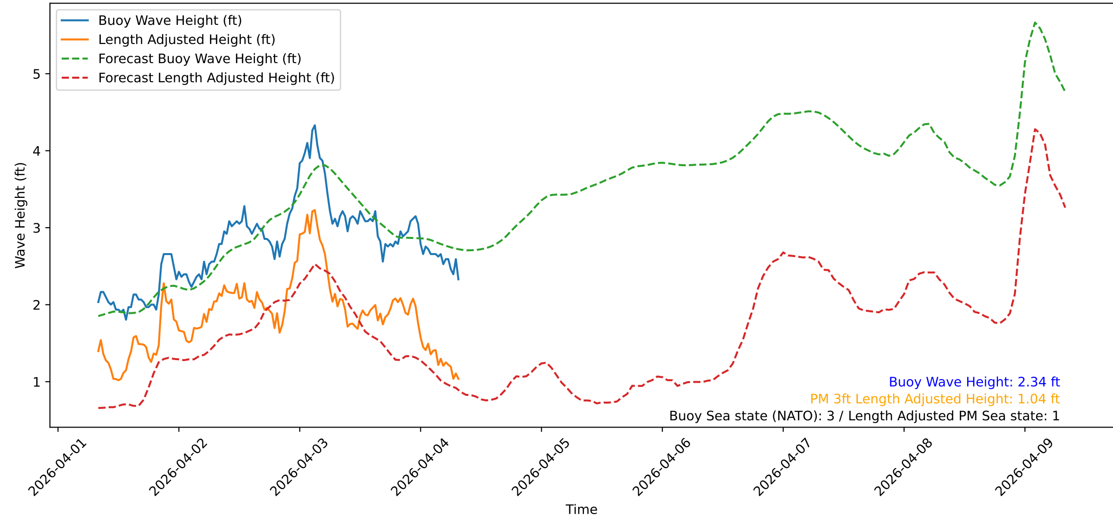
Wave Heights over Time for Green Beach at 2026-04-04 08:11:13
