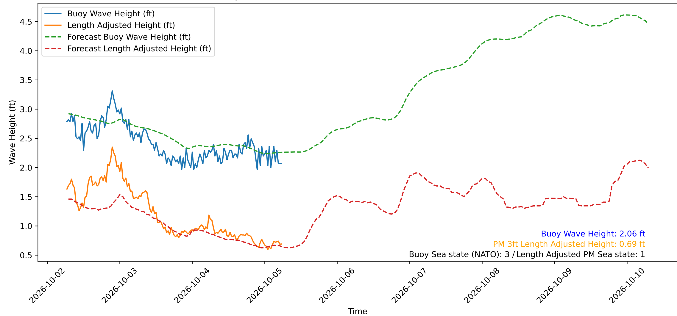
Wave Heights over Time for Oceanside Harbor at 2026-10-05 06:30:30
