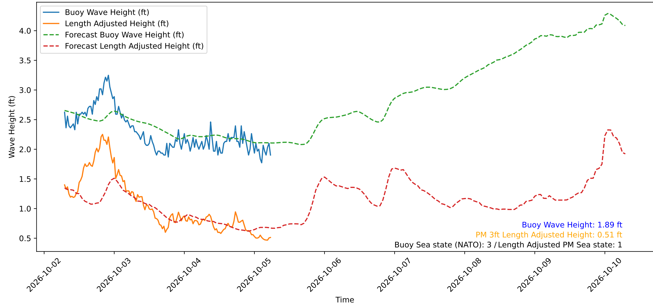
Wave Heights over Time for Red Beach at 2026-10-05 06:30:49
