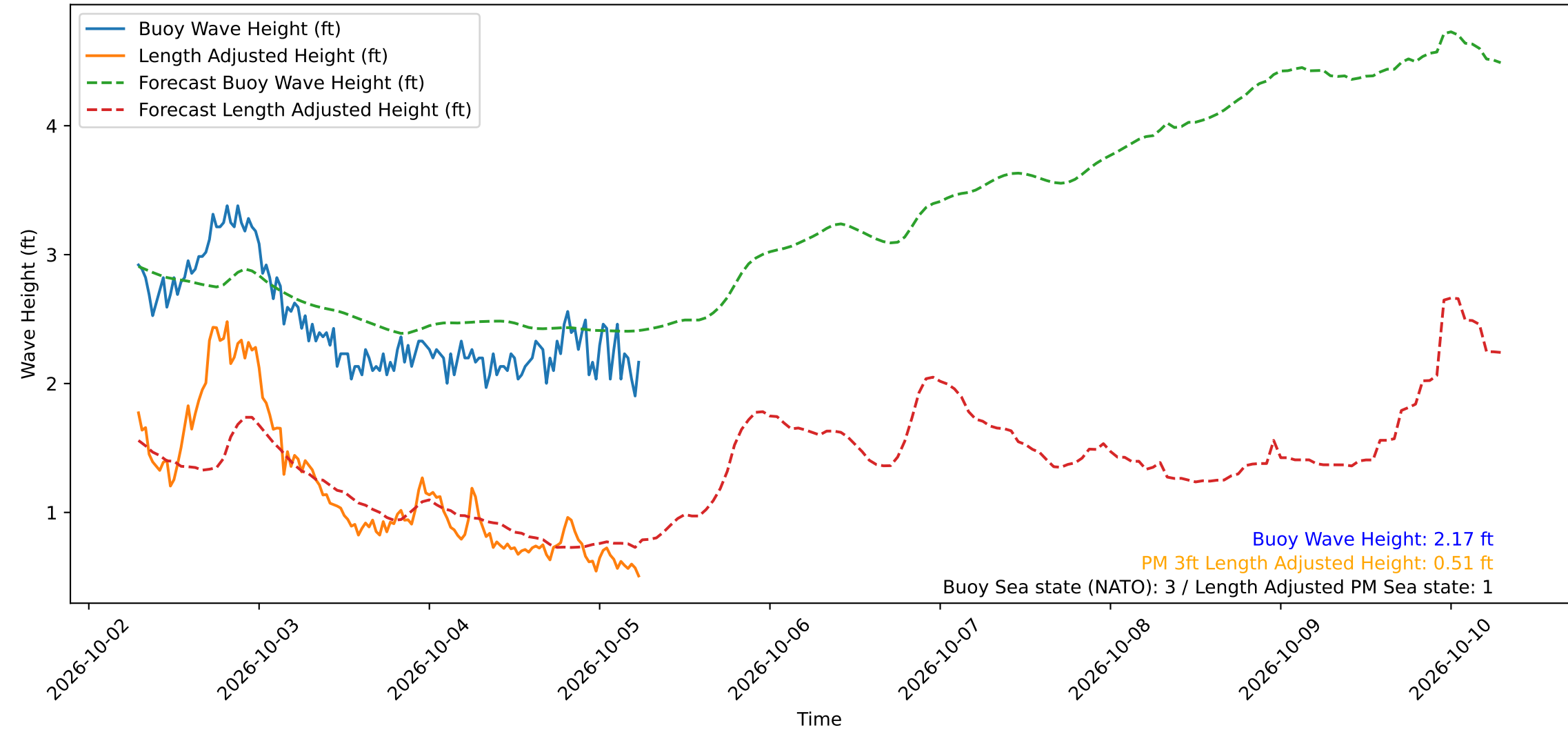
Wave Heights over Time for Green Beach at 2026-10-05 06:31:11
