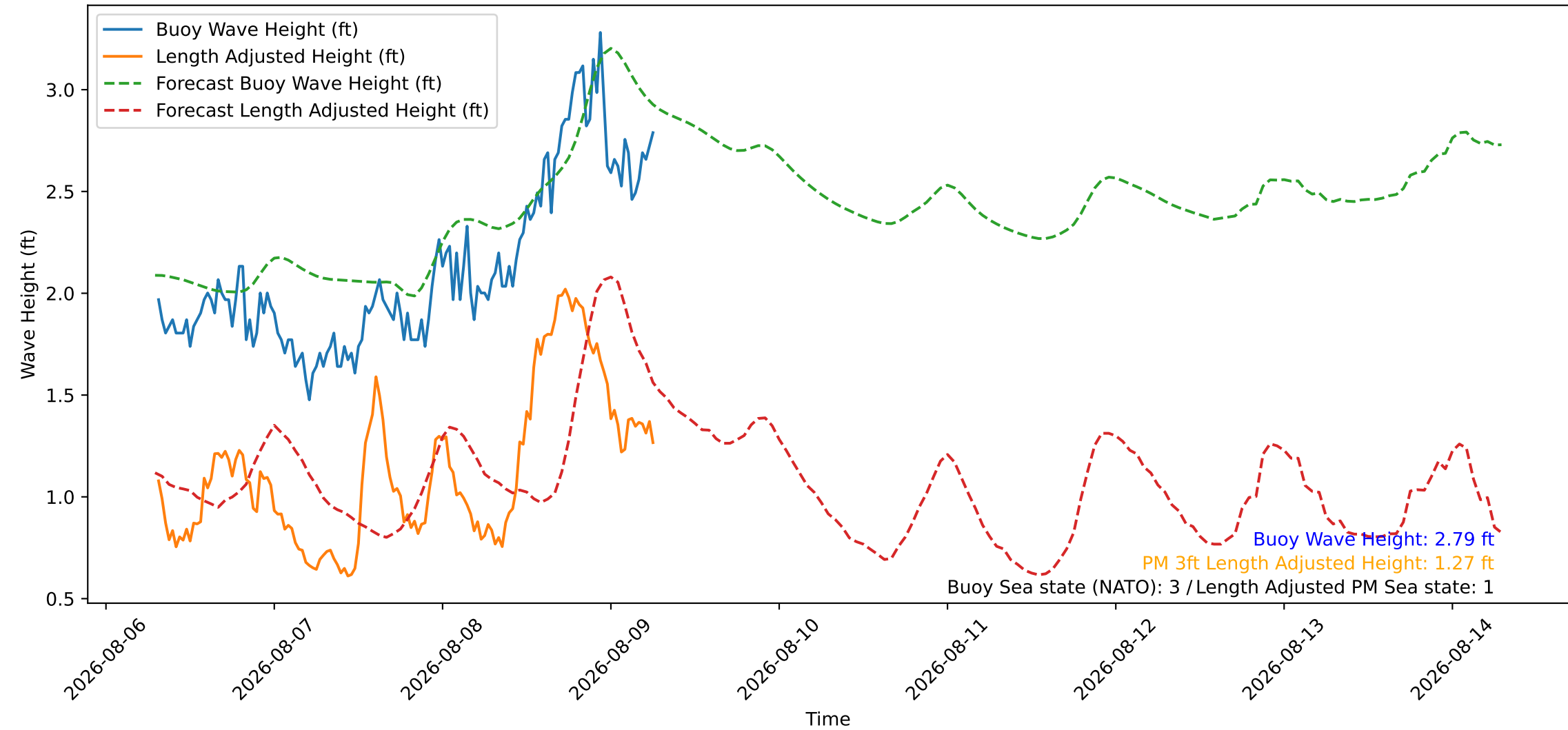
Wave Heights over Time for Red Beach at 2026-08-09 07:00:46
