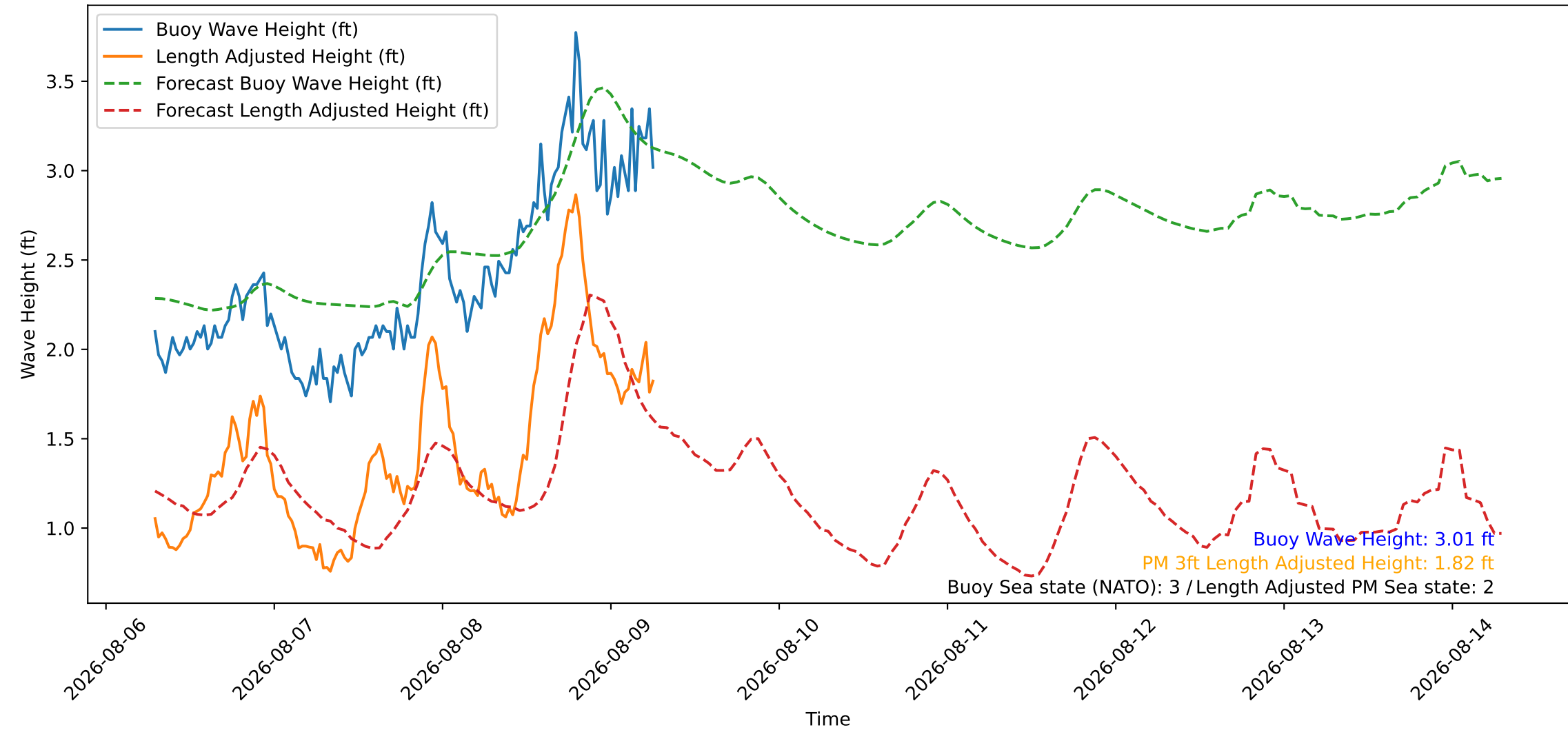
Wave Heights over Time for Green Beach at 2026-08-09 07:01:09
