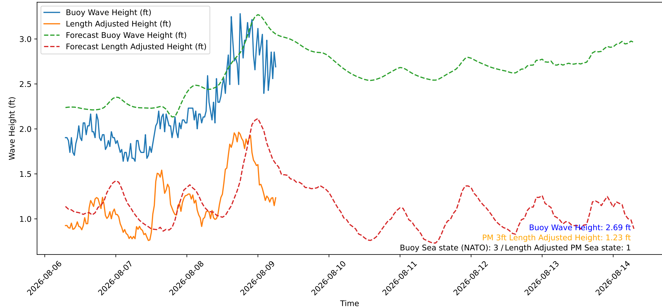
Wave Heights over Time for Oceanside Harbor at 2026-08-09 07:00:27
