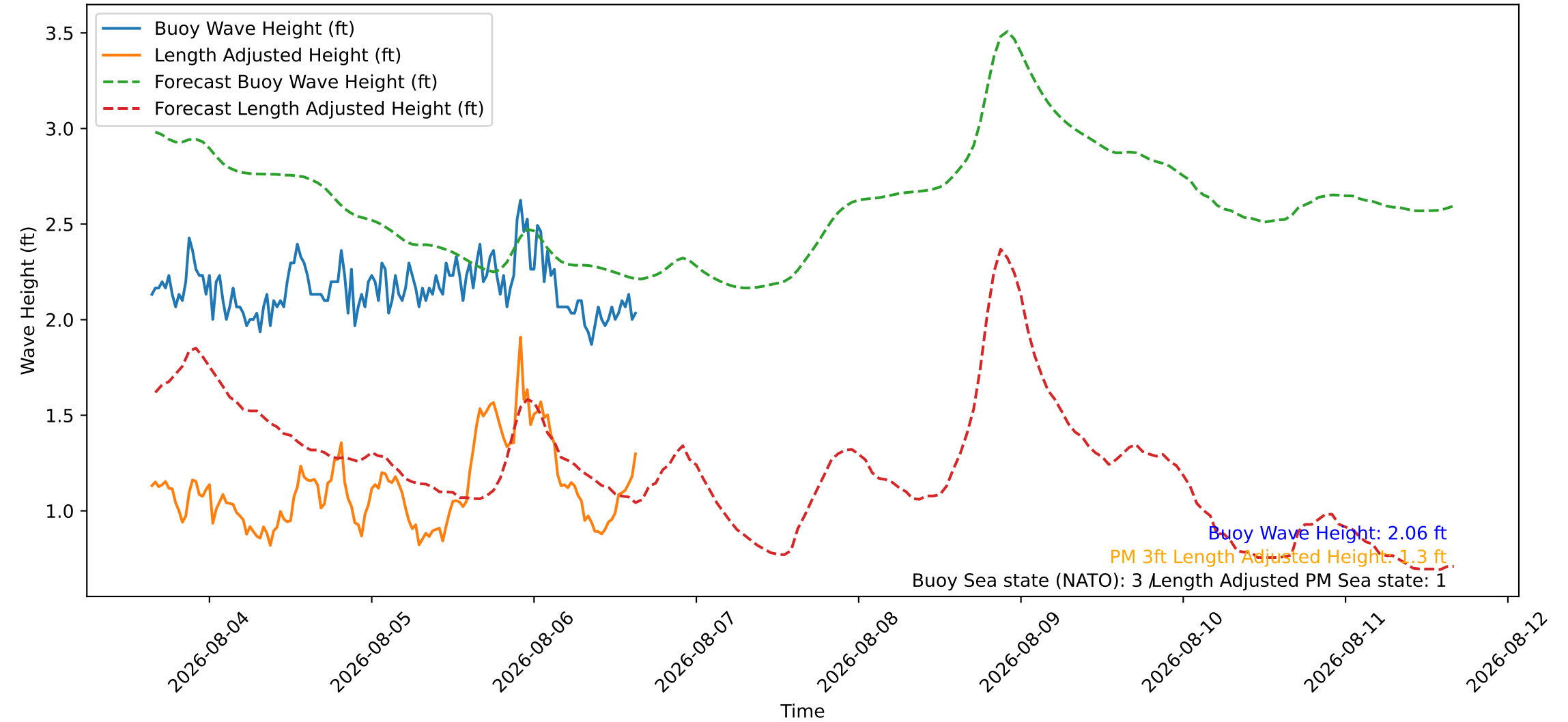
Wave Heights over Time for Green Beach at 2026-08-06 15:41:08
